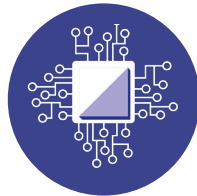
Intelligent Algorithm
