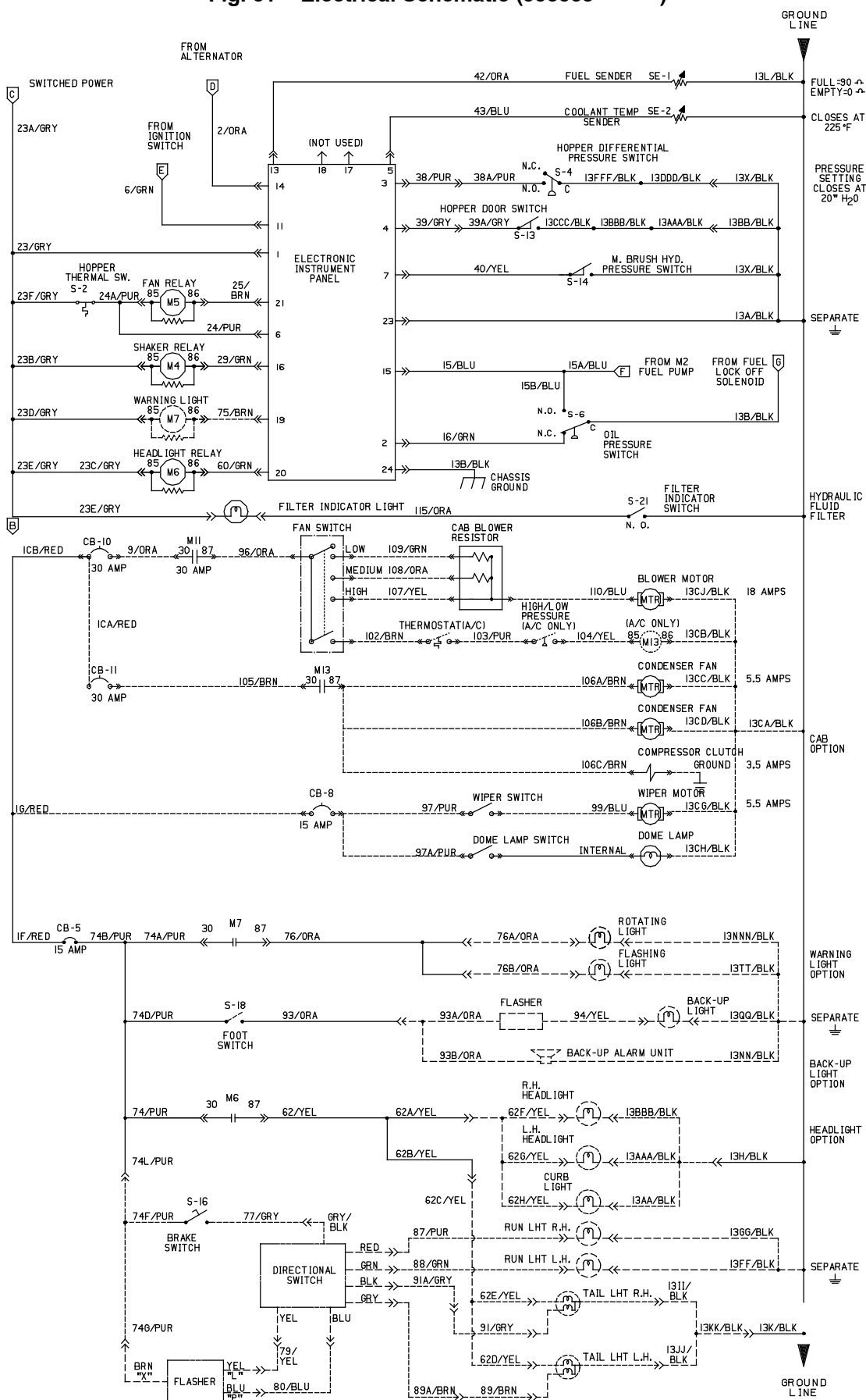
Fig. 61 - Electrical Schematic (006009- )
