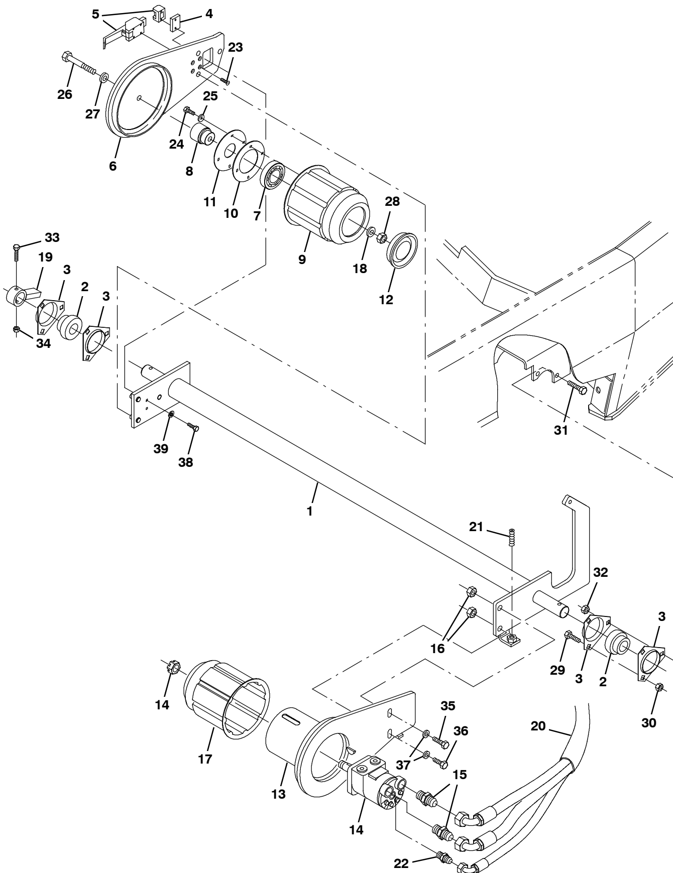
Fig. 51 - Brush Drive Group, Main
