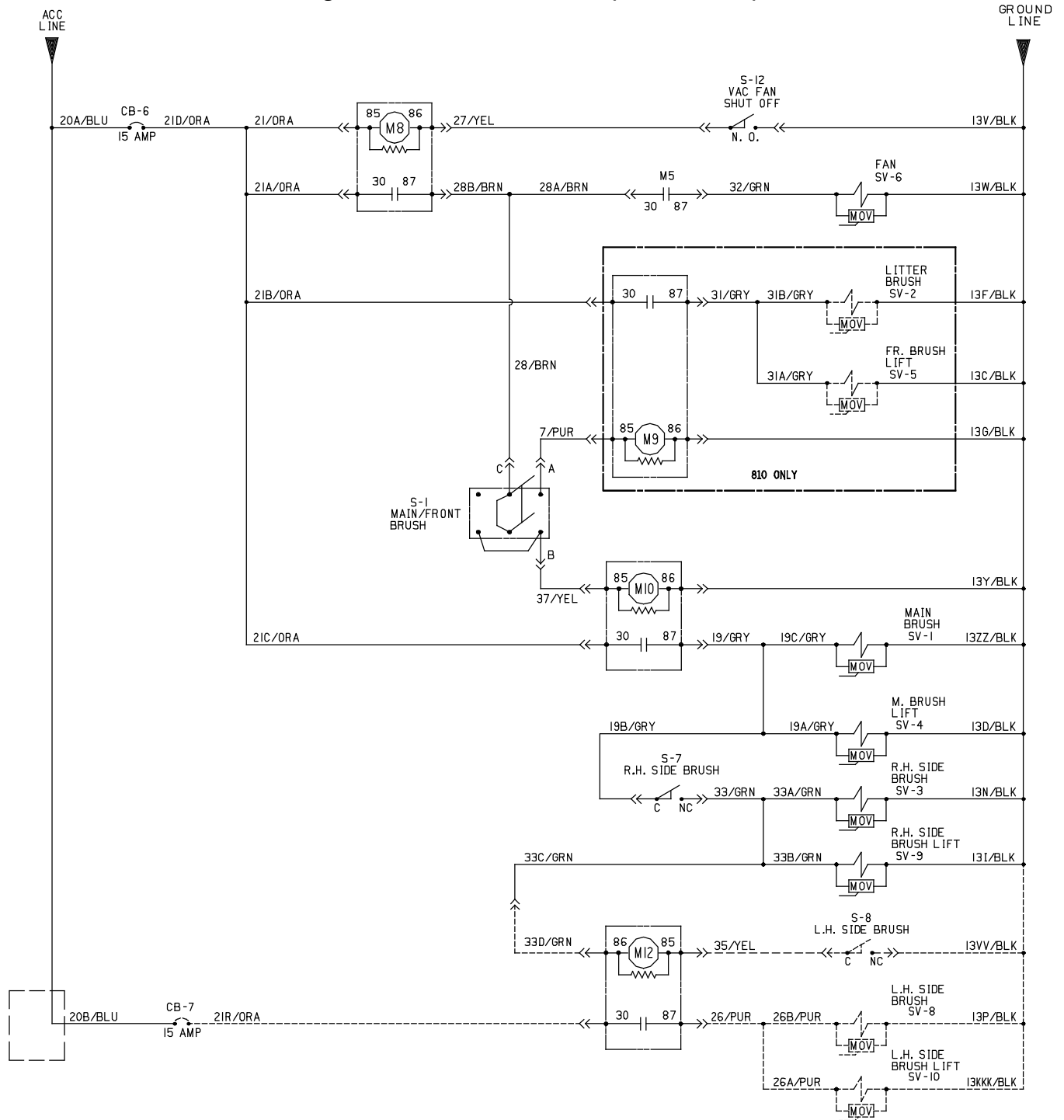
Fig. 61 - Electrical Schematic (006009- )
