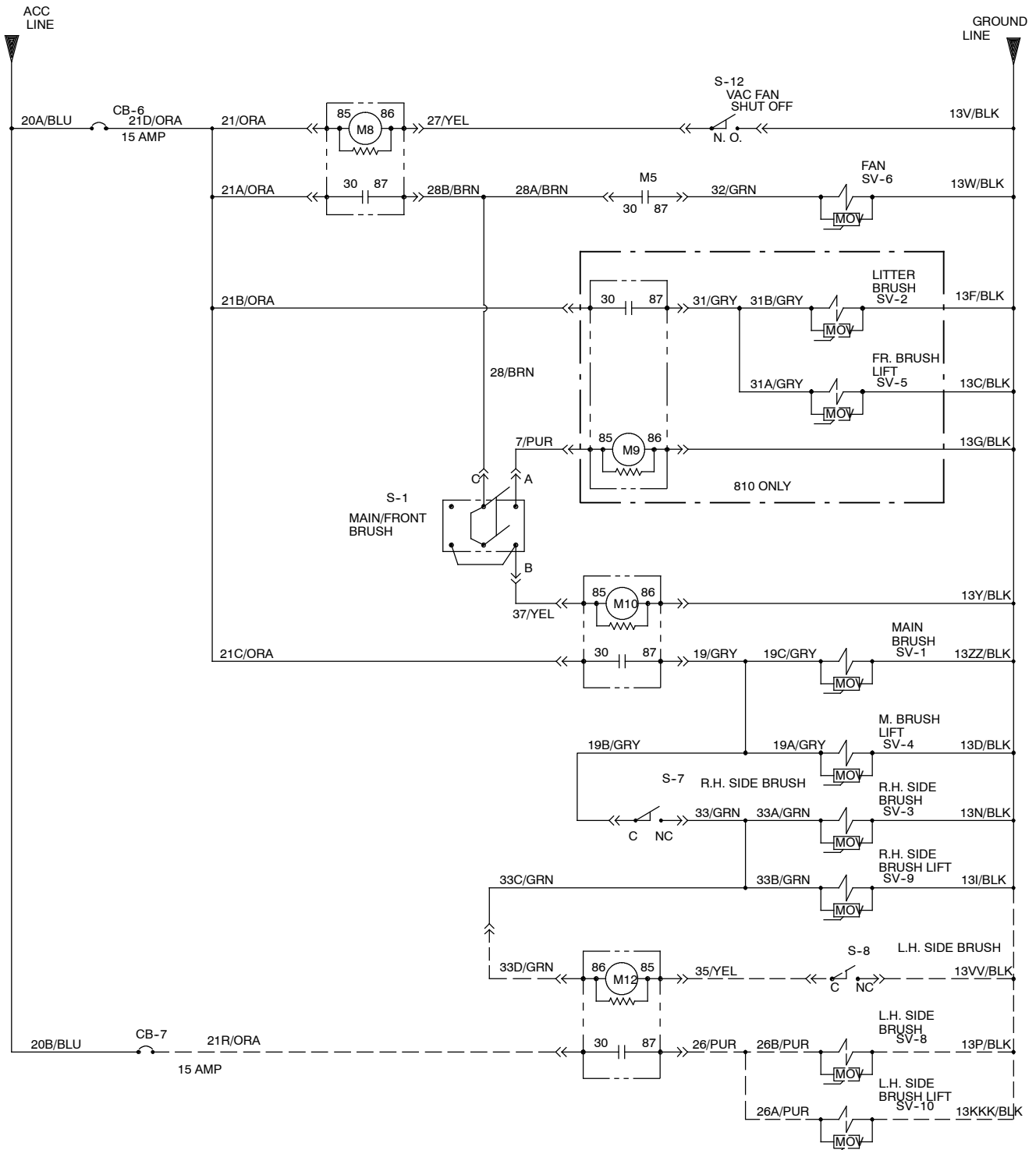
Fig. 59 - Electrical Schematic (004000- 004302)
