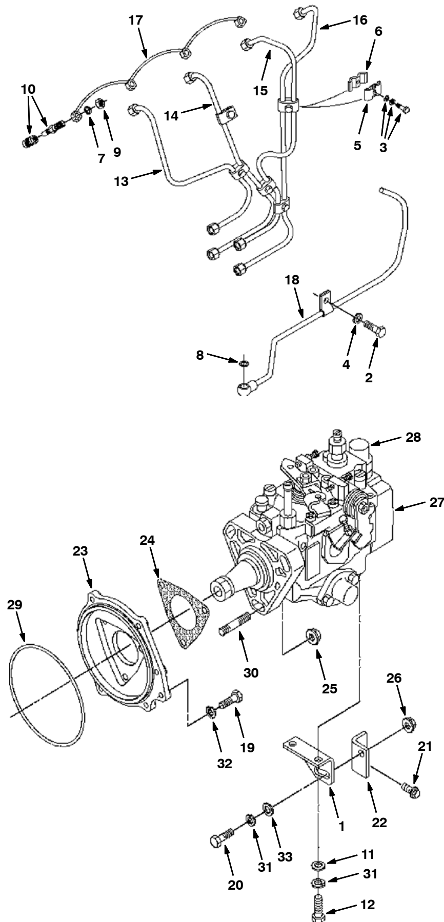
Fig. 13 - Fuel Group
