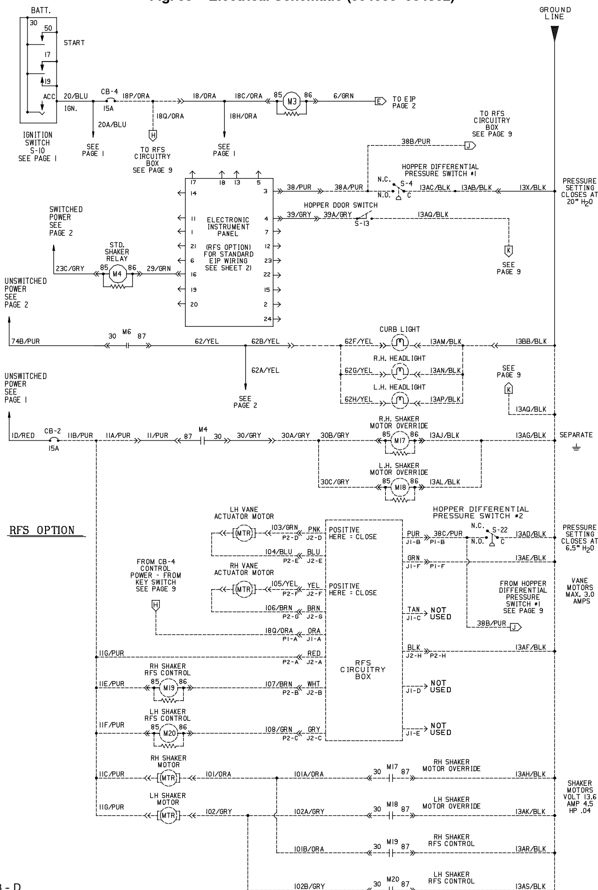
Fig. 59 - Electrical Schematic (004000-004302)
