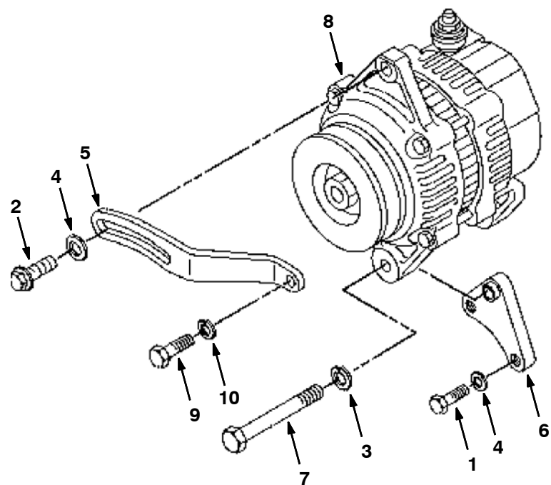
Fig. 15 - Alternator Group
