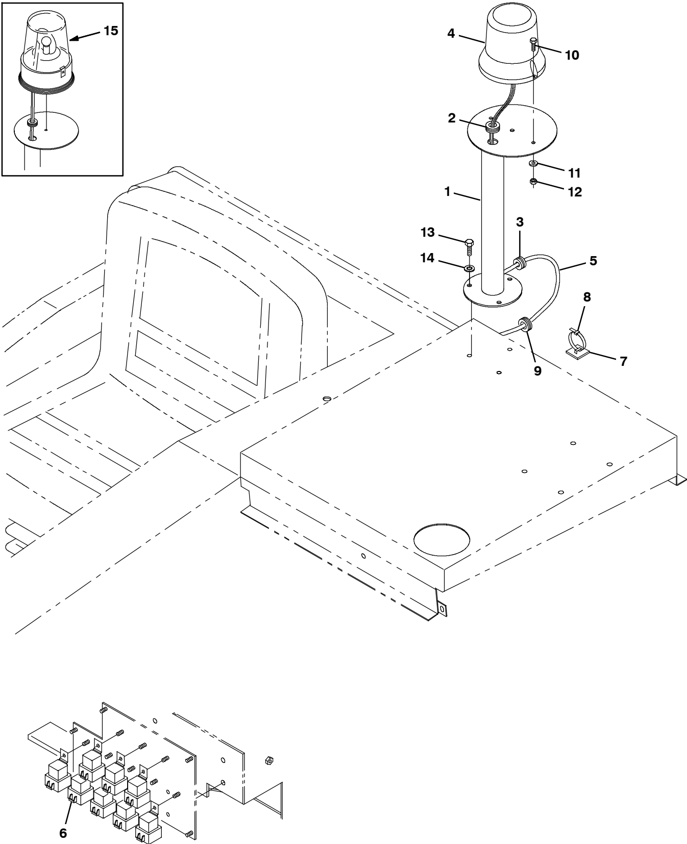
Fig. 6 - Light Kit, Strobe, Low
