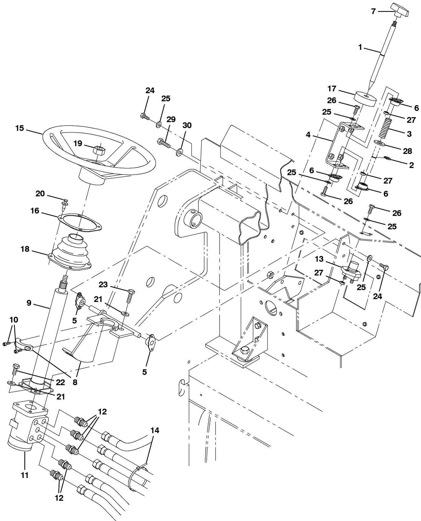
Fig. 56 - Steering Group
