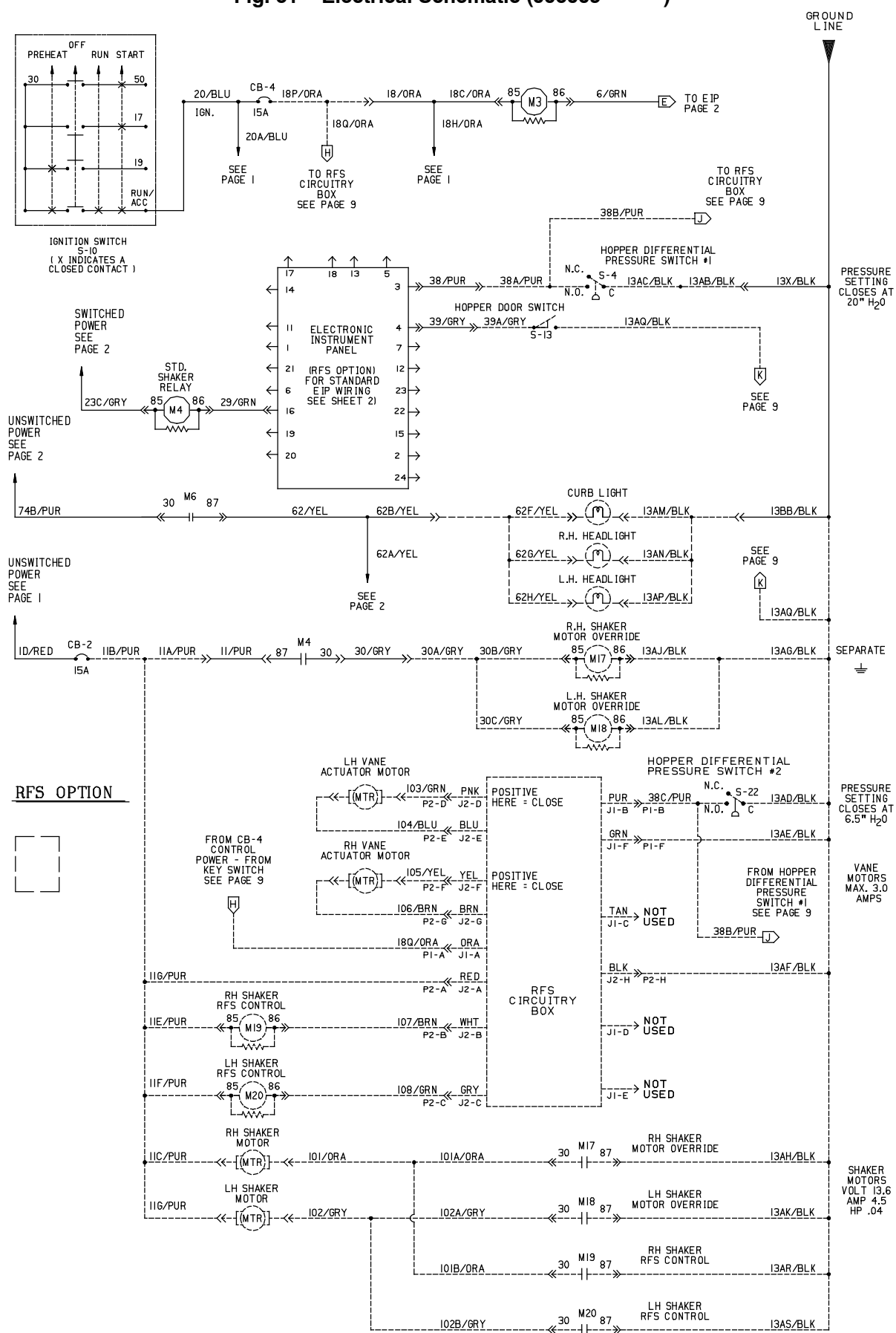
Fig. 61 - Electrical Schematic (006009- )
