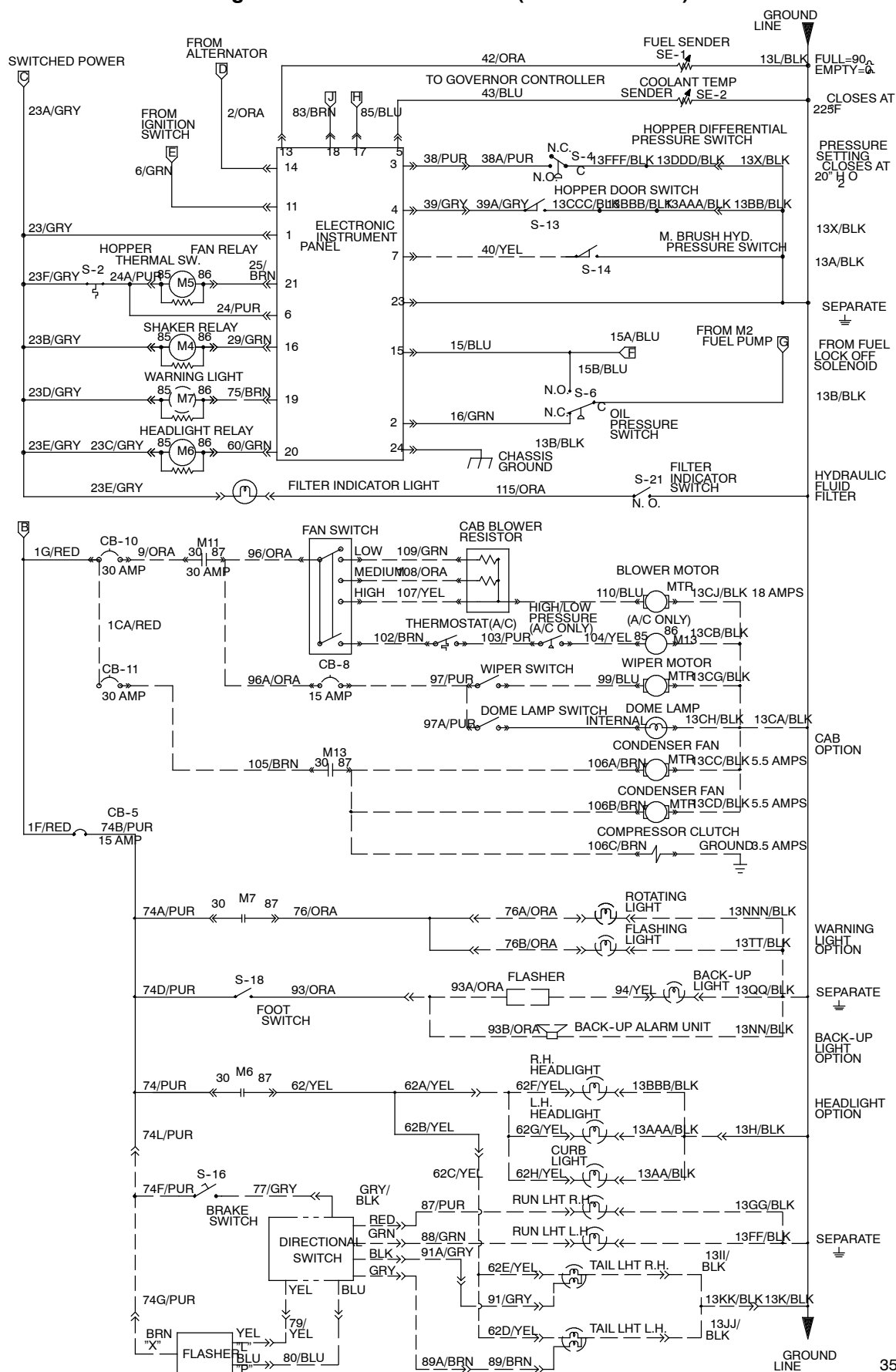
Fig. 59 - Electrical Schematic (004000- 004302)
