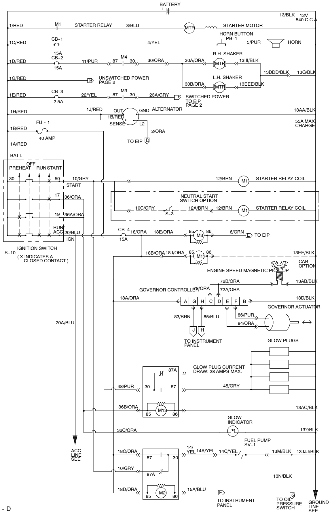
Fig. 59 - Electrical Schematic (004000- 004302)
