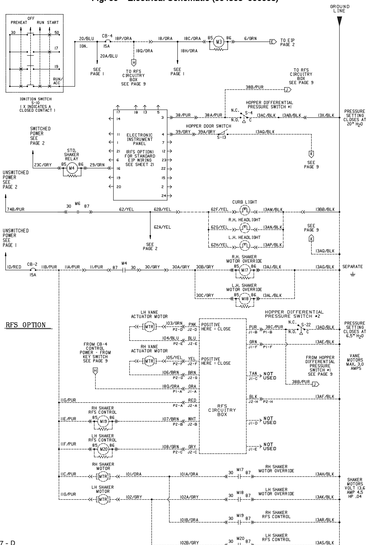
Fig. 60 - Electrical Schematic (004303-006008)
