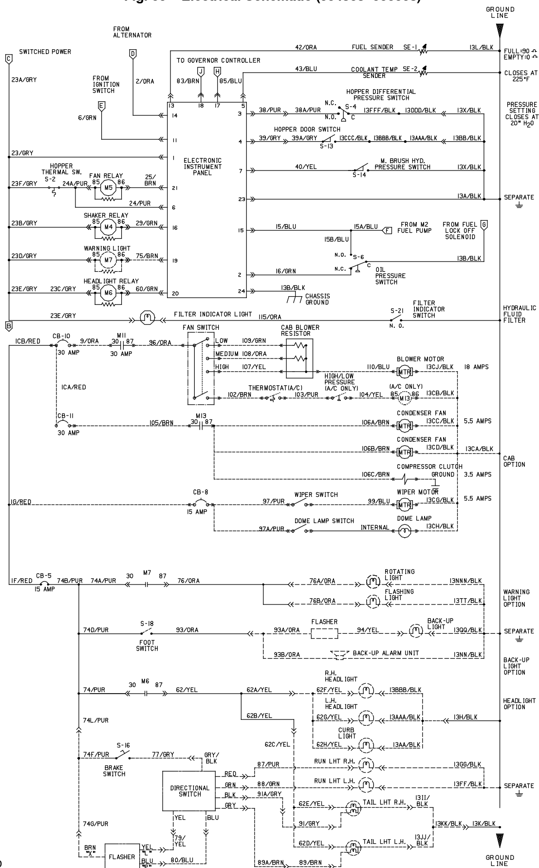
Fig. 60 - Electrical Schematic (004303-006008)
