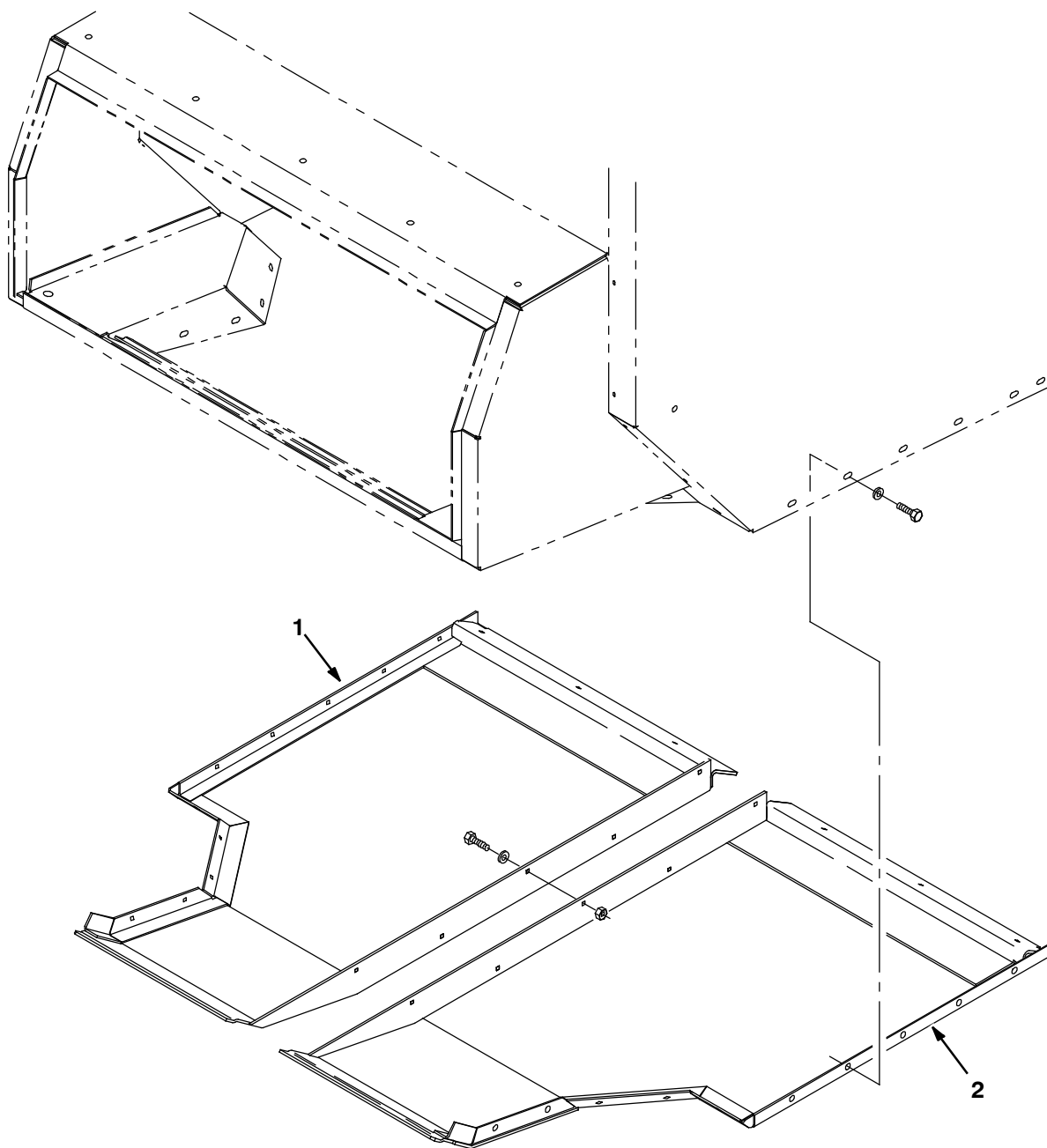
Fig. 10 - Hopper Floor Kit
