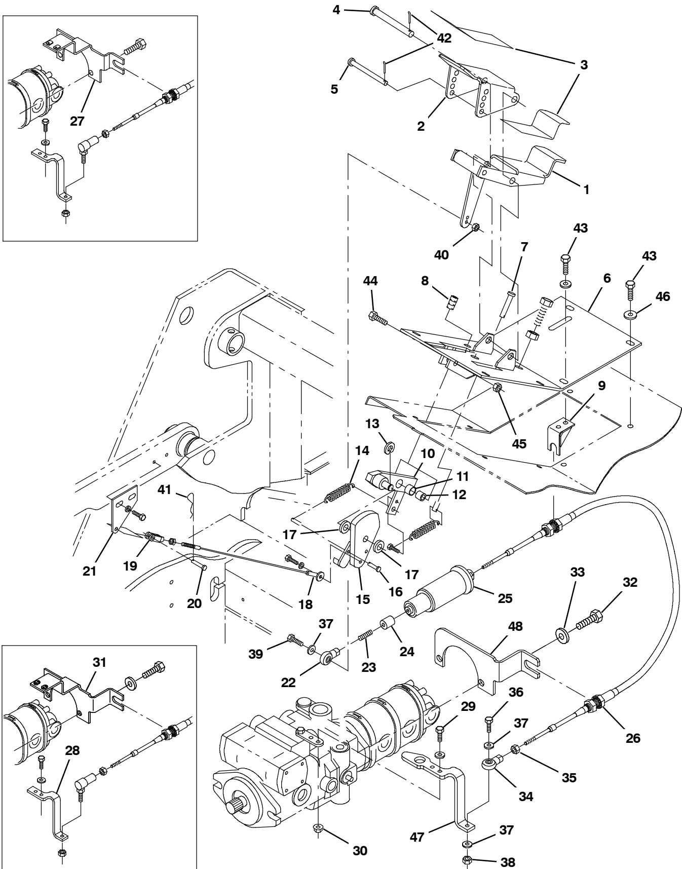
Fig. 41 - Directional Pedal Group
