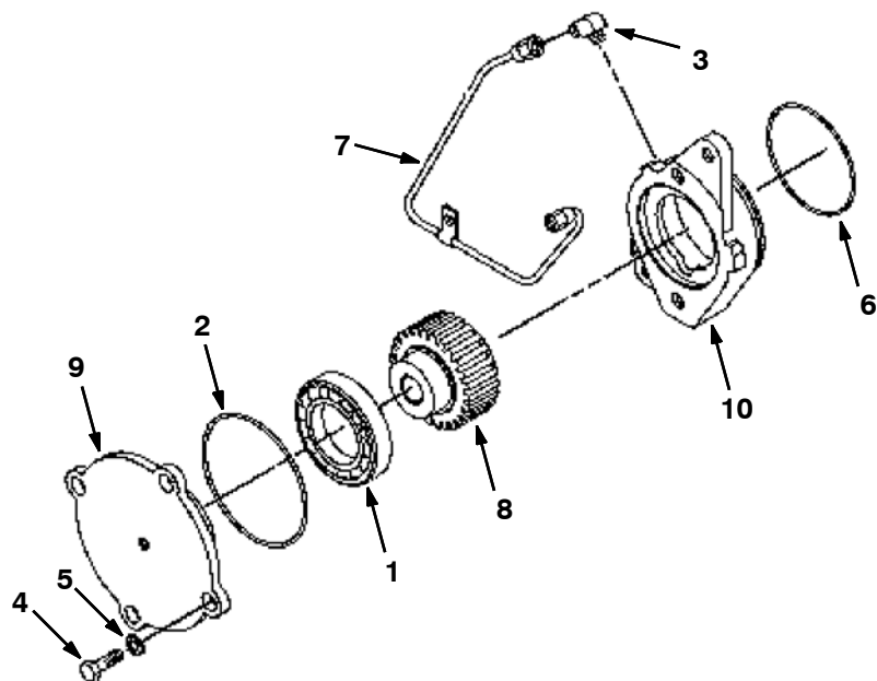
Fig. 8 - Auxiliary Drive Group
