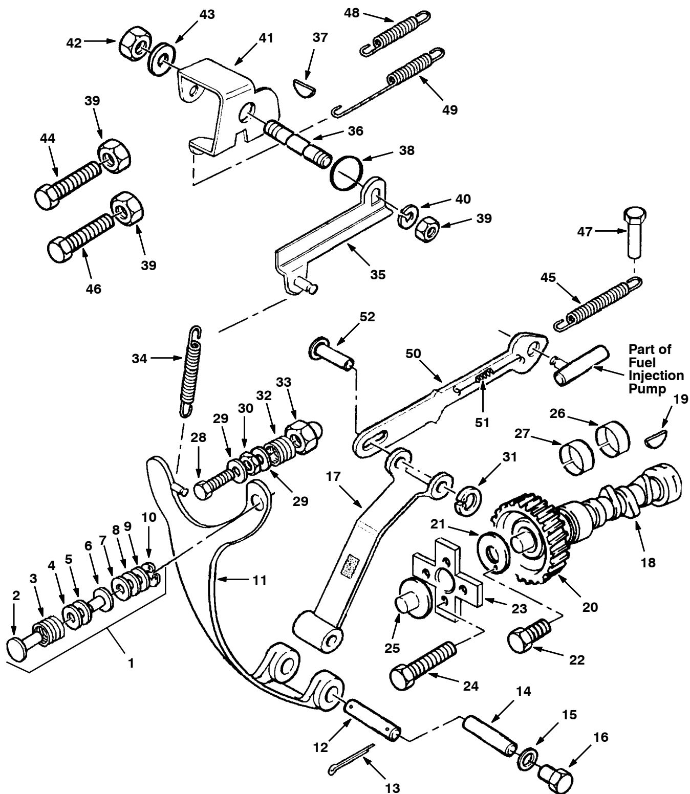
Fig. 7 - Auxiliary Drive Group
