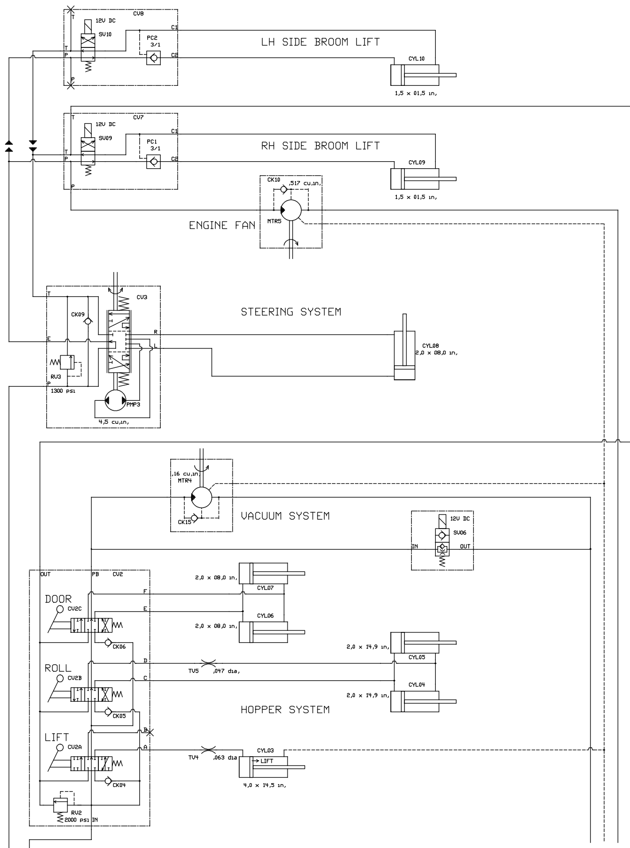
Fig. 43 - Hydraulic Schematic
