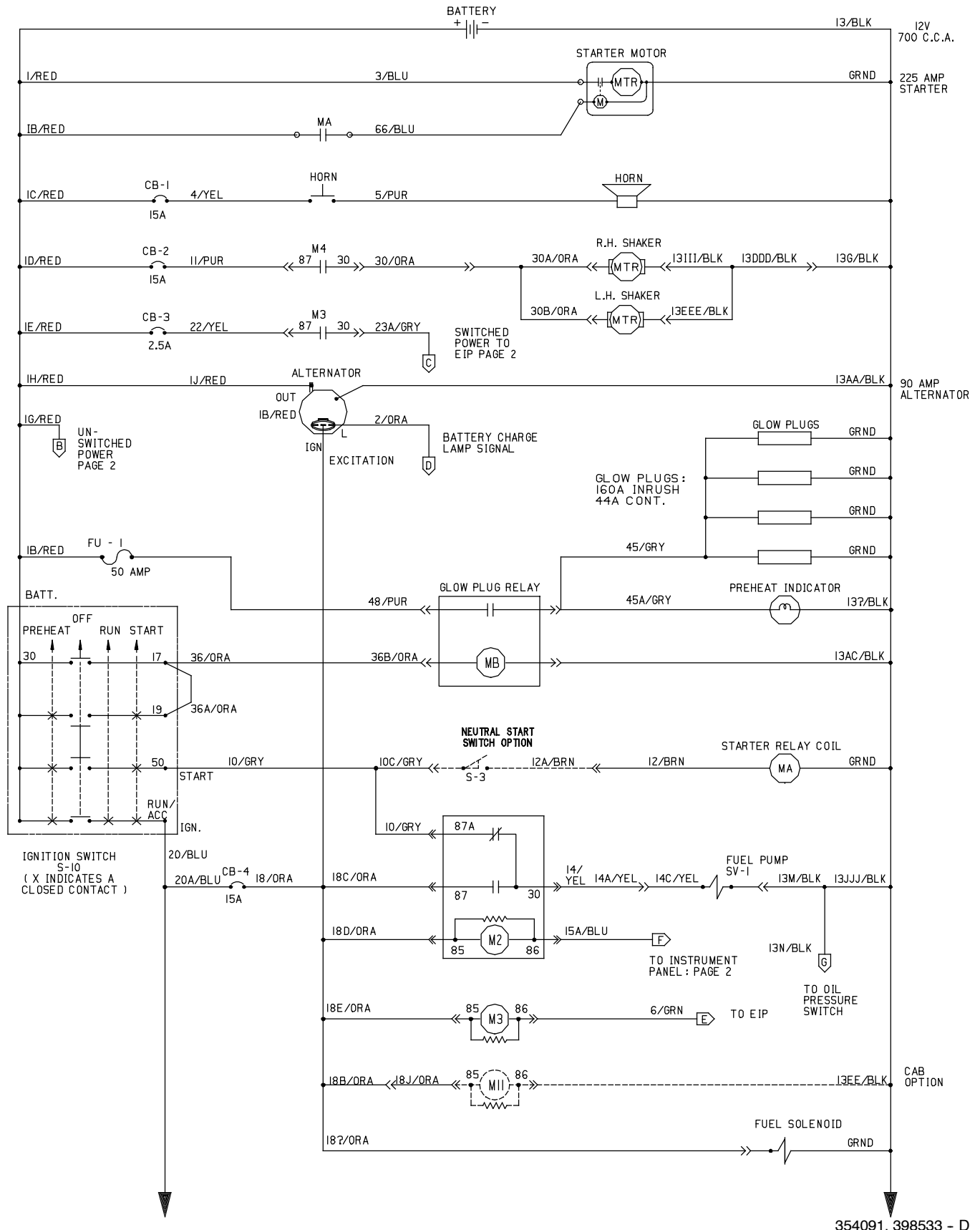
Fig. 61 - Electrical Schematic (006009- )
