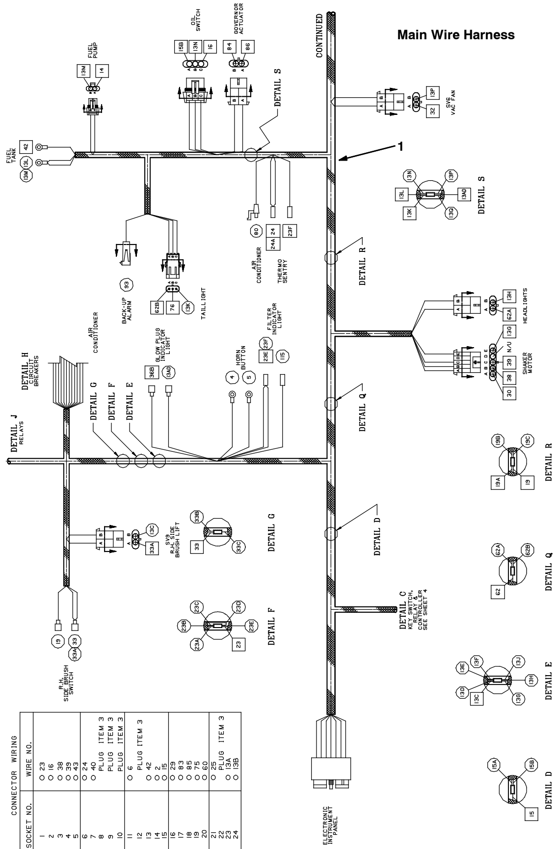
Fig. 62 - Wire Harness Group, Diesel, Main (004000- 004302)
