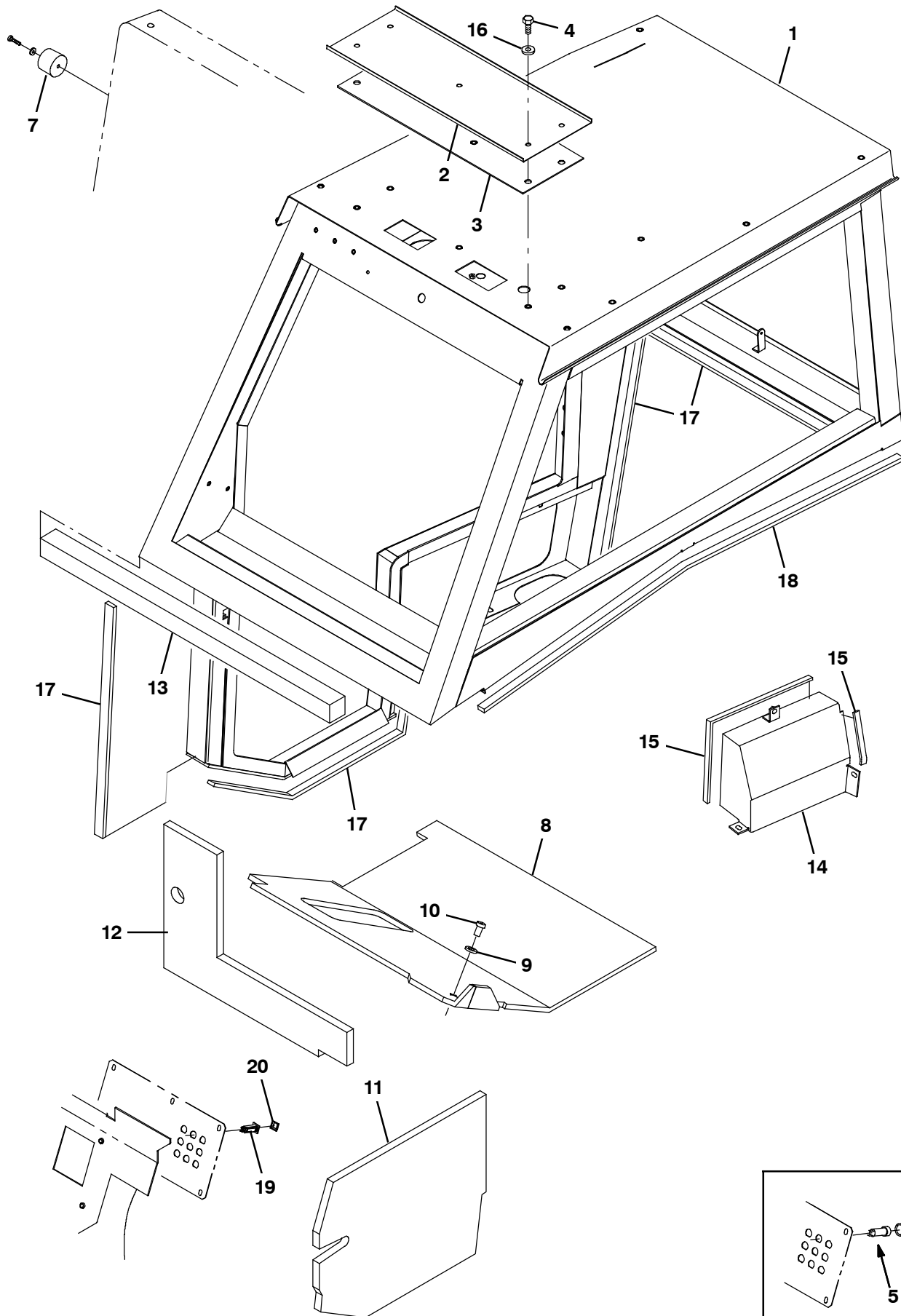
Fig. 17 - Cab Kit
