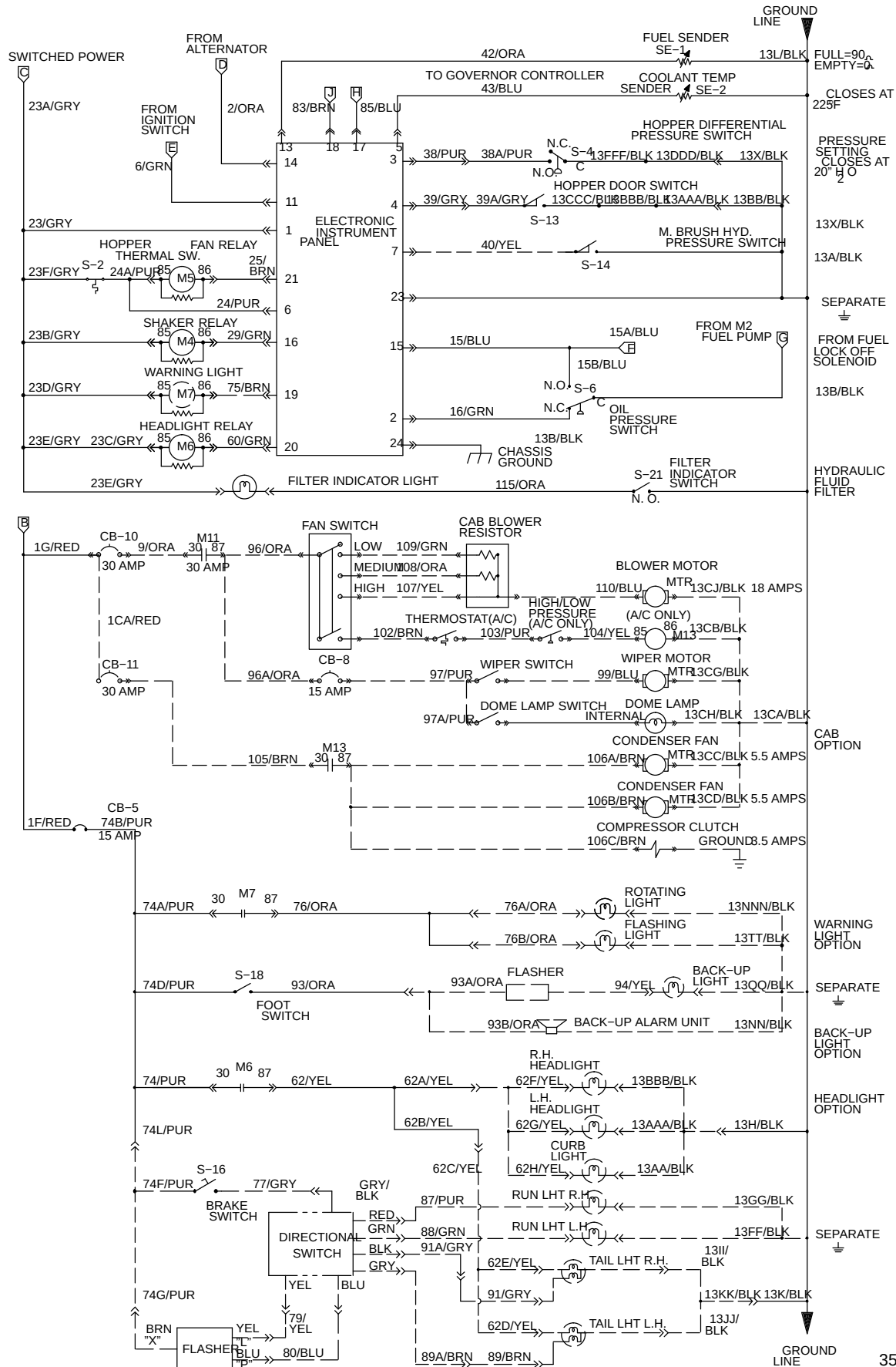
Fig. 59 – Electrical Schematic (004000– 004302)
