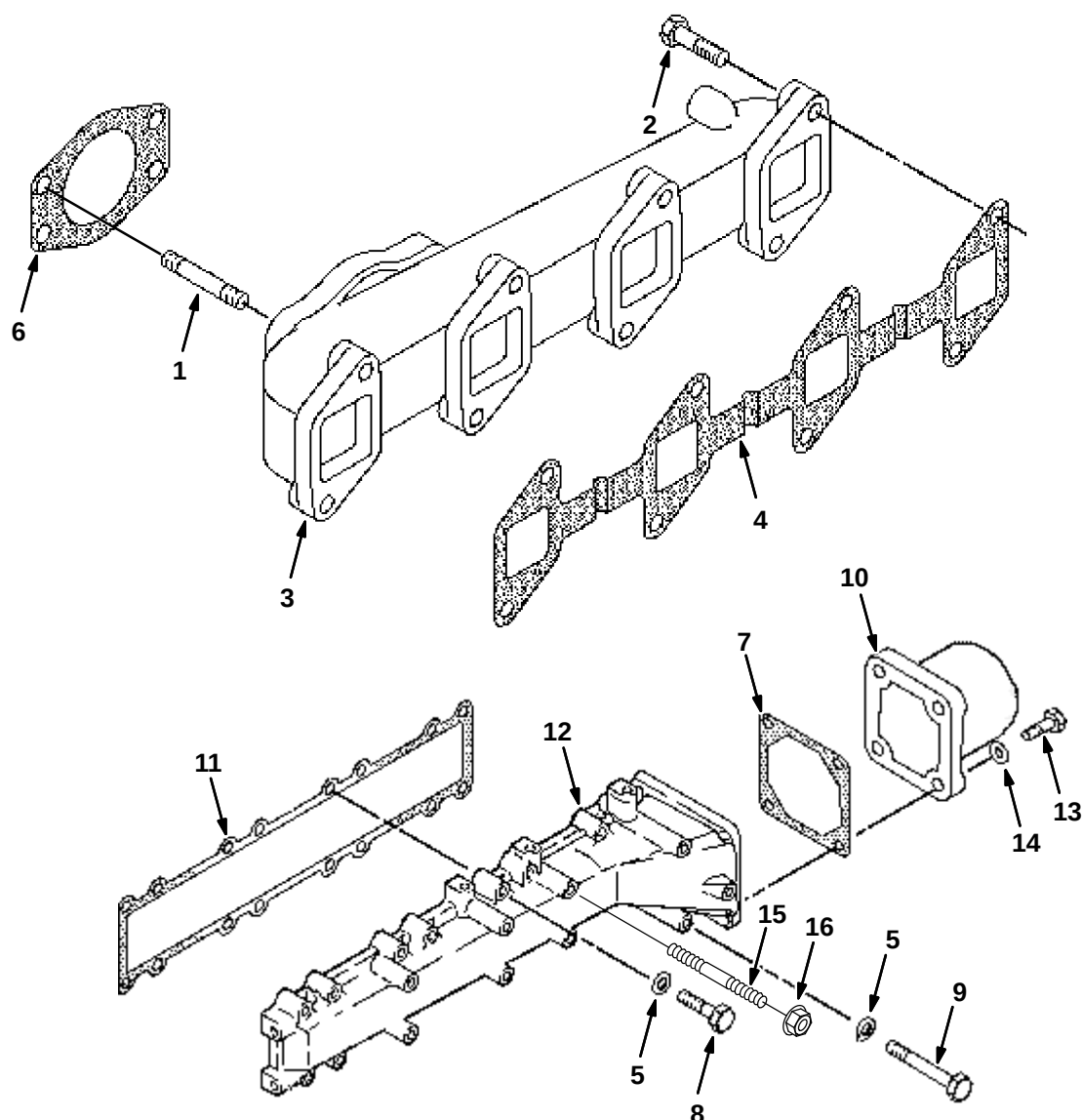
Fig. 12 – Manifold Group
