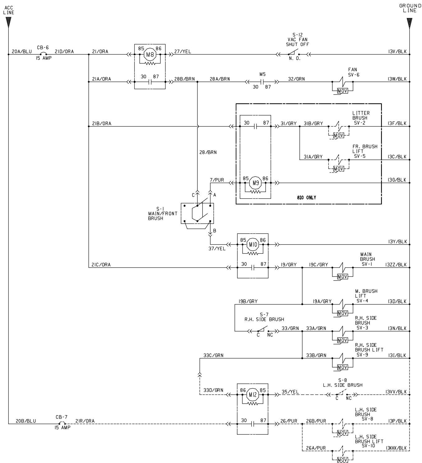
Fig. 60 – Electrical Schematic (004303-006008)
