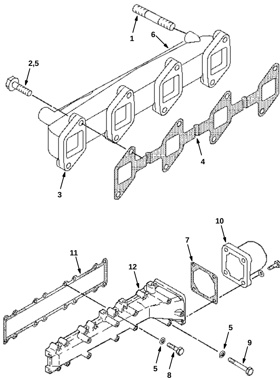
Fig. 12 – Manifold Group
