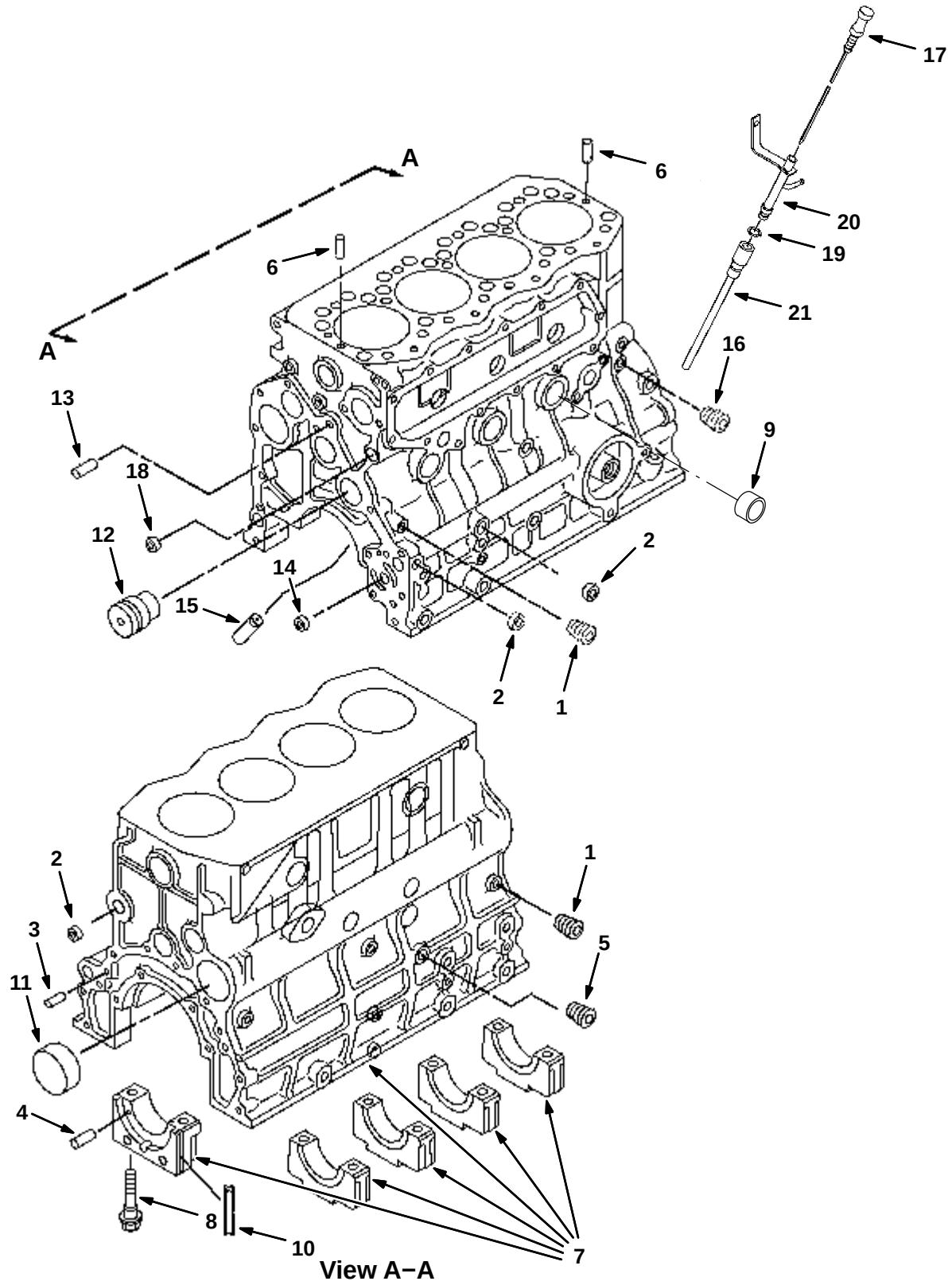
Fig. 1 – Cylinder Block Group
