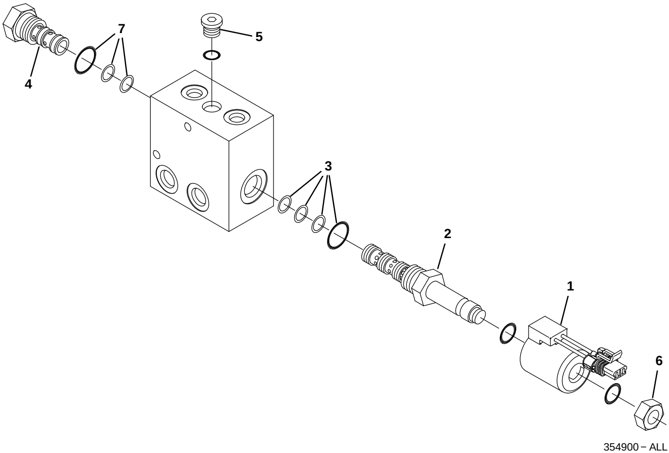
Fig. 38 – Hydraulic Solenoid Valve Breakdown, 1049211
