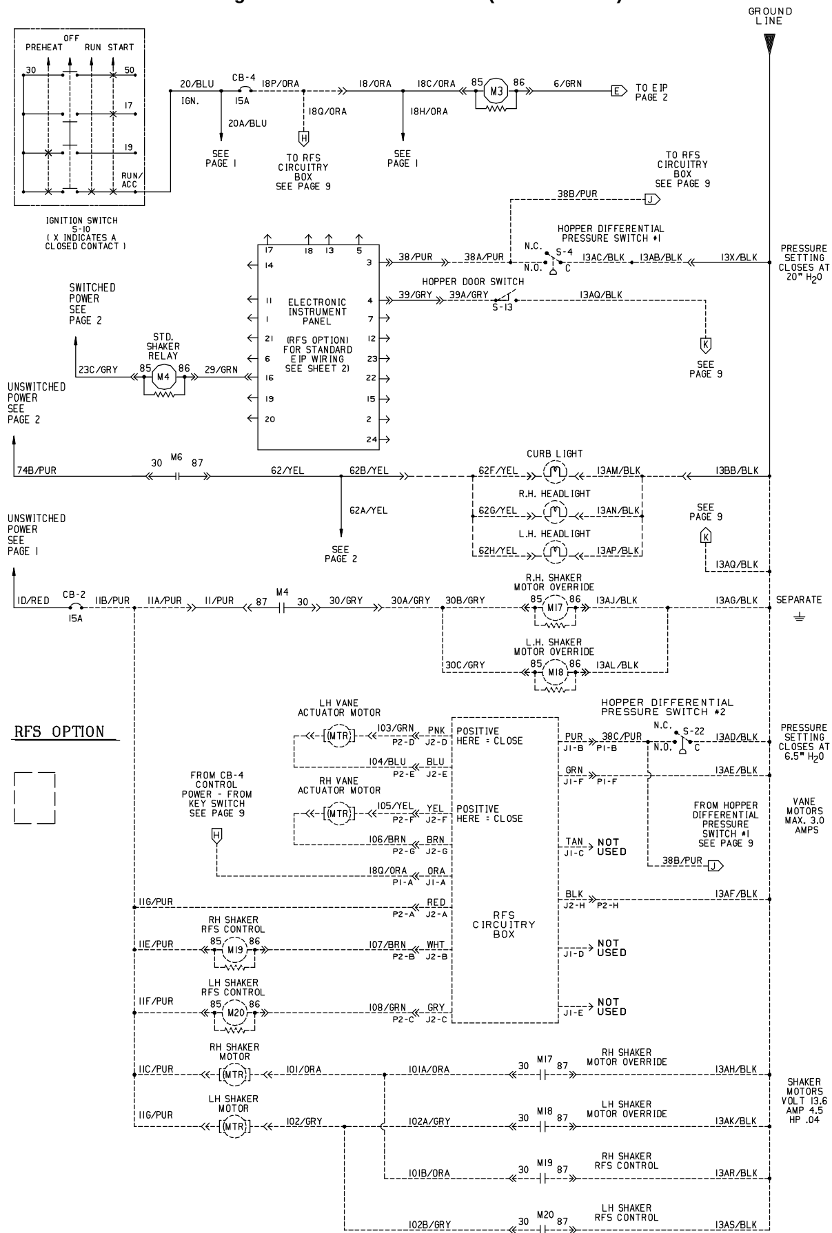
Fig. 61 – Electrical Schematic (006009– )
