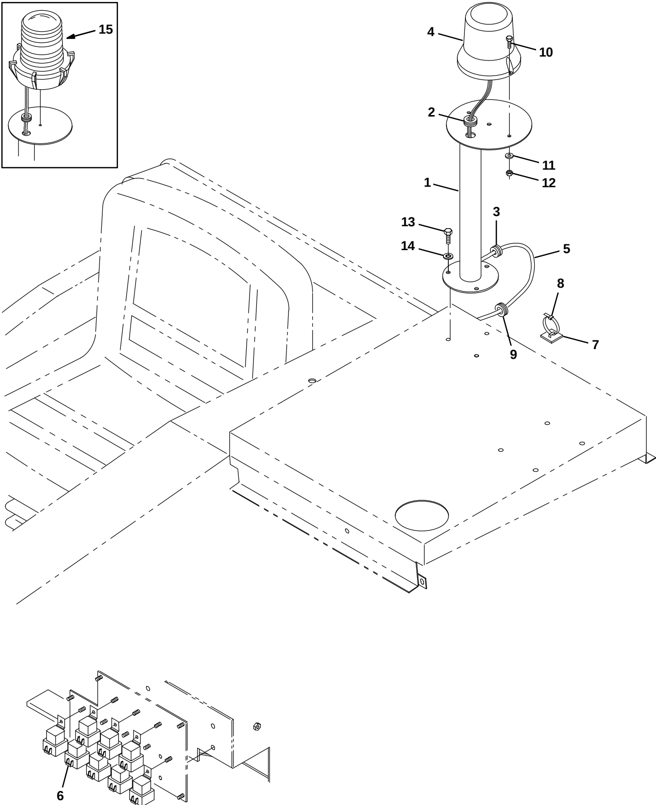
Fig. 5 – Light Kit, Flashing Low
