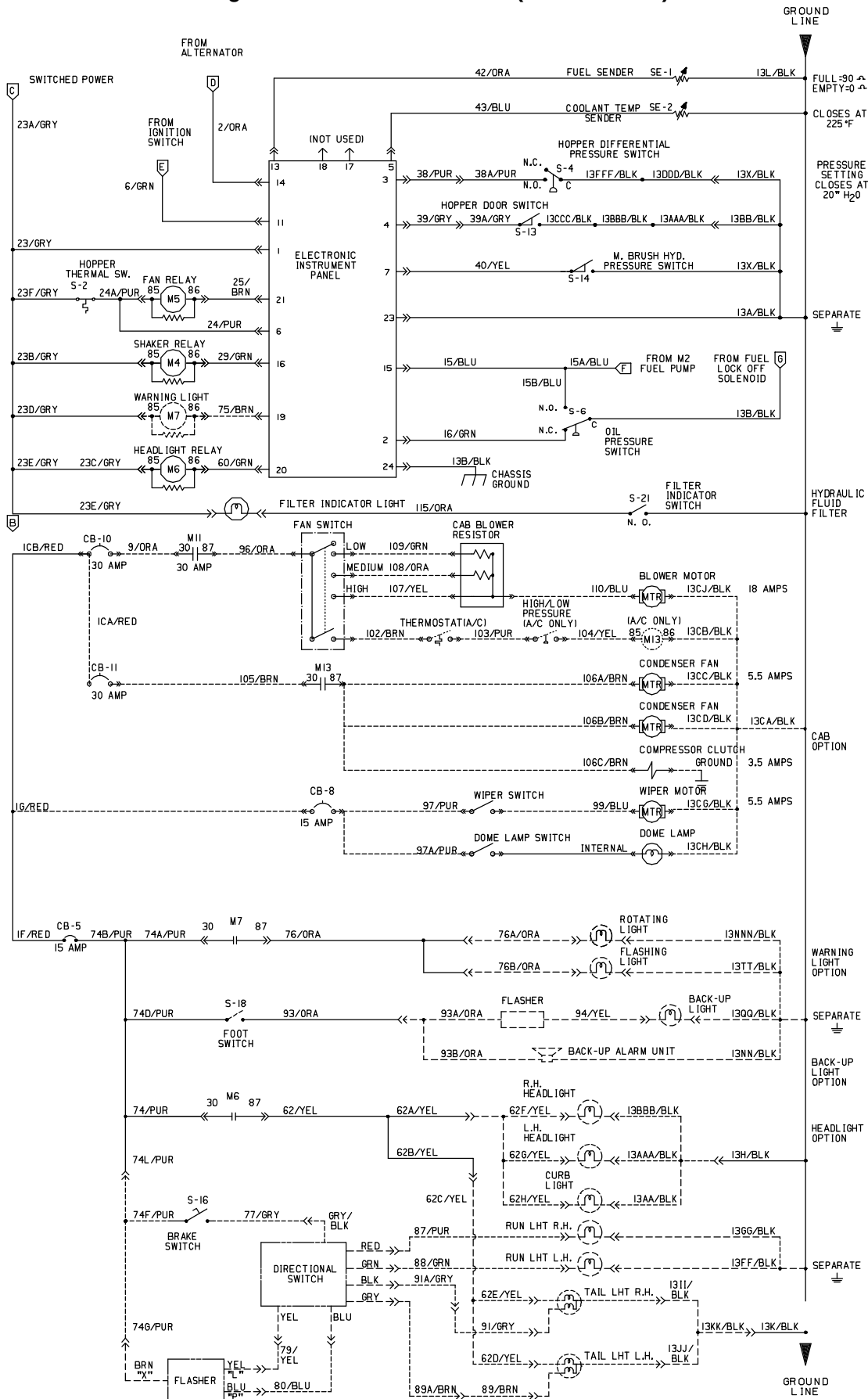
Fig. 61 – Electrical Schematic (006009– )
