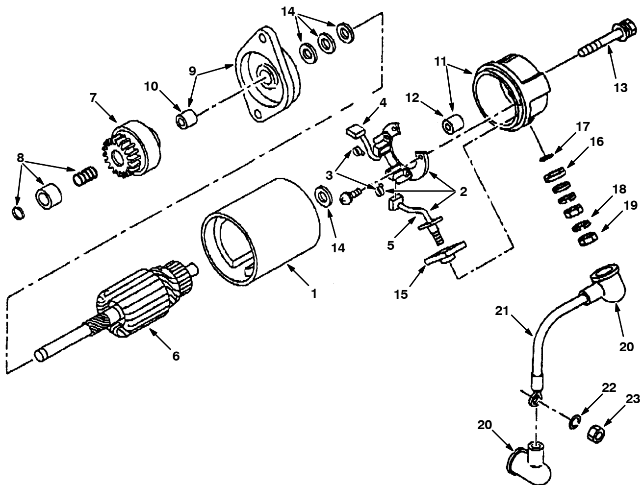
Fig. 13 - Starter Breakdown, 385966
