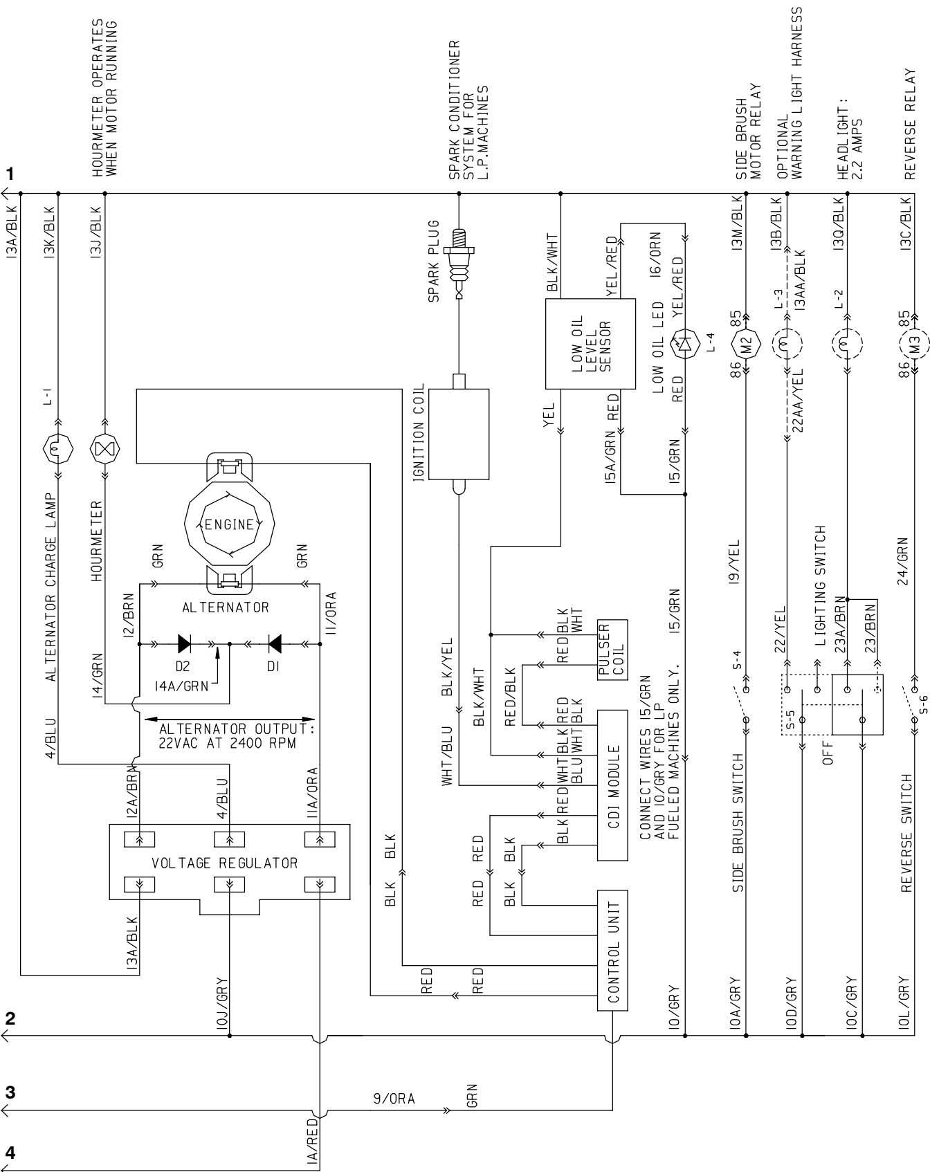
Fig. 37 - Electrical Schematic, LPG
