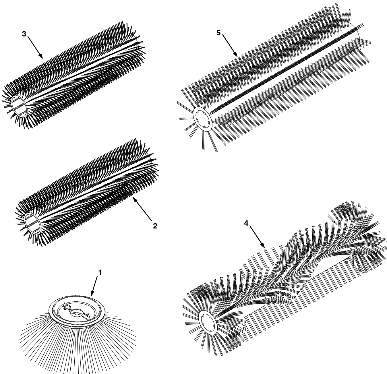
Fig. 2 - Replacement Brushes
