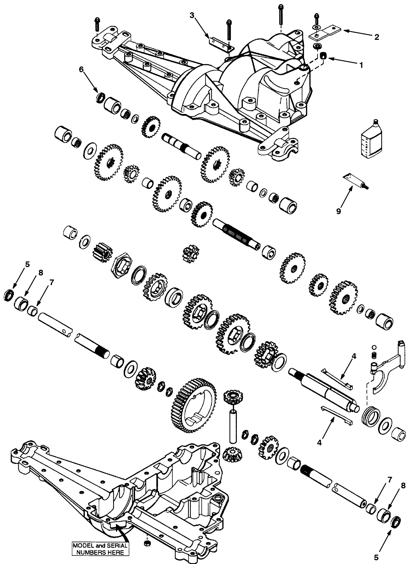
Fig. 1 - Transaxle Breakdown, 80476
