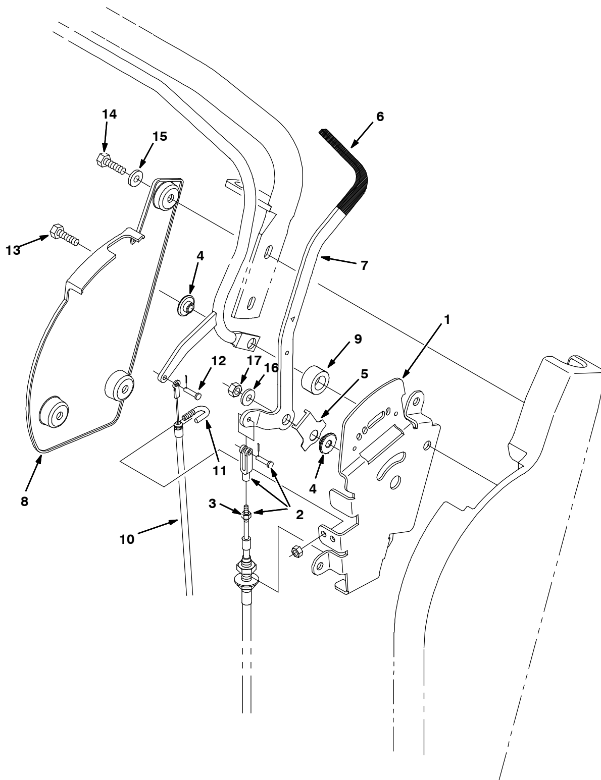
Fig. 11 - Clutch and Shift Handle Group
