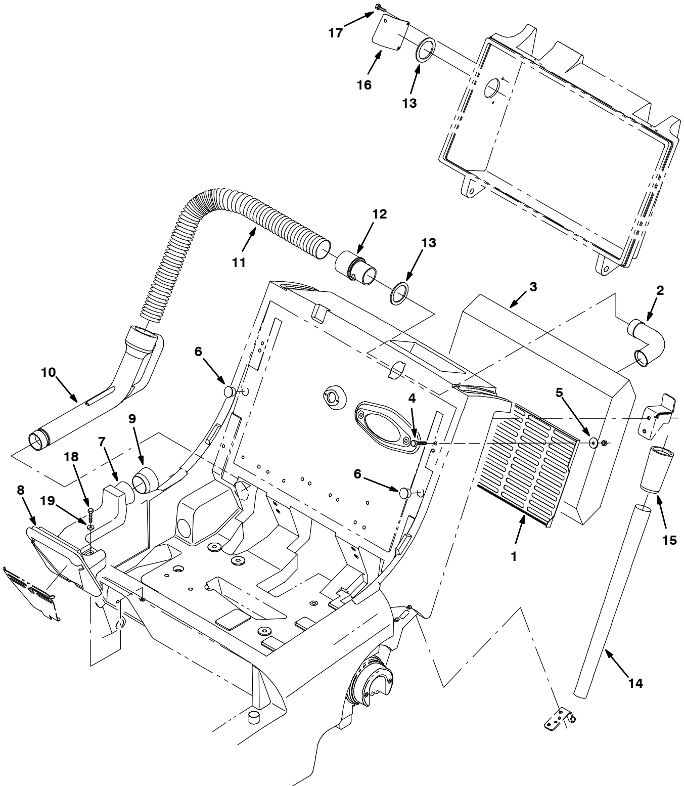
Fig. 7 - High Flow To Standard Bag Kit
