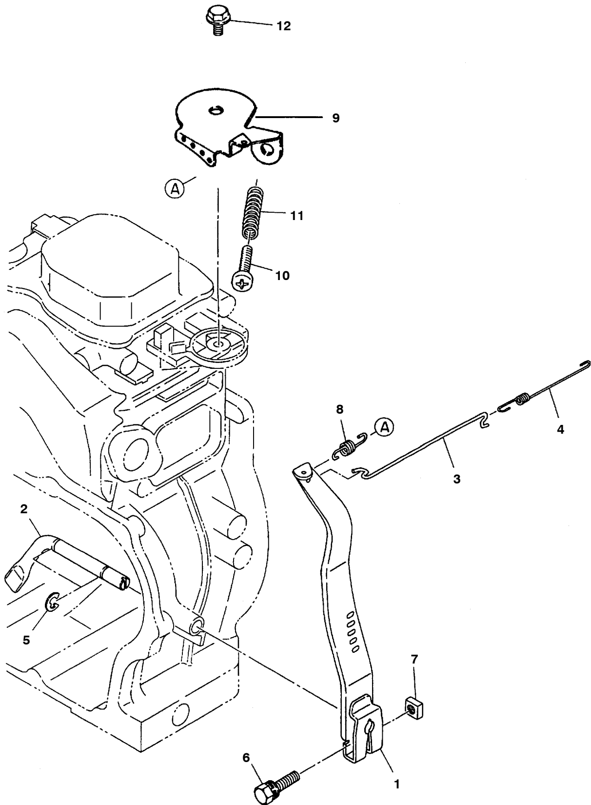
Fig. 4 - Governor Group
