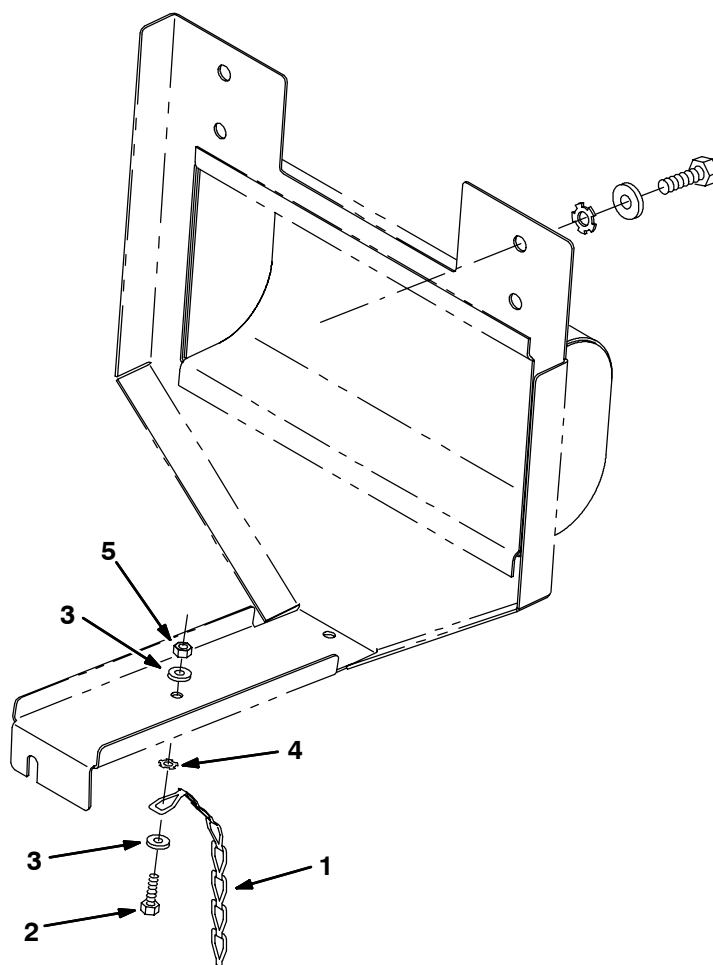
Fig. 13 - Steel Static Chain Kit
