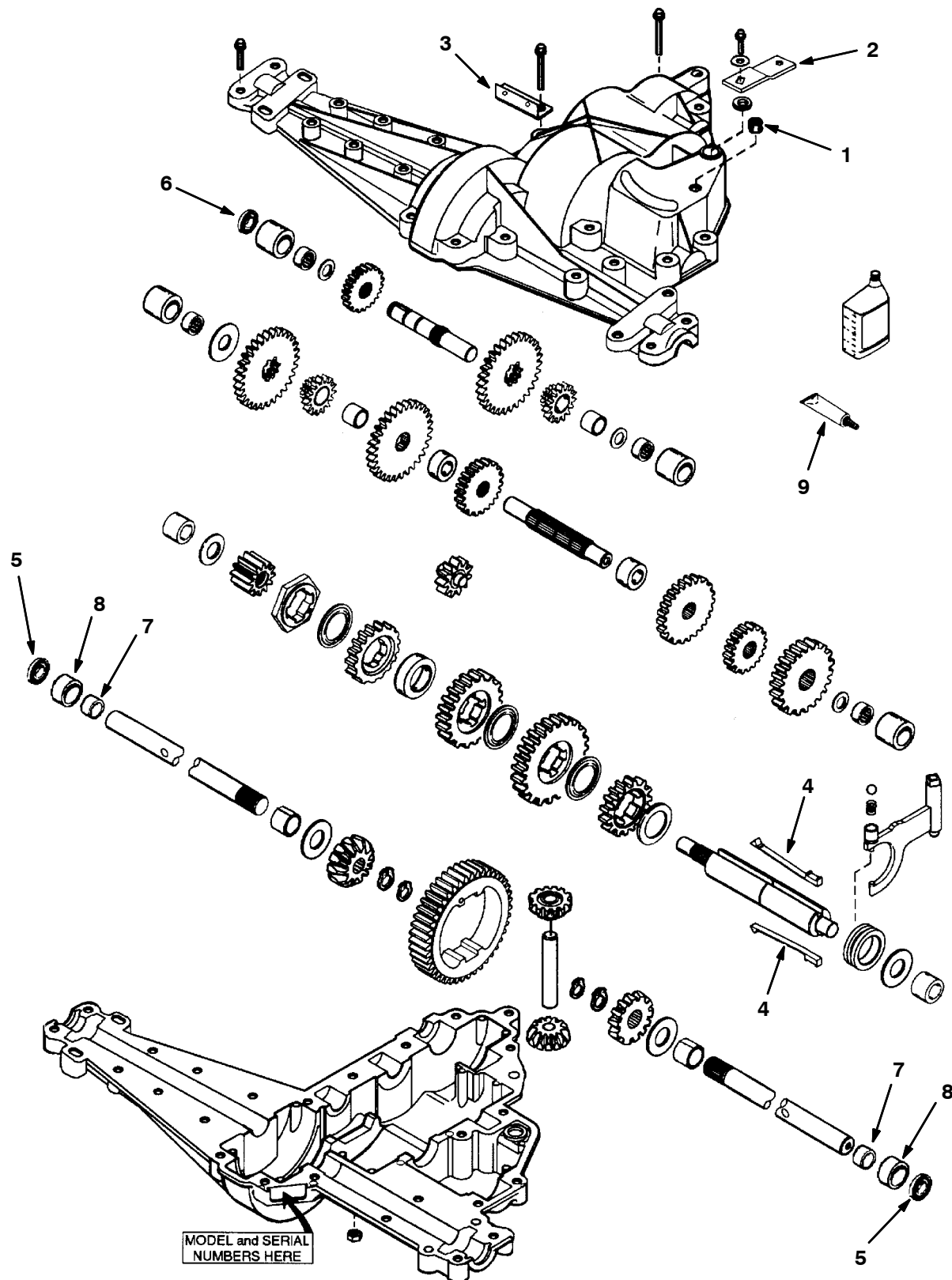
Fig. 1 - Transaxle Breakdown, 80476
