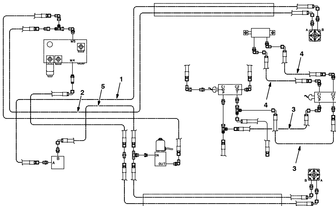
Fig. 15 - Side Brush Hydraulic Hose Group, L.H.
