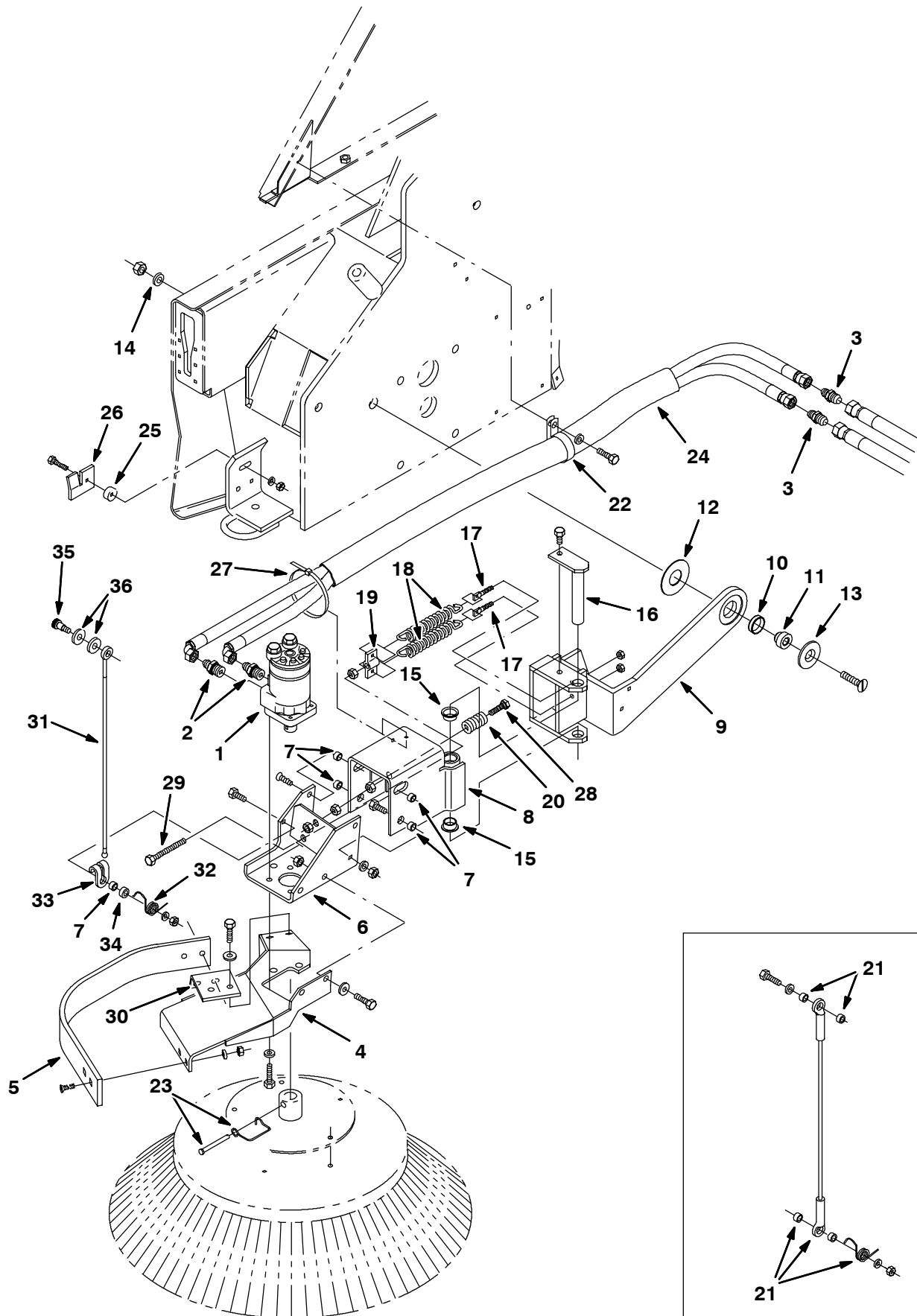
Fig. 41 - Side Brush Group
