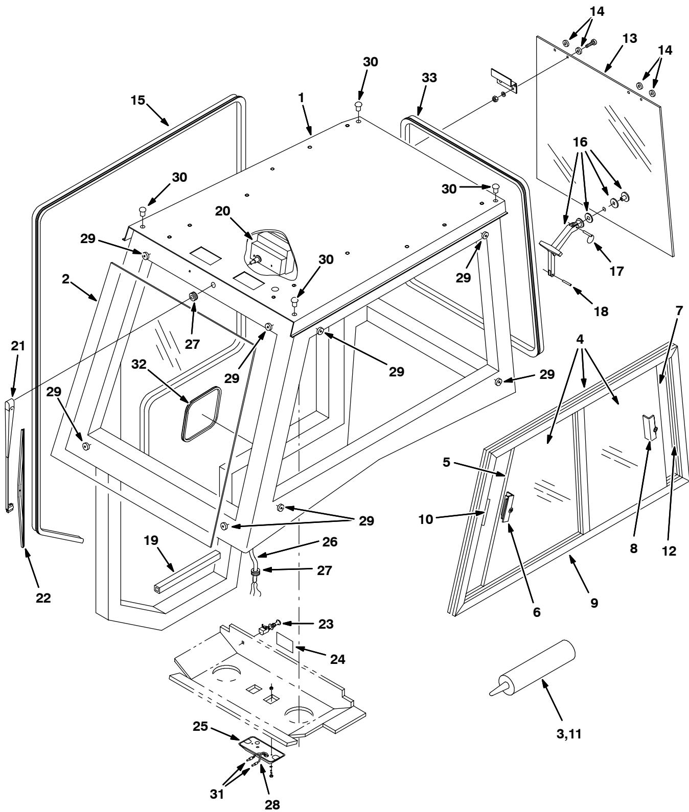
Fig. 16 - Cab Assembly
