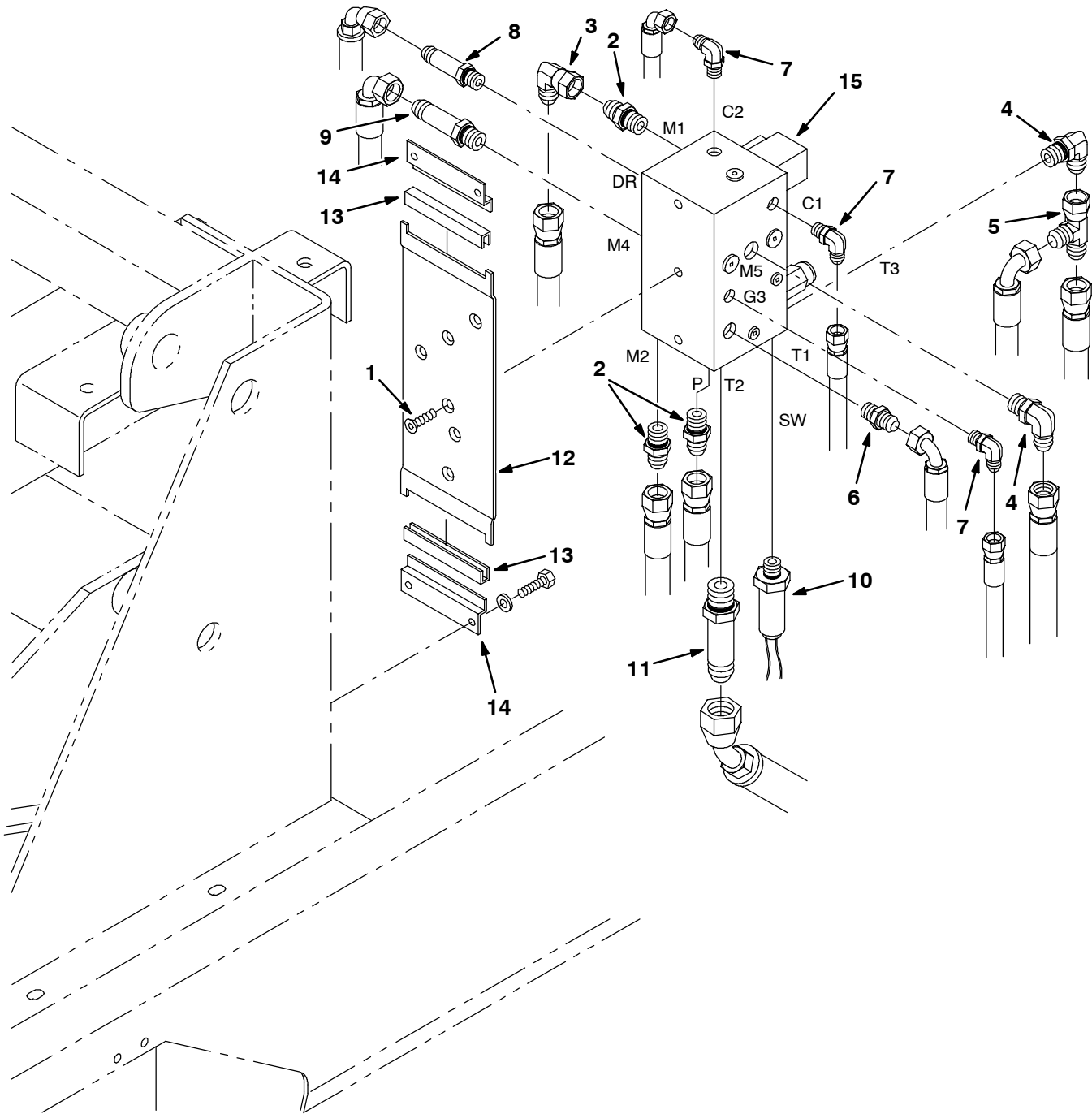
Fig. 39 - Hydraulic Solenoid Valve Group
