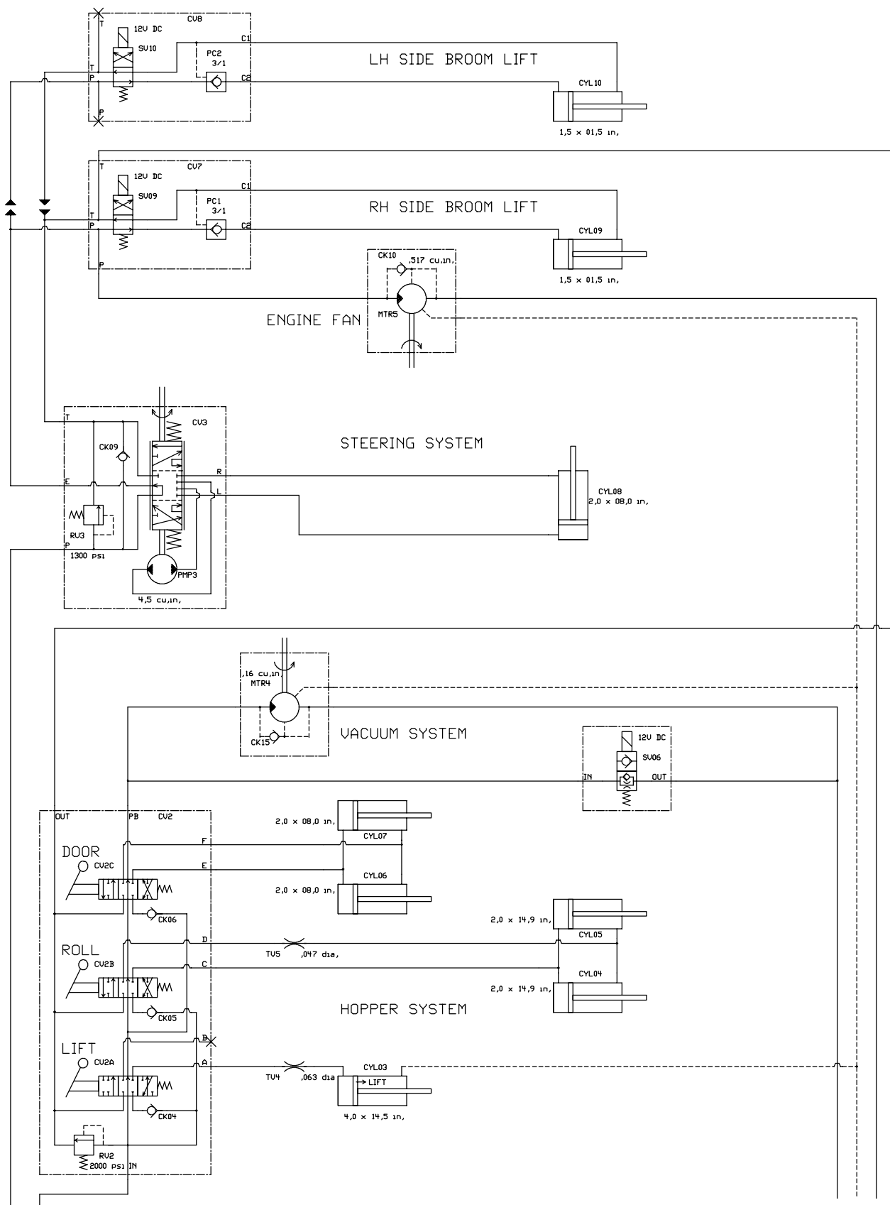
Fig. 35 - Hydraulic Schematic
