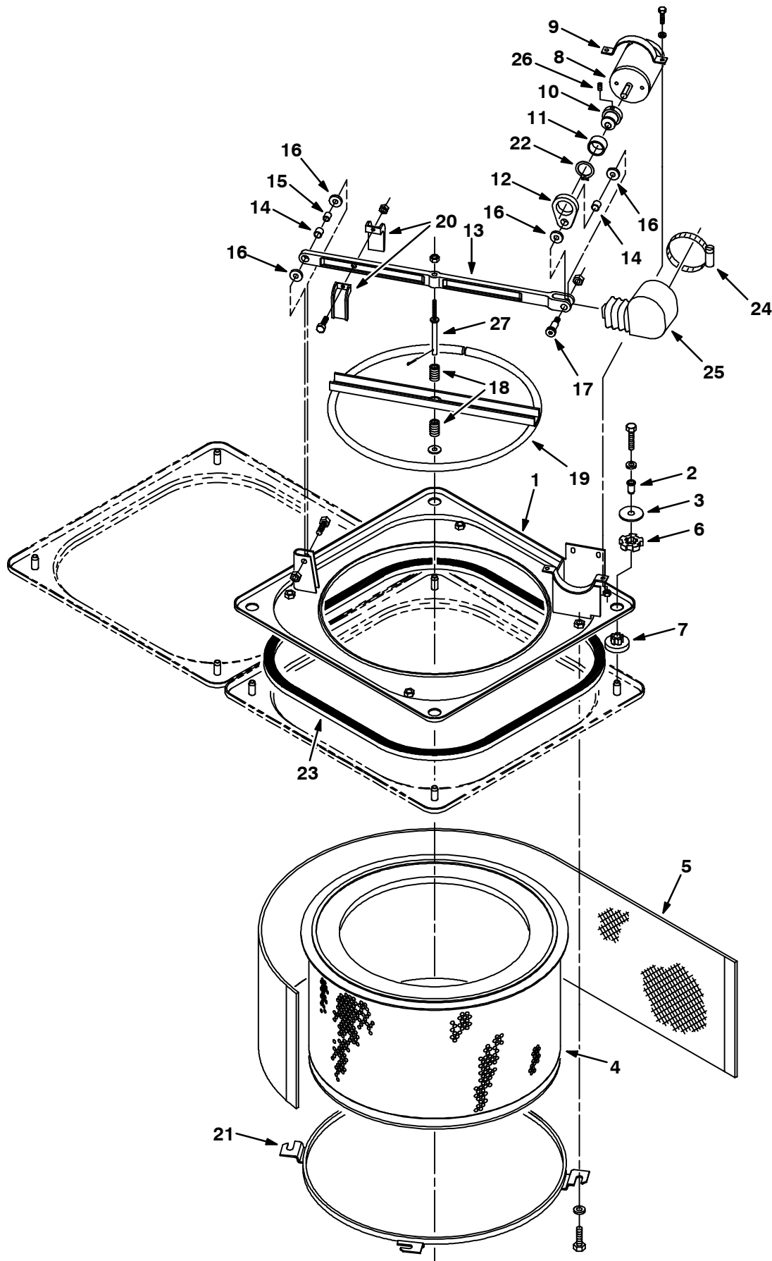
Fig. 16 - Filter Shaker Group
