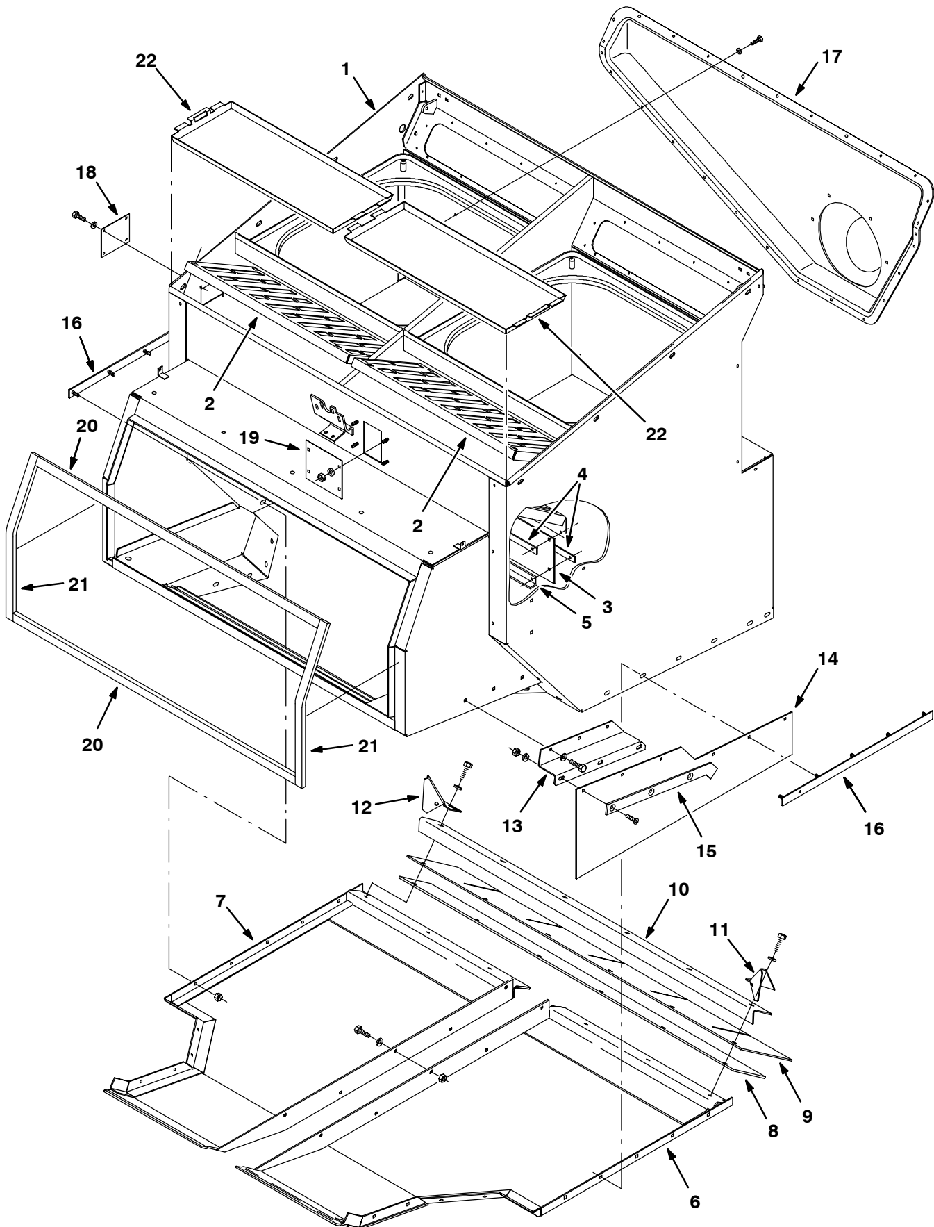
Fig. 12 - Hopper Group
