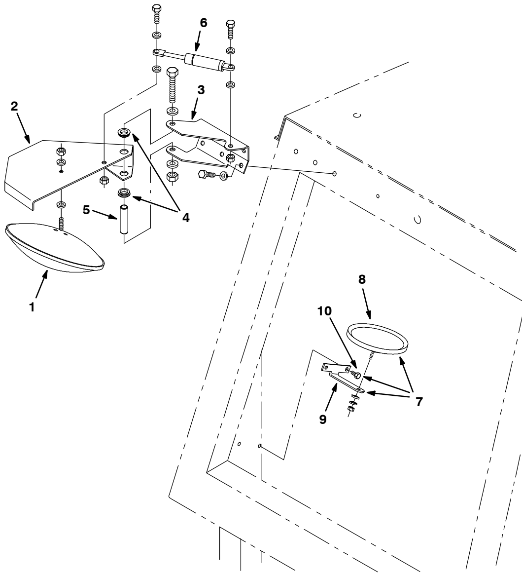
Fig. 18 - Mirror Kit
