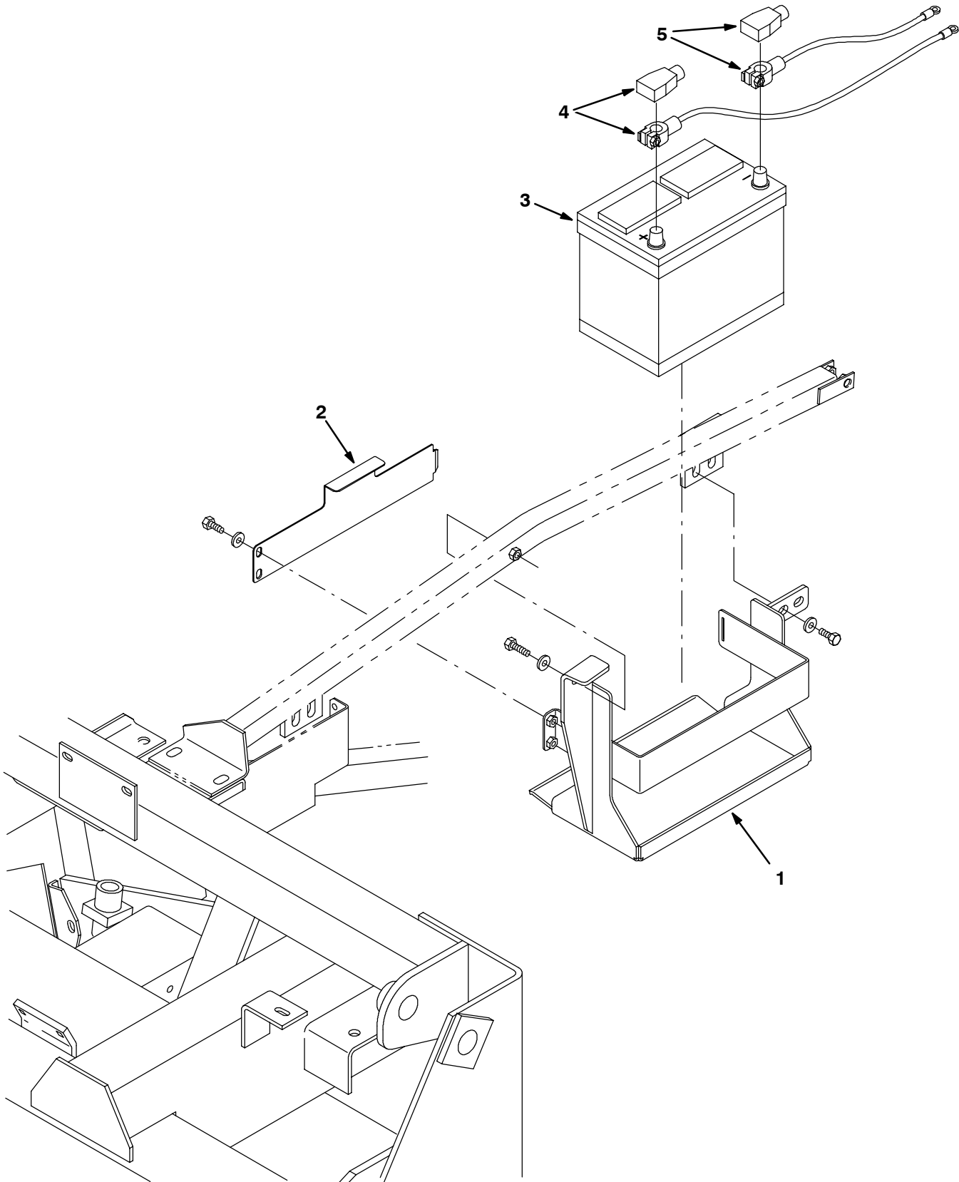
Fig. 28 - Battery Group
