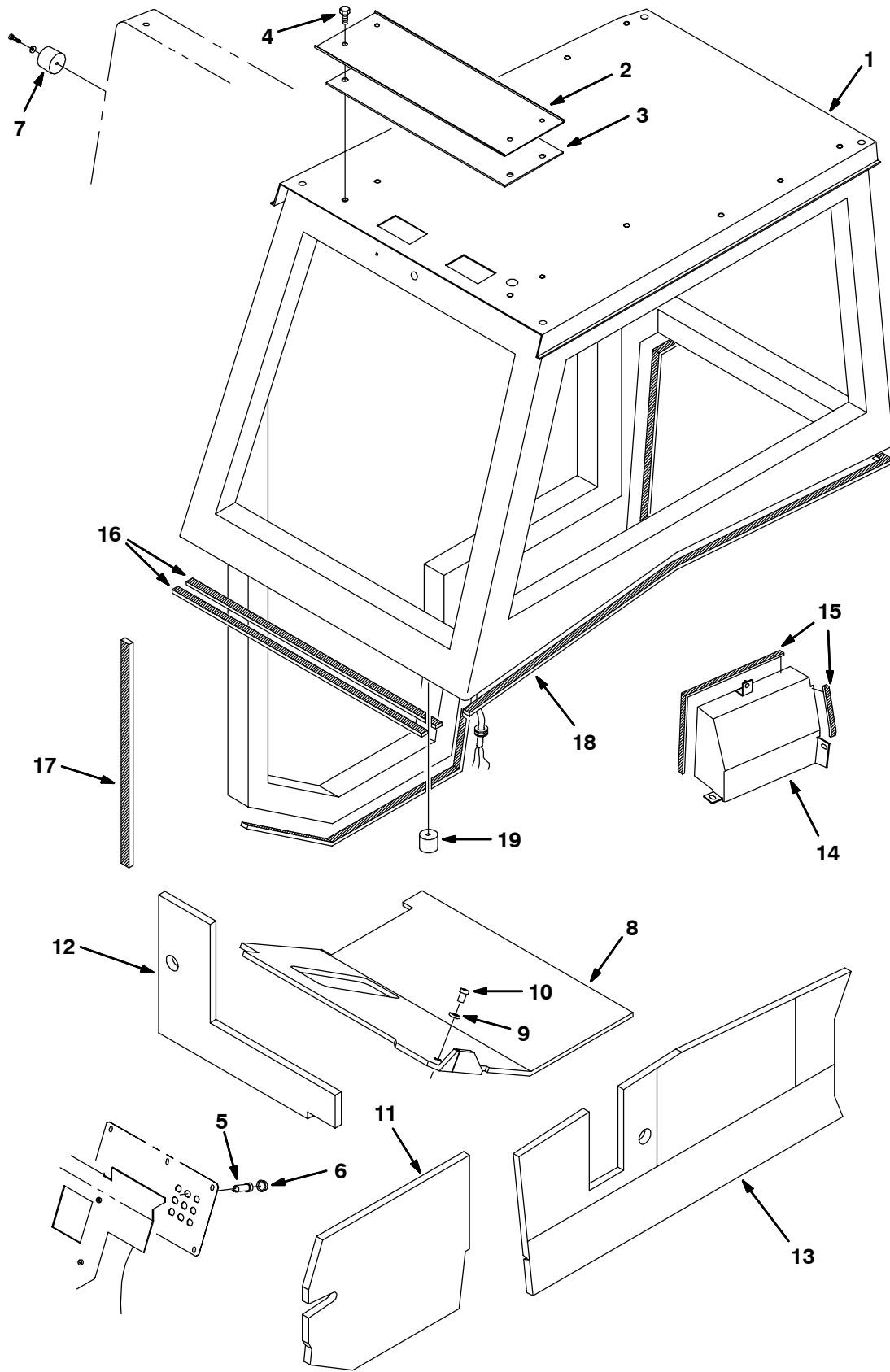
Fig. 17 - Cab Kit
