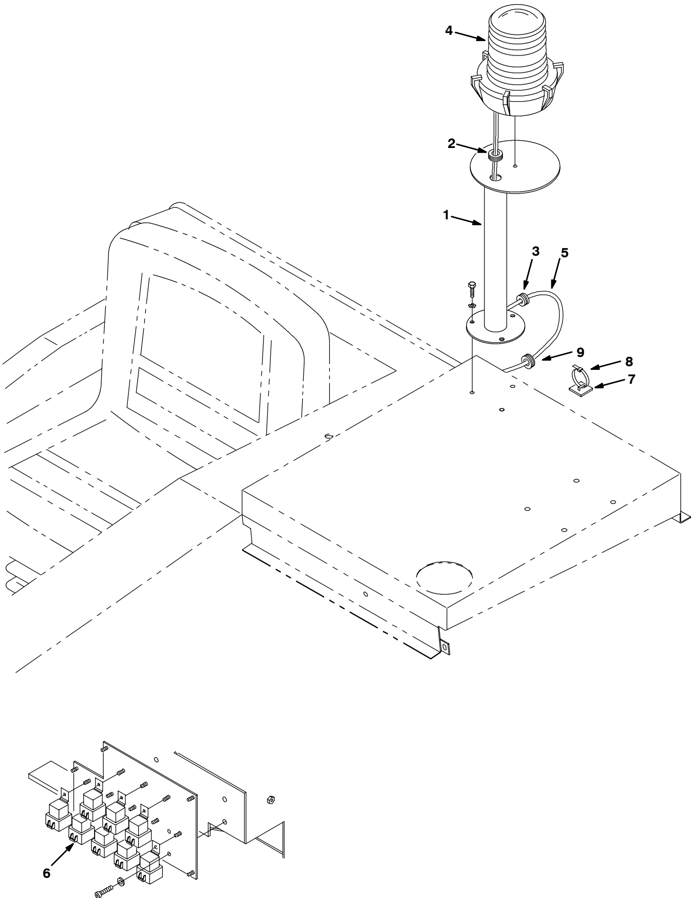
Fig. 5 - Flashing Light Kit, Low
