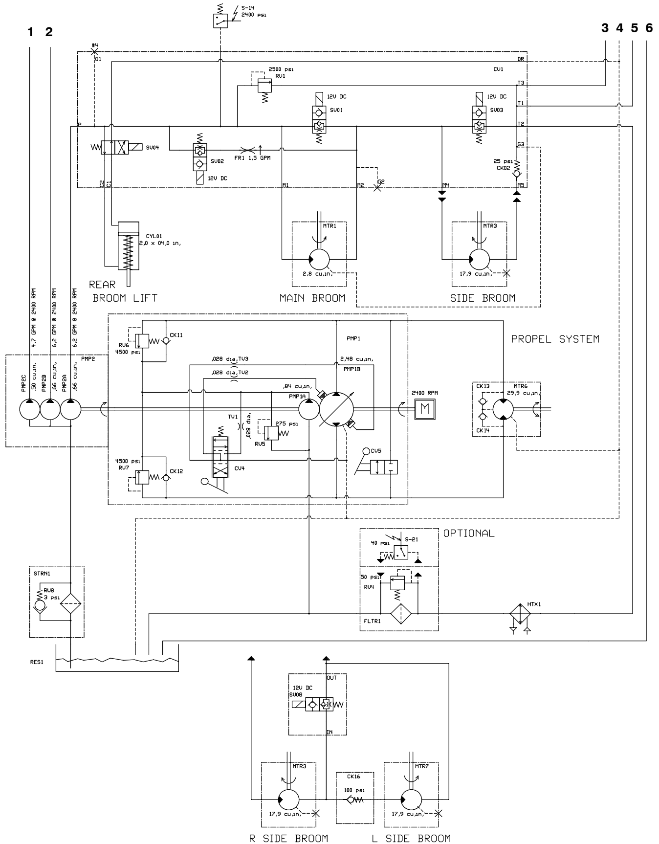
Fig. 35 - Hydraulic Schematic
