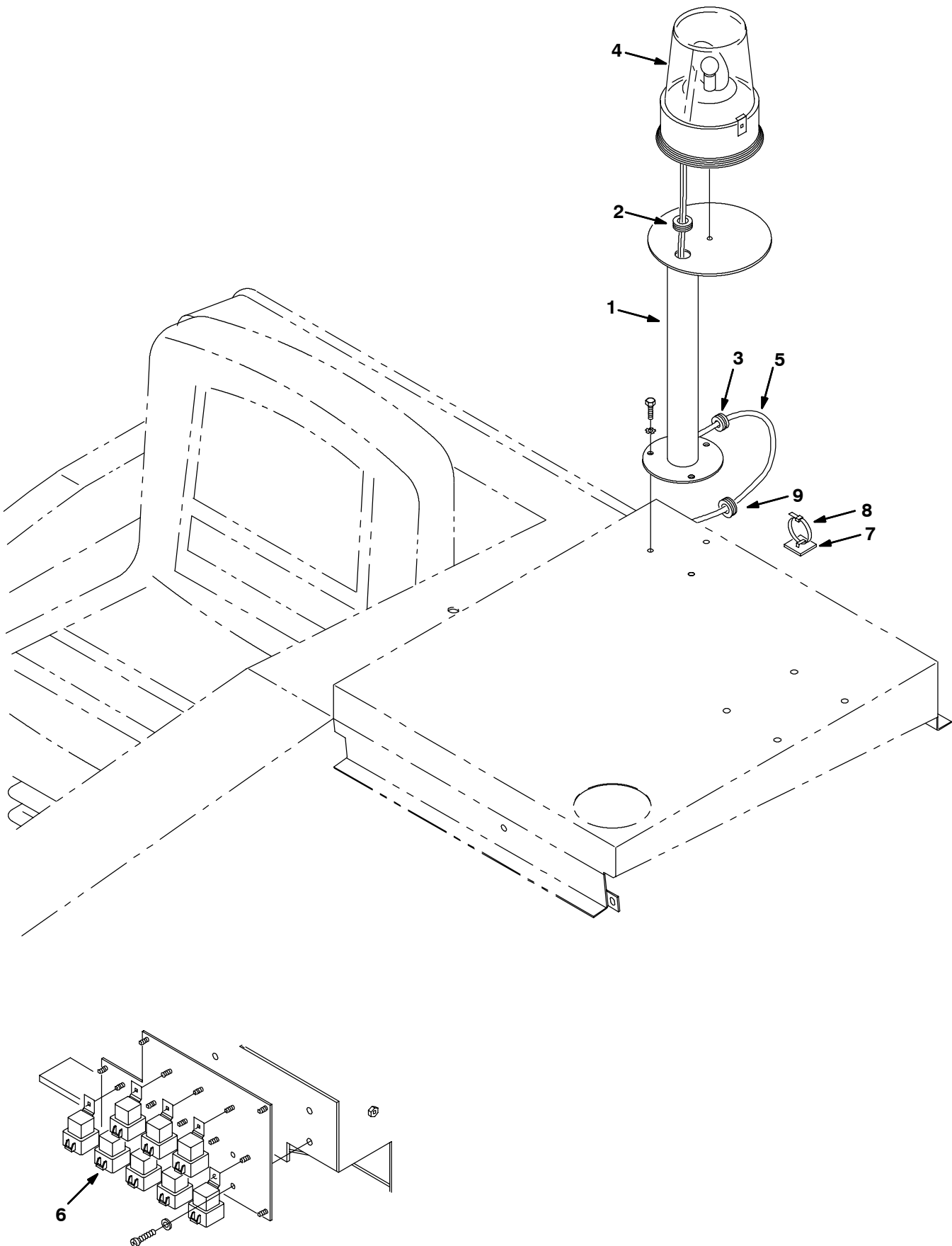
Fig. 6 - Revolving Light Kit, Low
