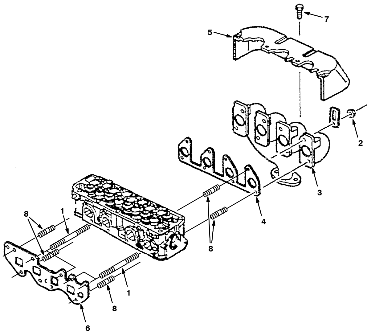
Fig. 5 – Manifold Group
