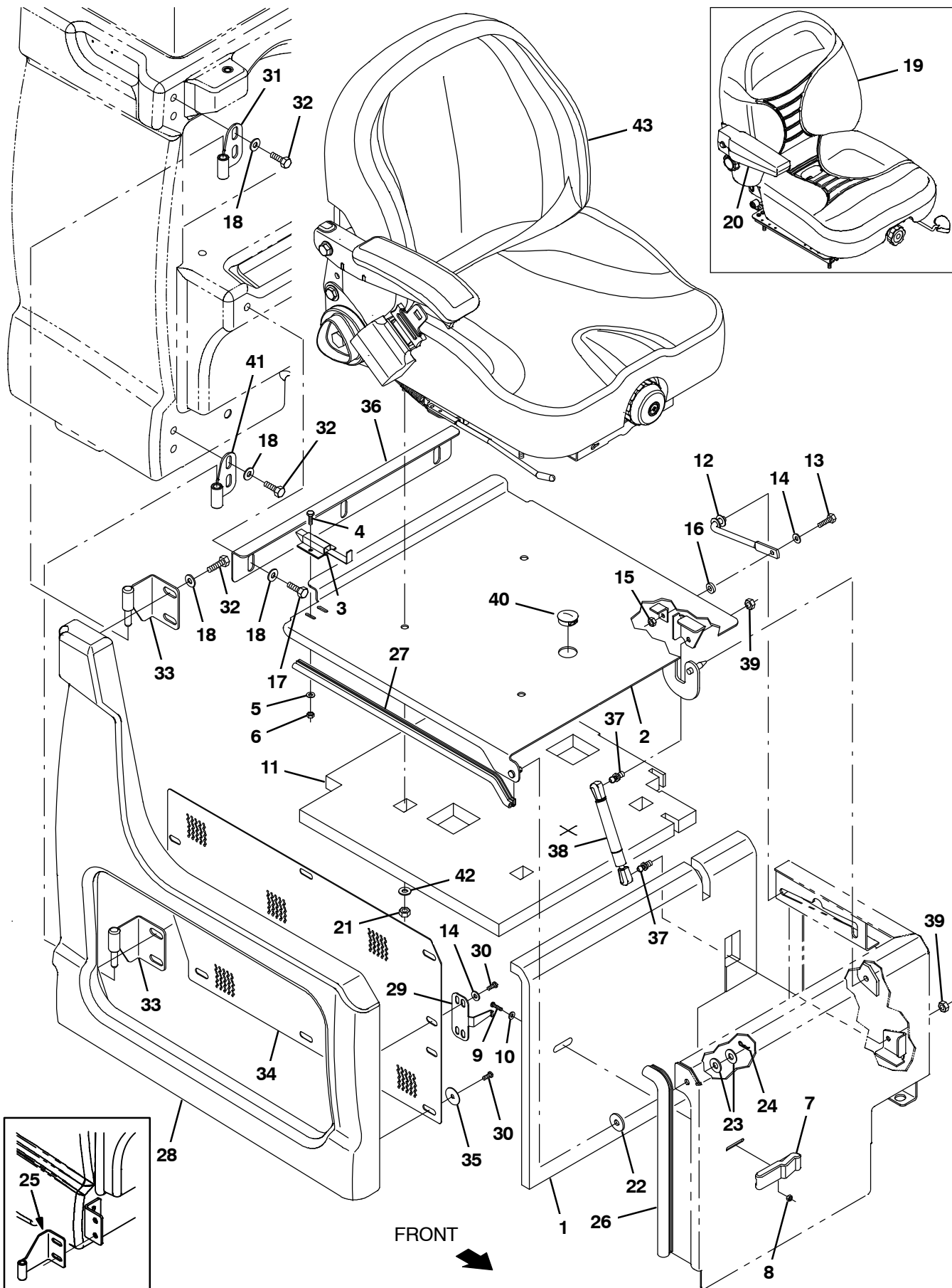
Fig. 7 – Seat Group
