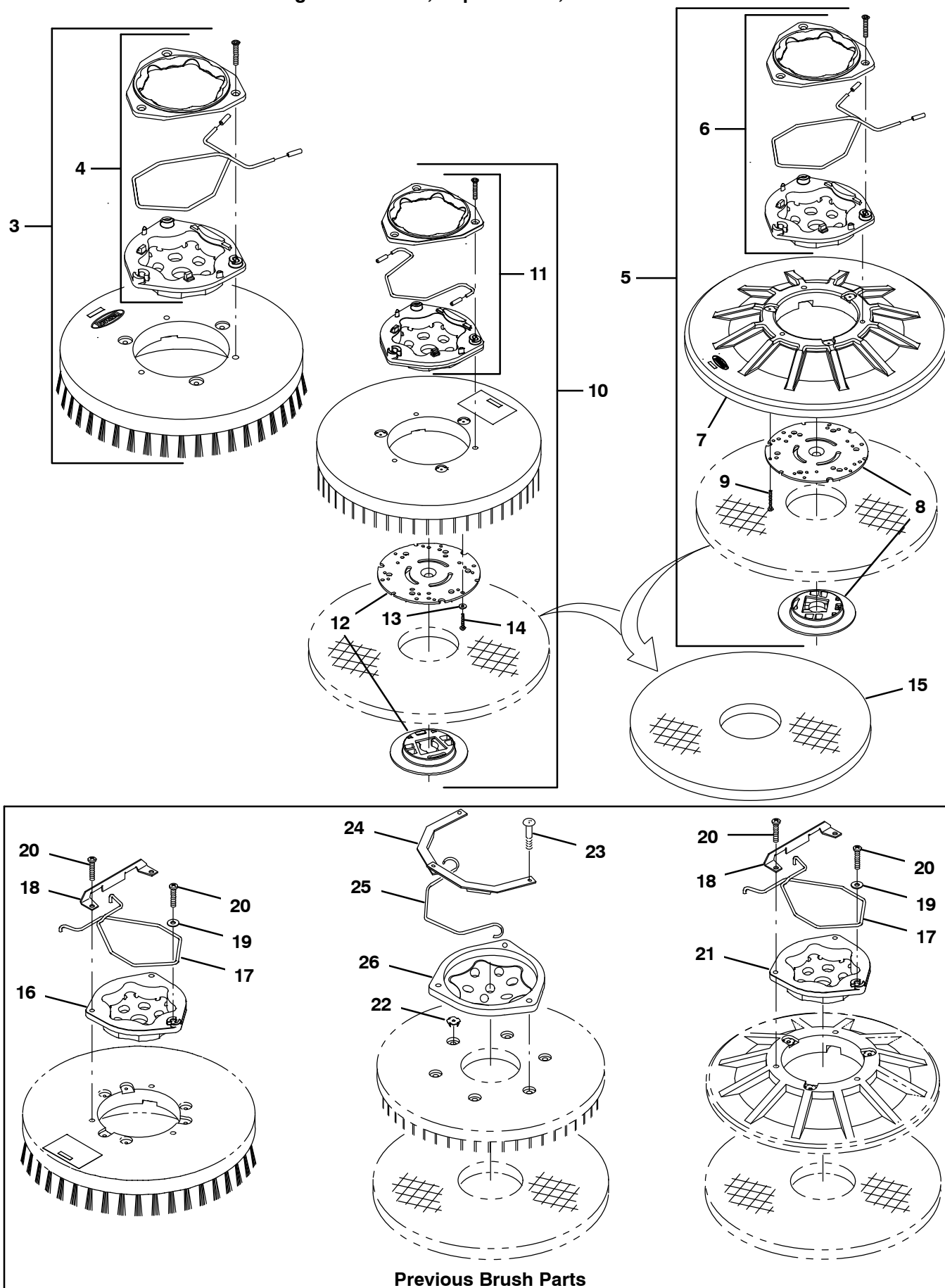
Fig. 1 – Brushes, Replacement, Scrub Head
