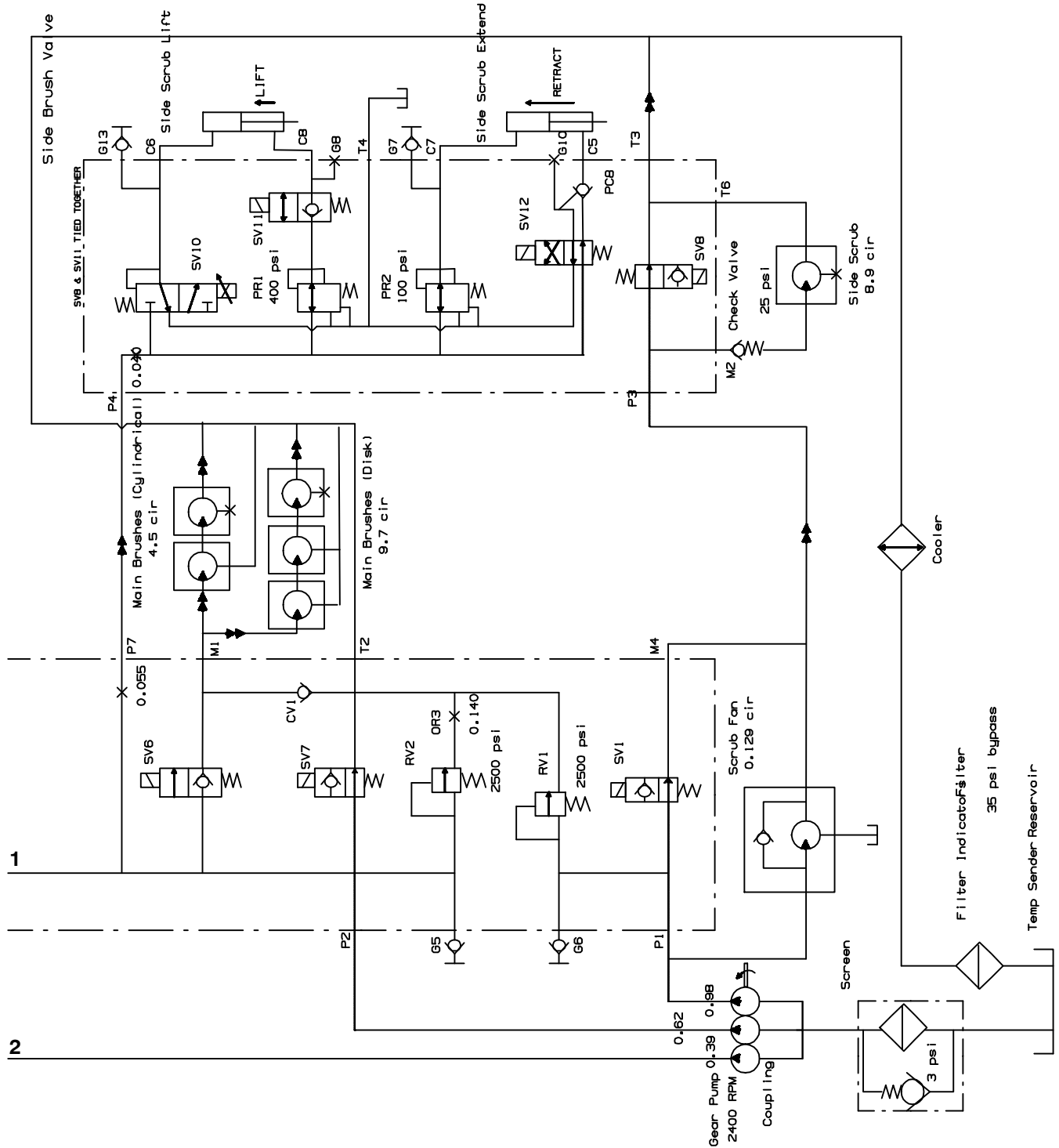
Fig. 72 – Hydraulic Schematic (001504-002282)
