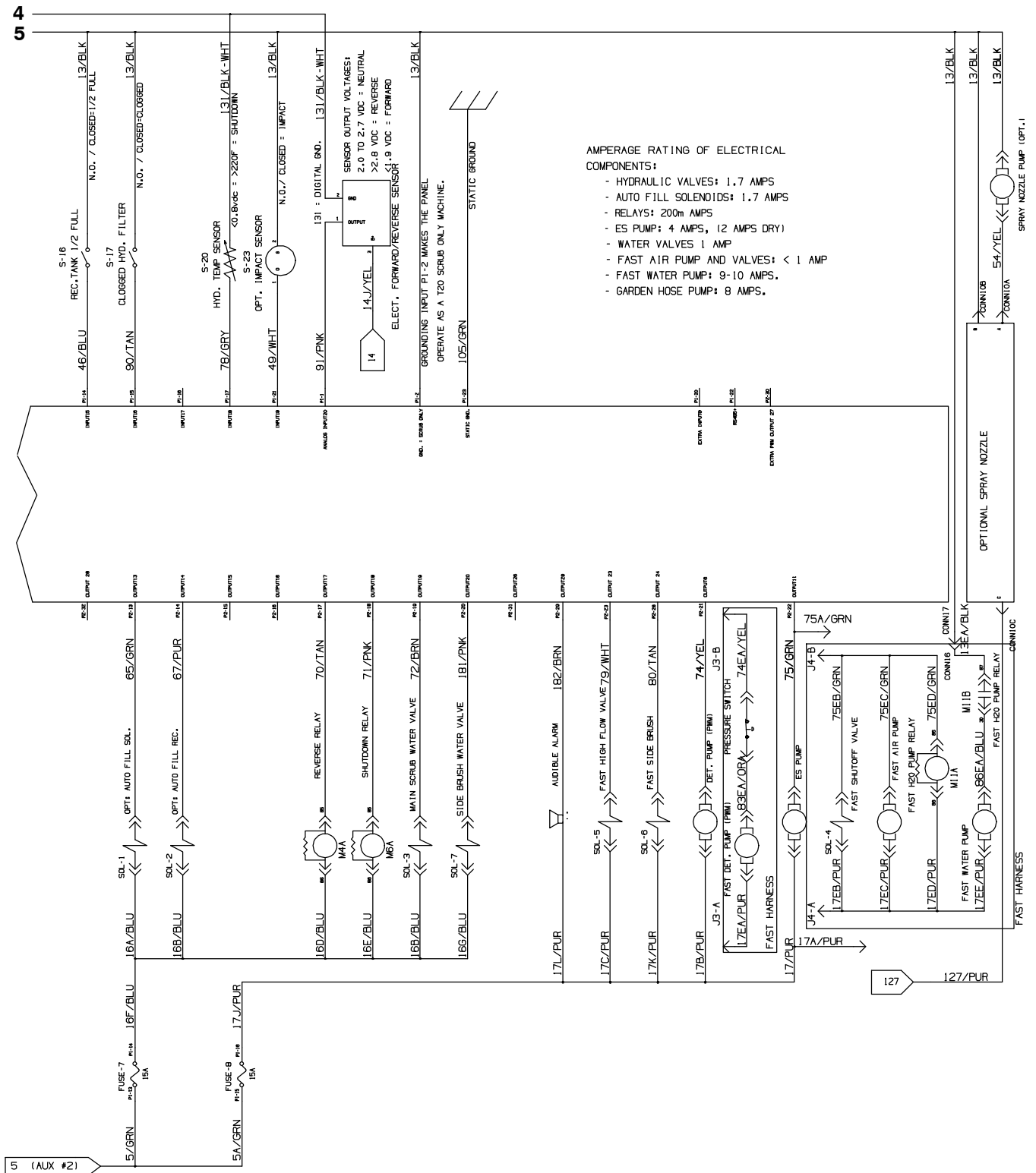
Fig. 83 –GM Electrical Schematic (000000–001499)
