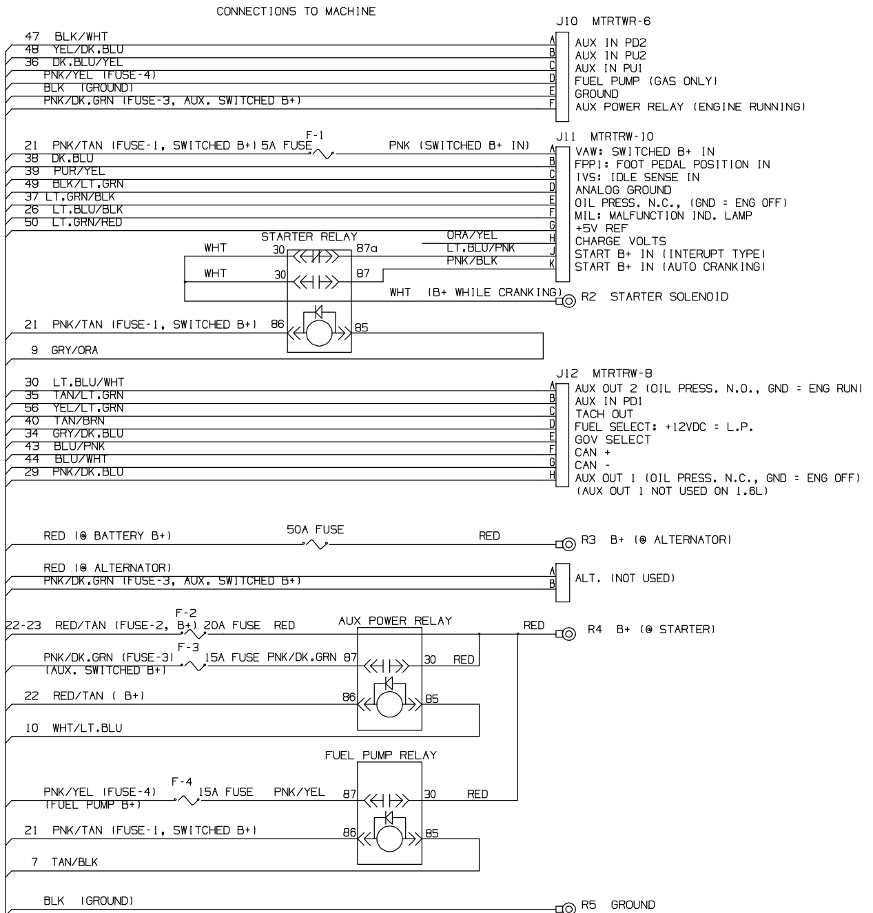
Fig. 86 – GM Electrical Schematic, Gasoline/LPG Engine Harness (000000–001499)
