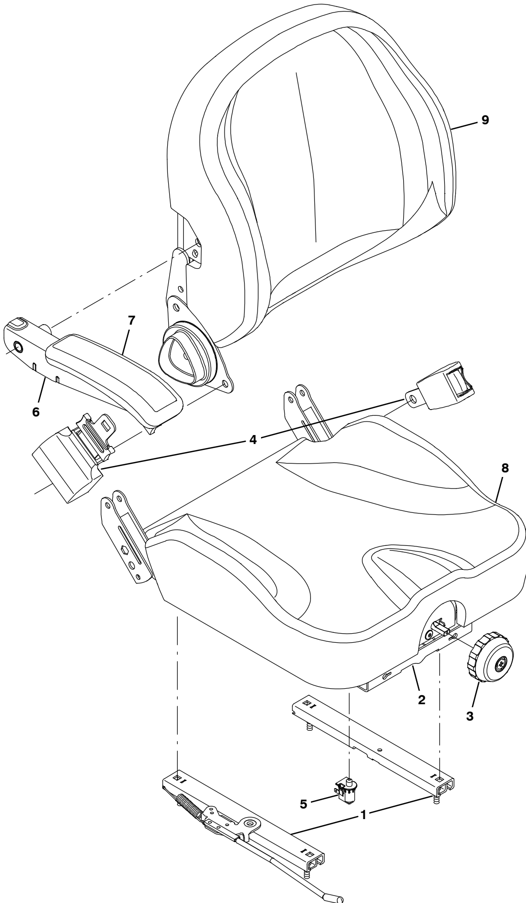
Fig. 17 – Seat Breakdown, 1072456
