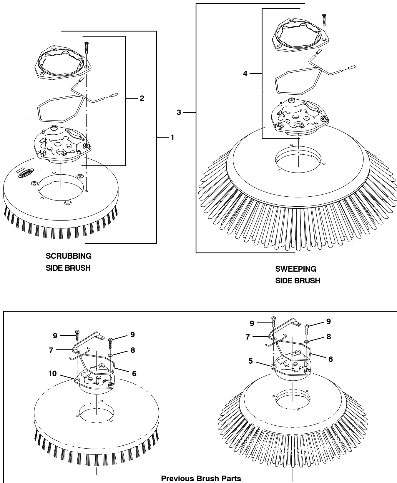
Fig. 2 – Brushes, Replacement, Side Brush
