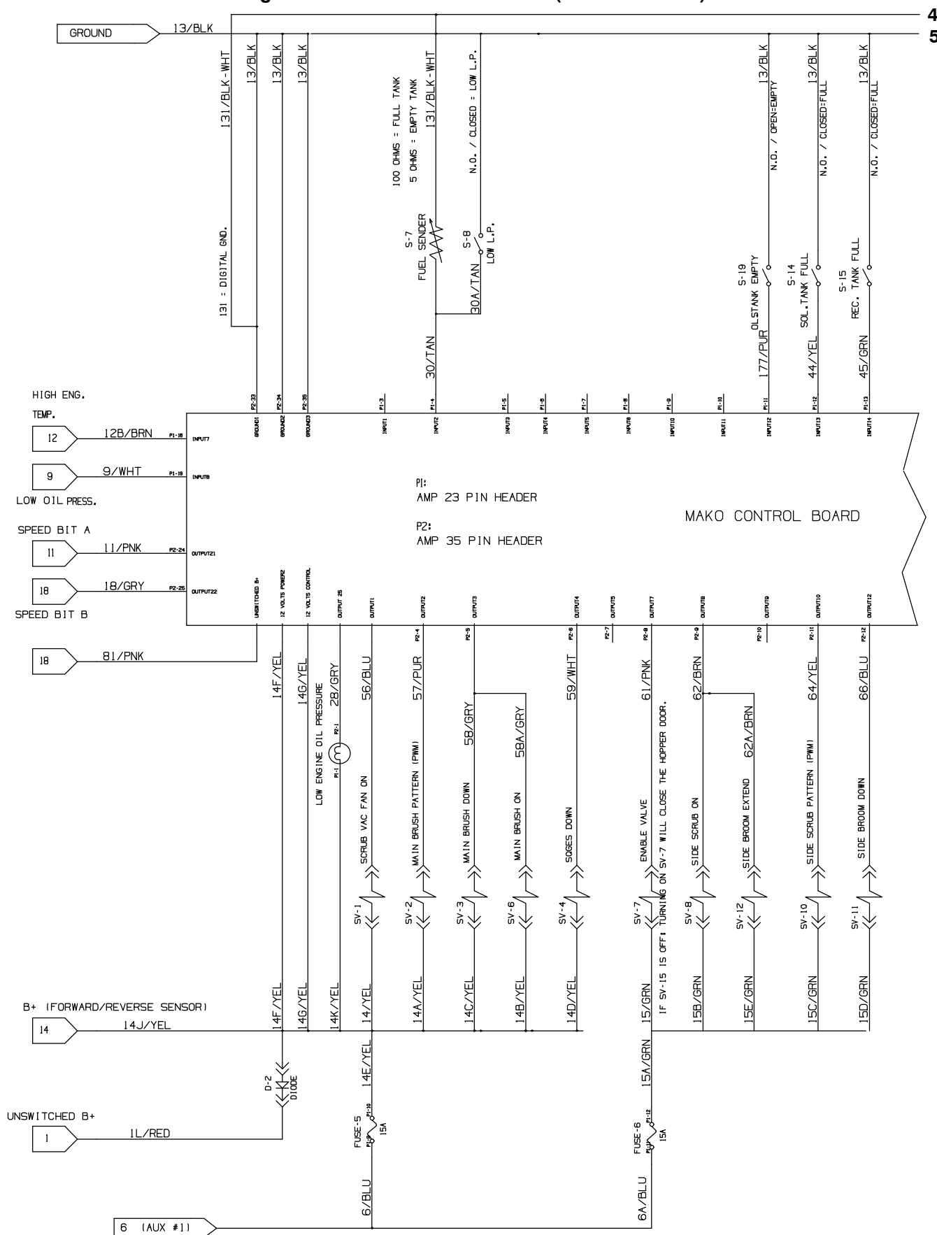
Fig. 83 – GM Electrical Schematic (000000–001499)
