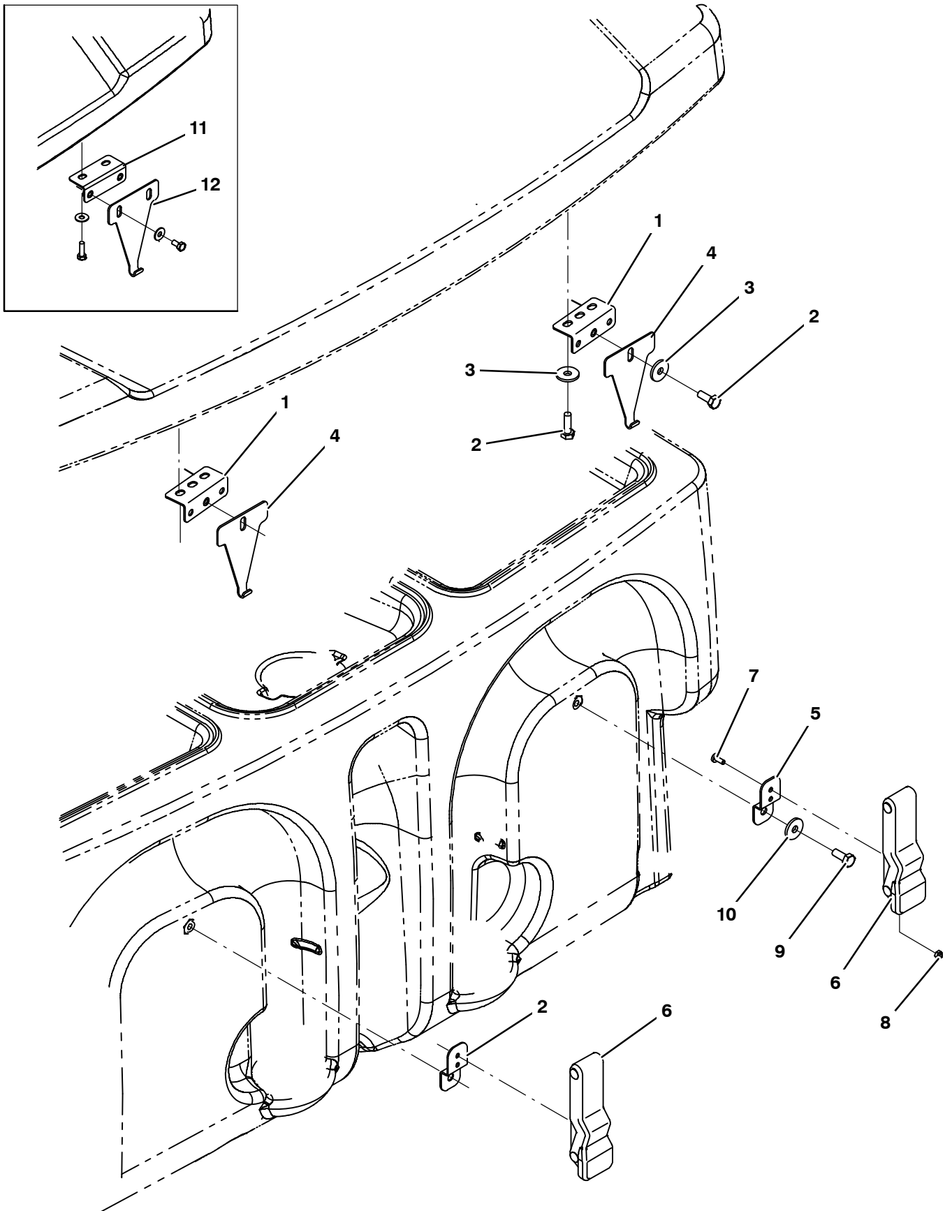
Fig. 45 – Transport Kit
