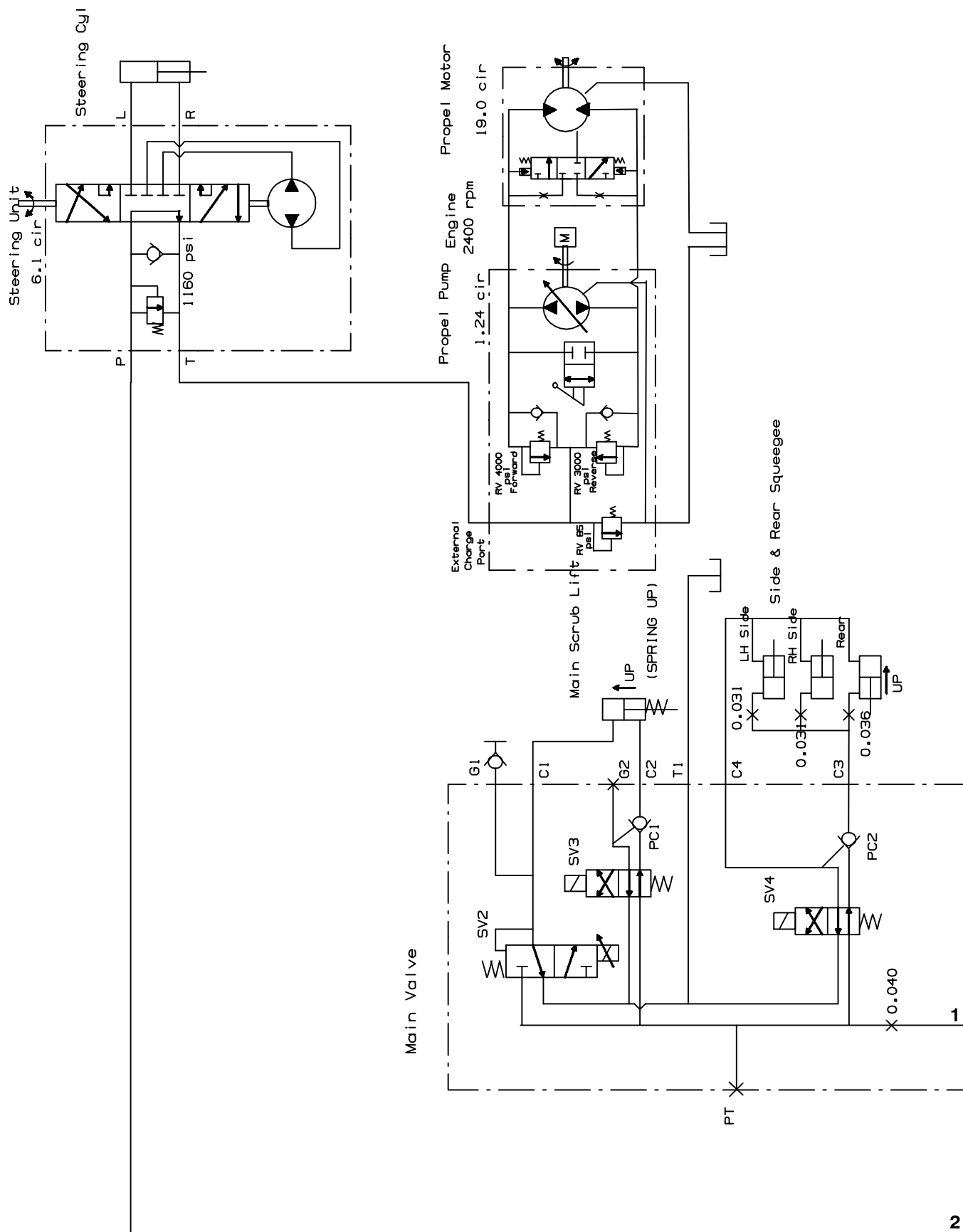
Fig. 72 – Hydraulic Schematic (001504-002282)
