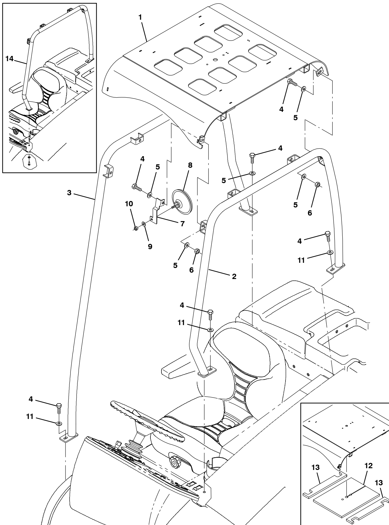
Fig. 34 – Overhead Guard Kit
