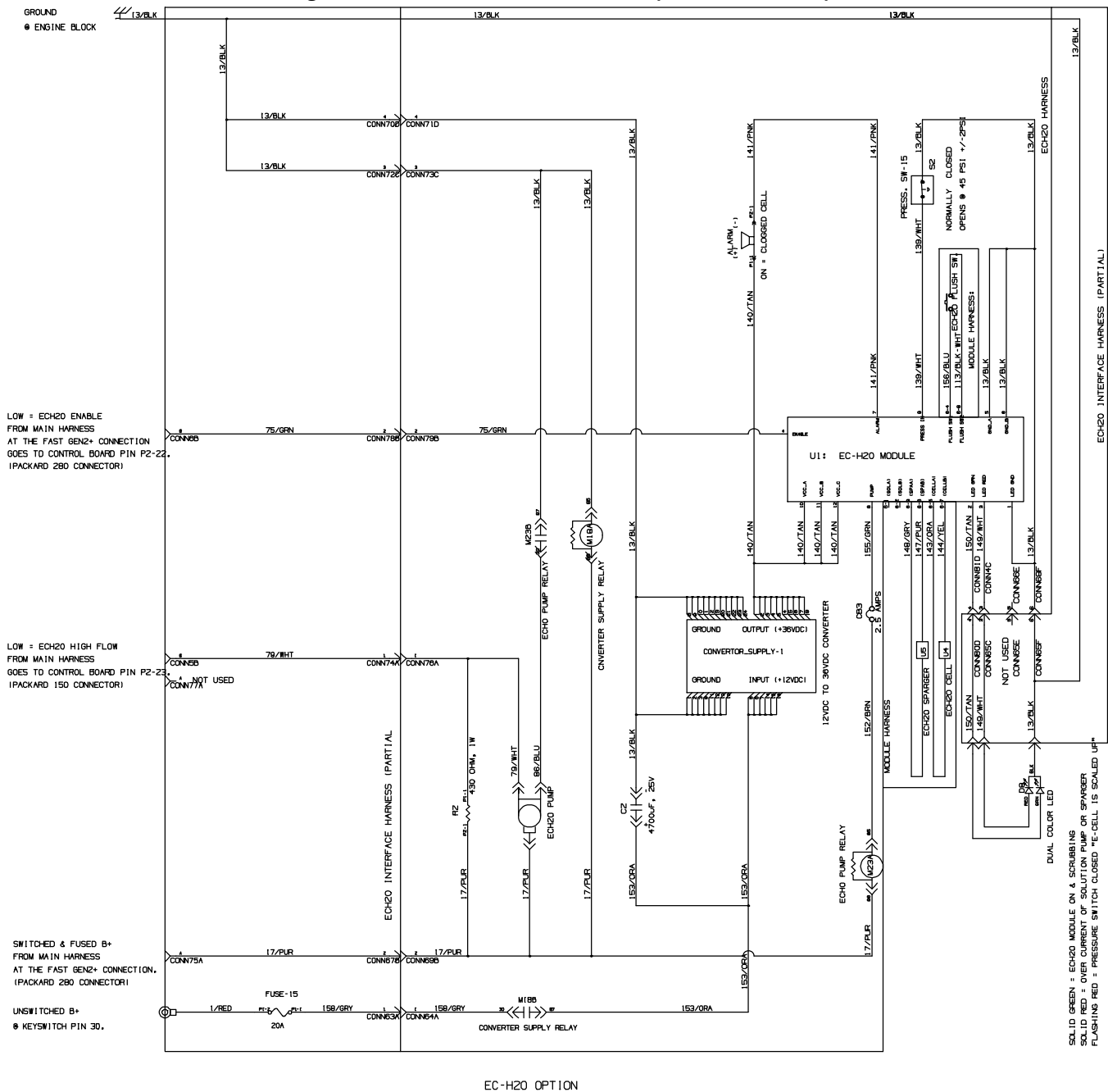
Fig. 85 – GM Electrical Schematic (001743–004999)
