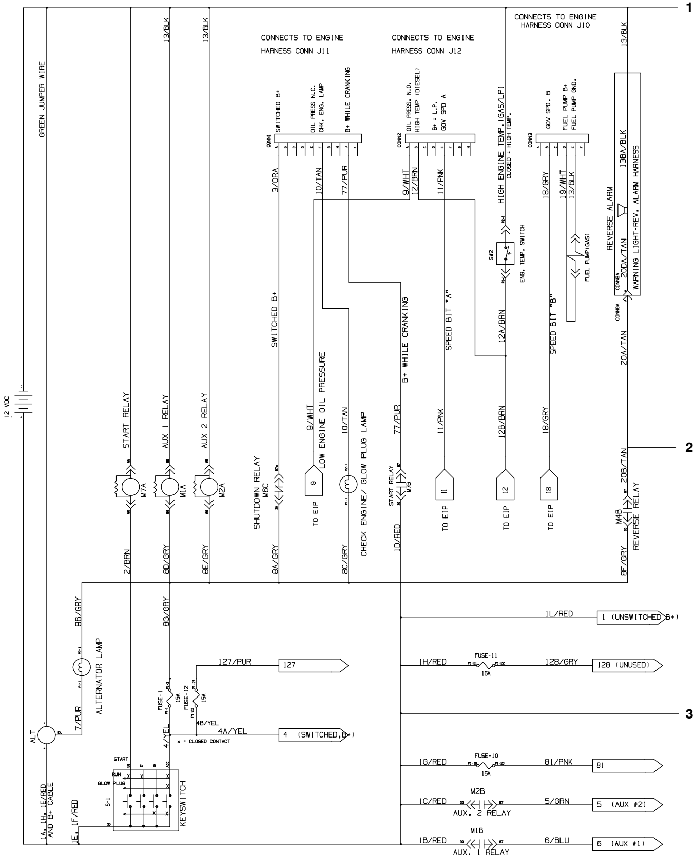
Fig. 62 – Electrical Schematic (000000-001742)
