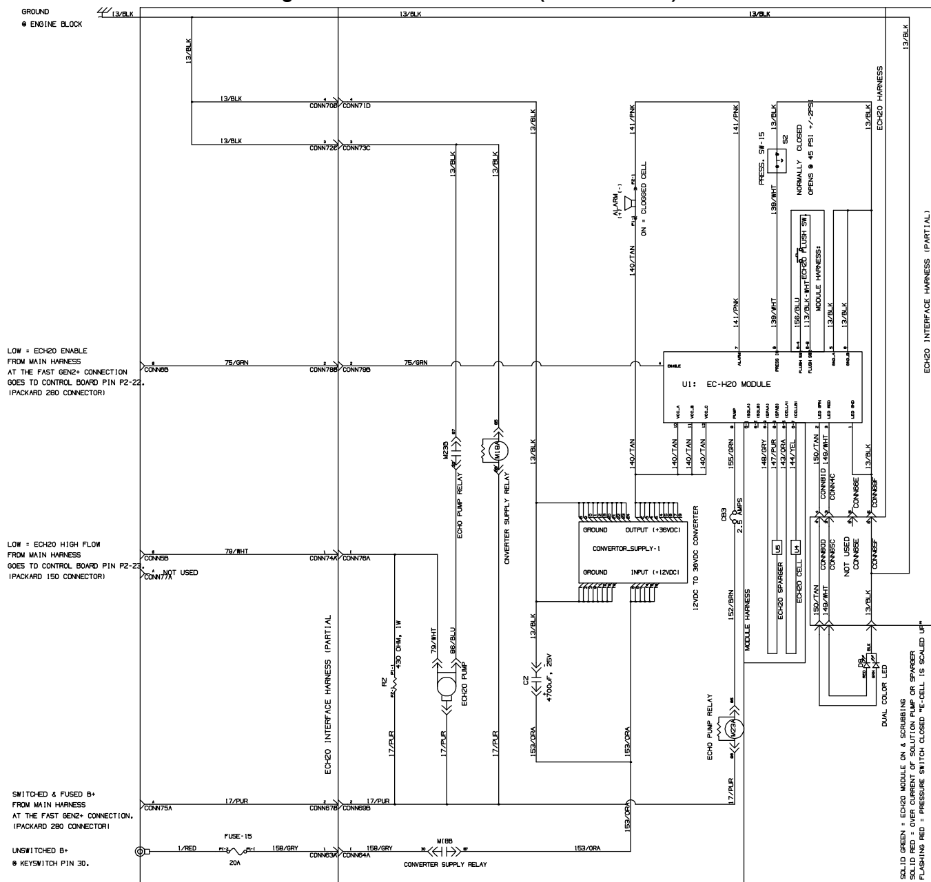
Fig. 63 – Electrical Schematic (001743– )
