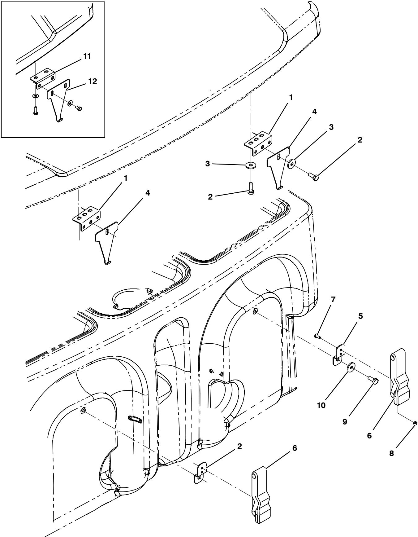
Fig. 45 – Transport Group
