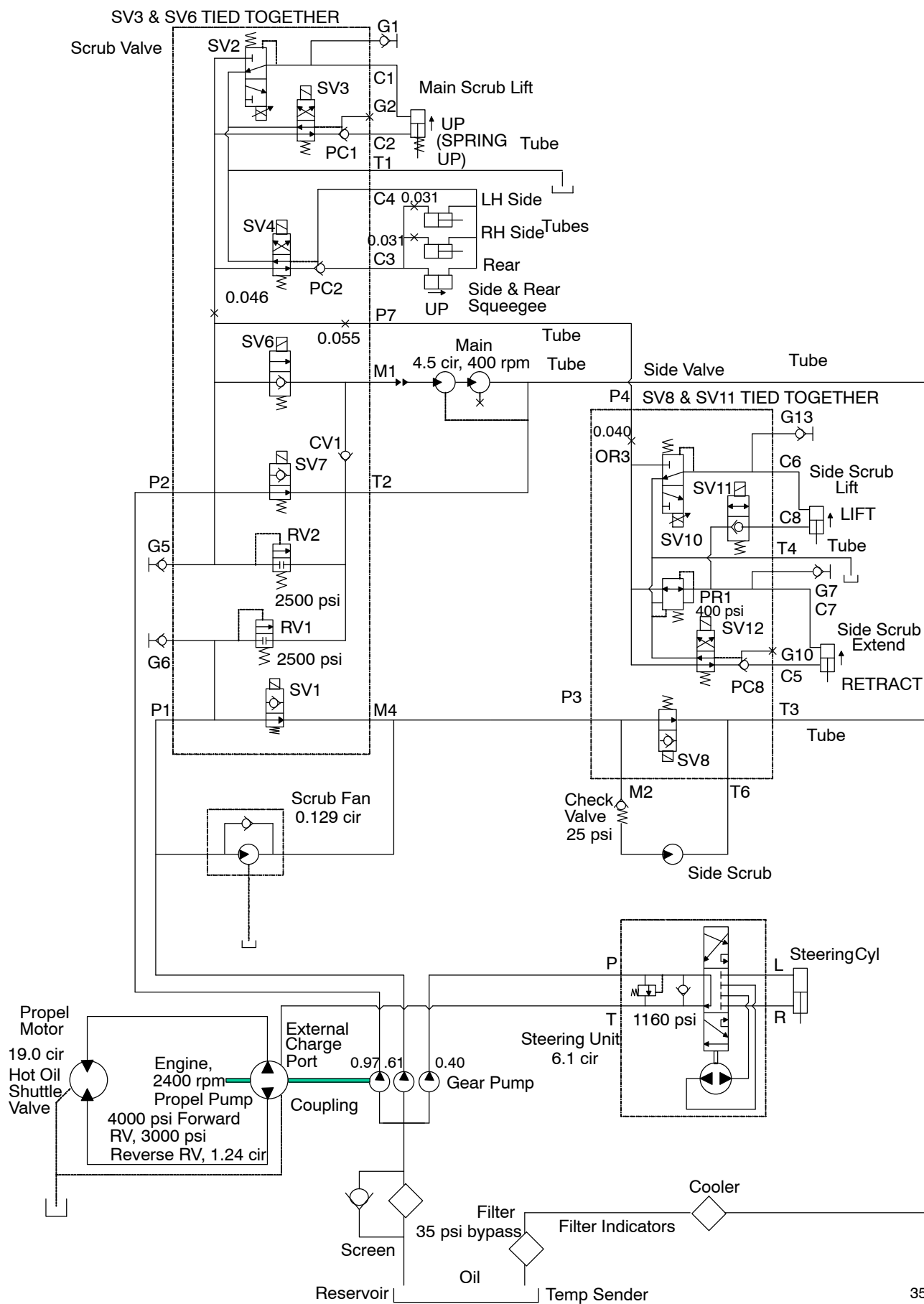
Fig. 50 – Hydraulic Schematic (000000-001503)
