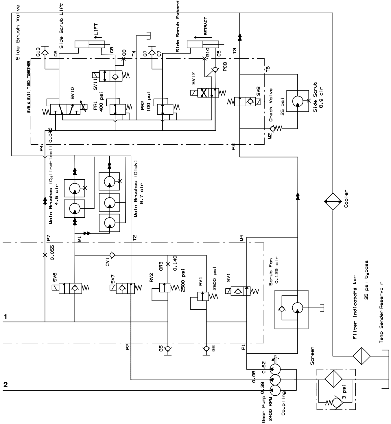
Fig. 52 – Hydraulic Schematic (002283– )
