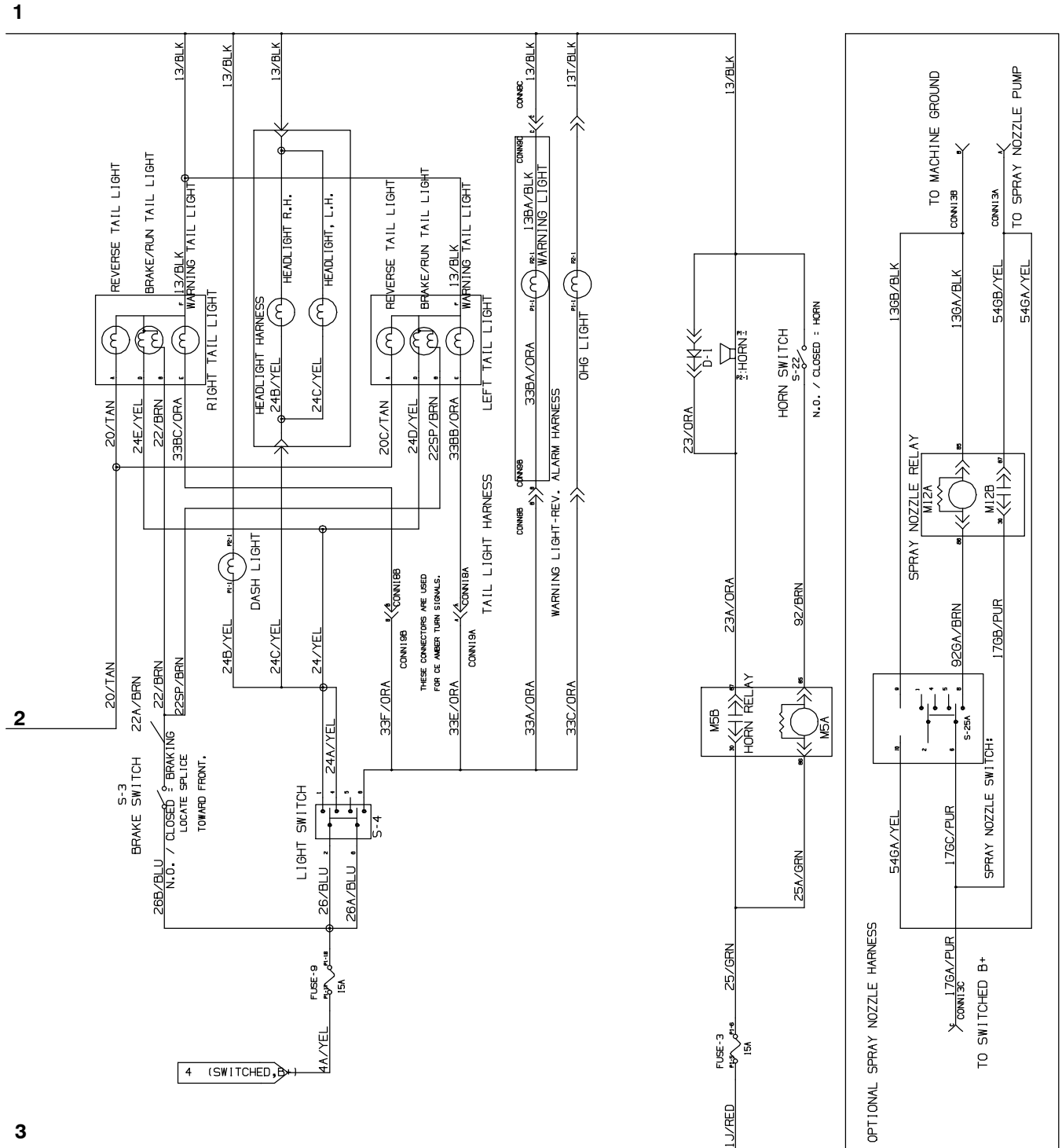
Fig. 63 – Electrical Schematic (001743–
