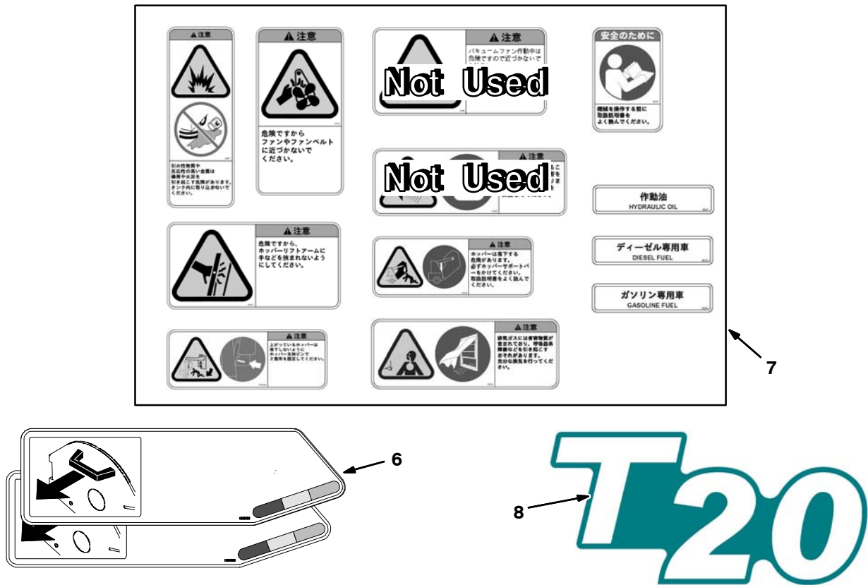
Fig. 68 – Label Group
