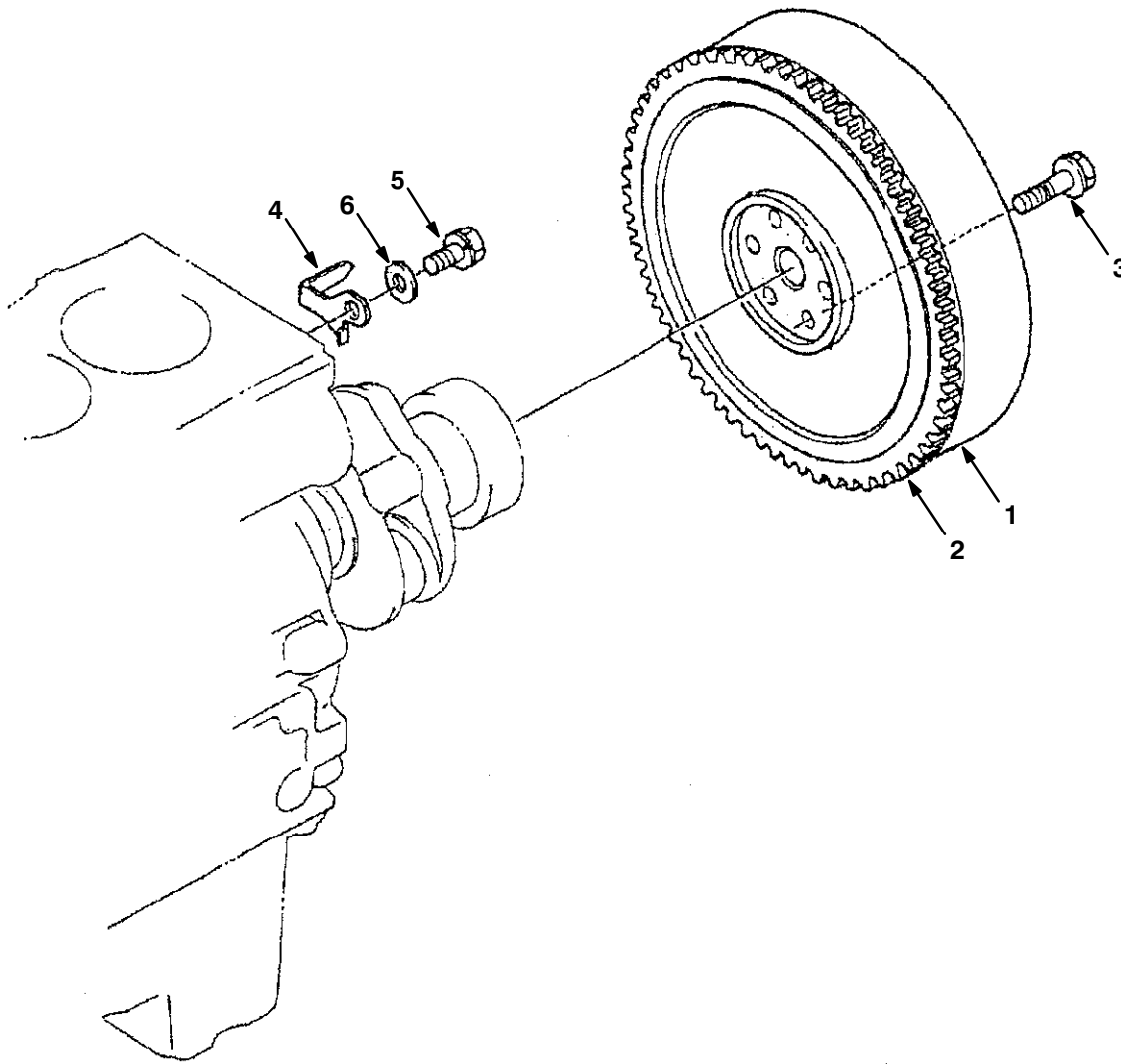
Fig. 13 – Flywheel Group
