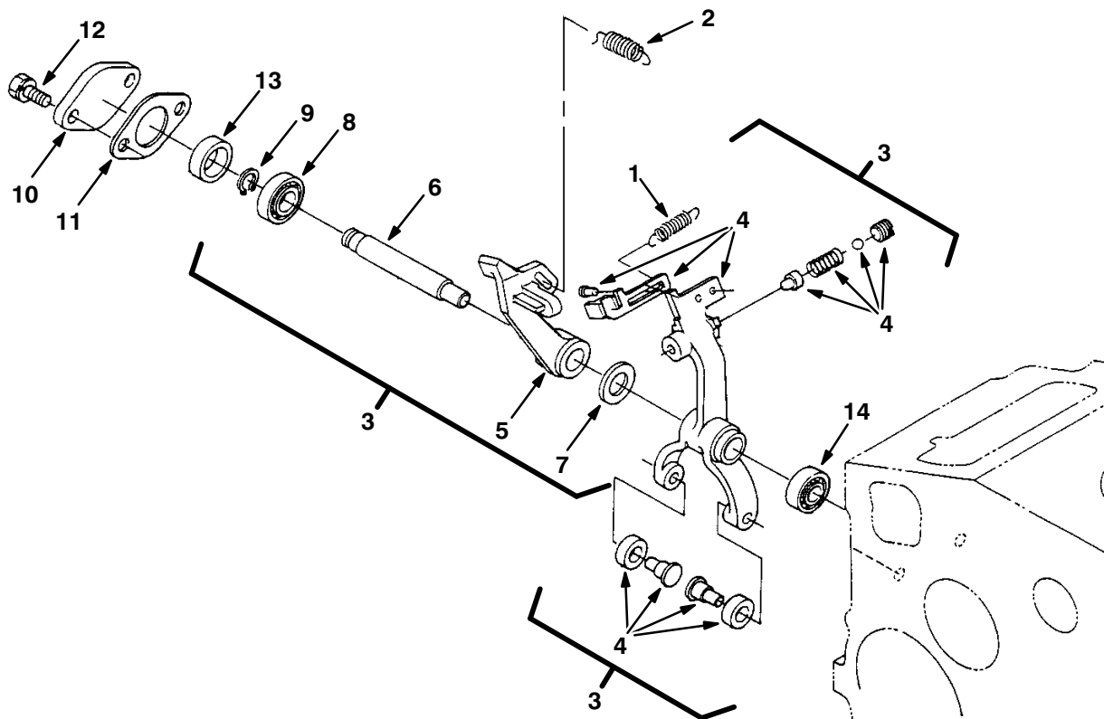
Fig. 20 – Governor Group
