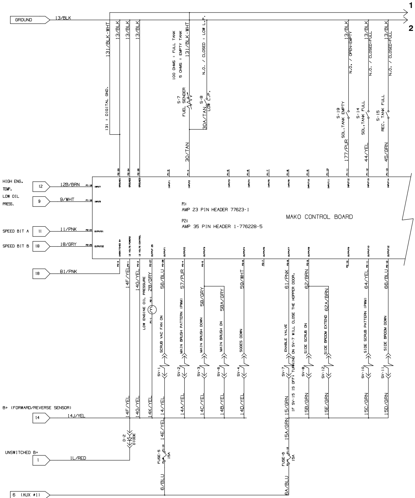
Fig. 63 – Electrical Schematic (001743– )
