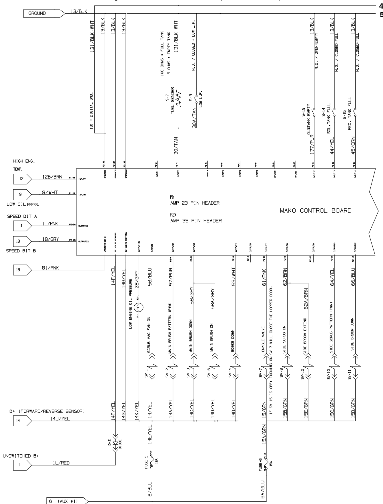
Fig. 62 – Electrical Schematic (000000-001742)
