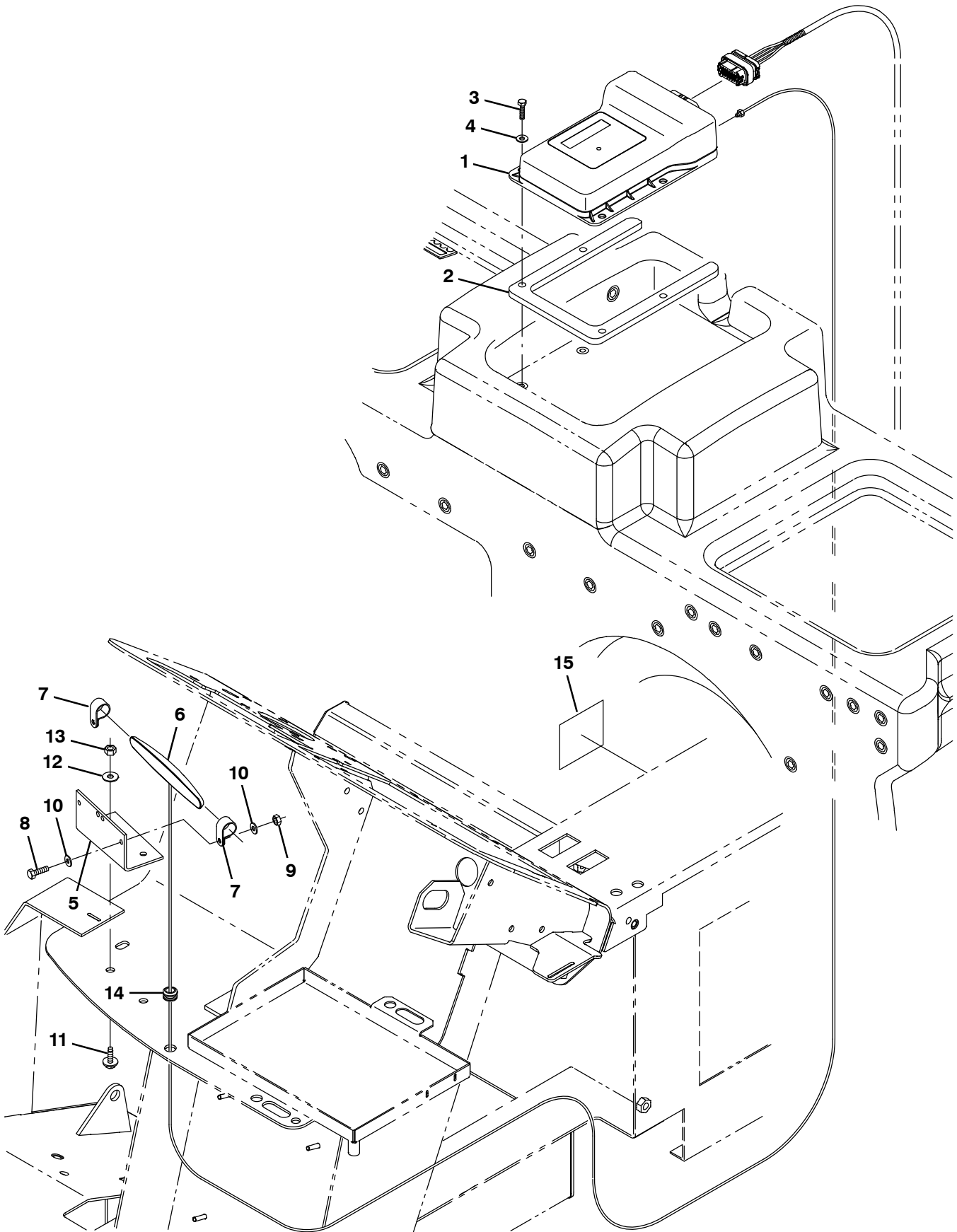
Fig. 36 – Telemetry Group
