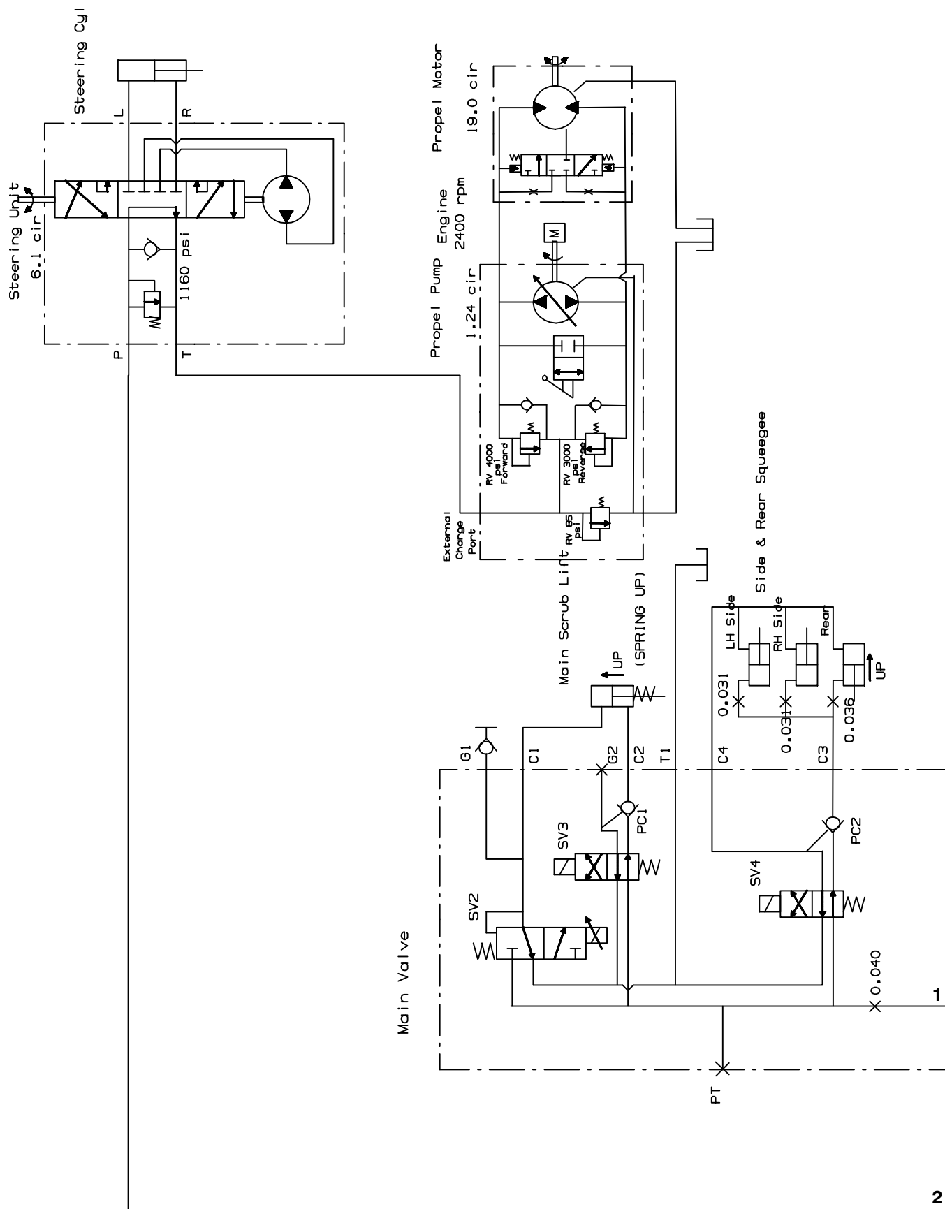
Fig. 52 – Hydraulic Schematic (002283– )
