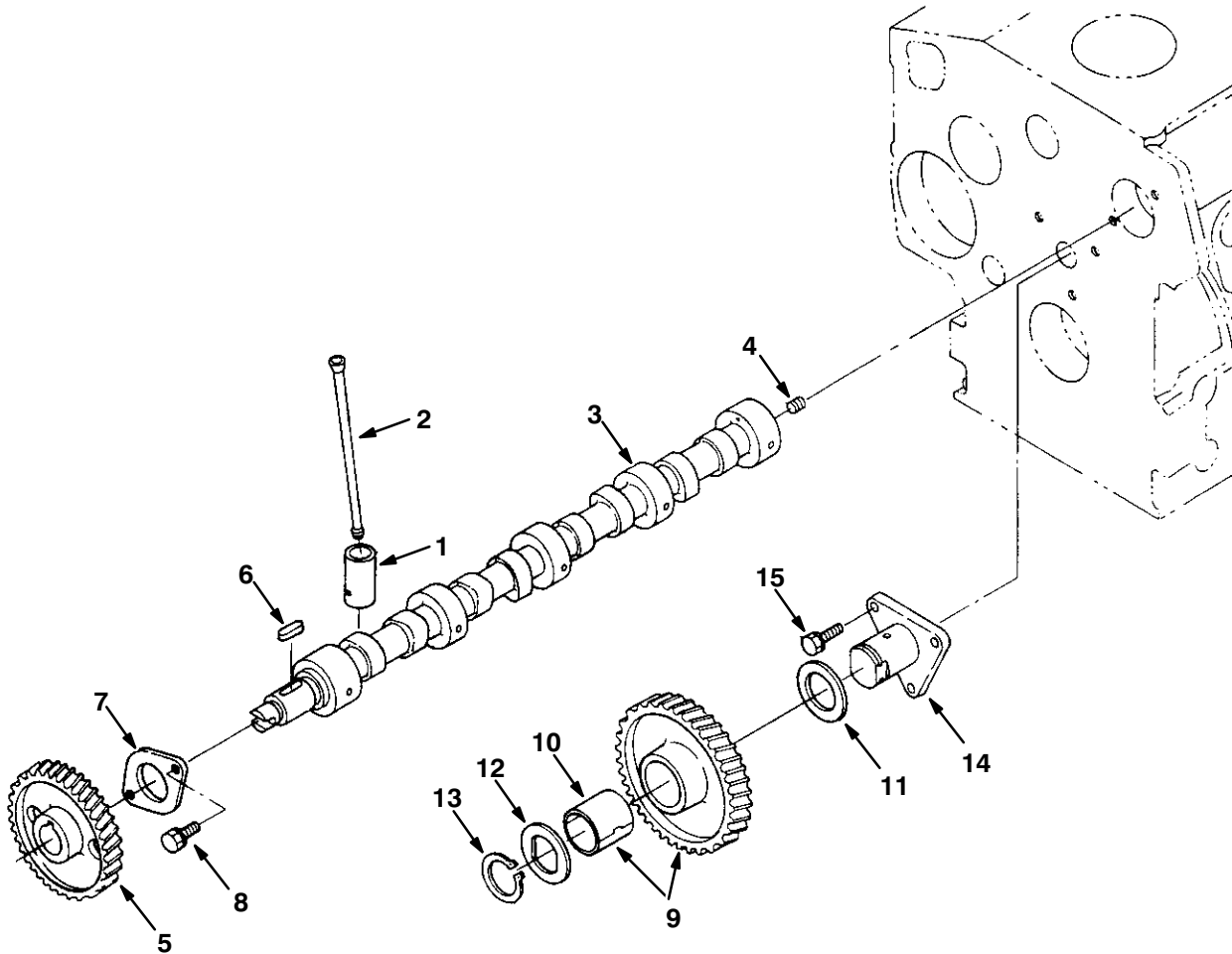
Fig. 11 – Camshaft Group
