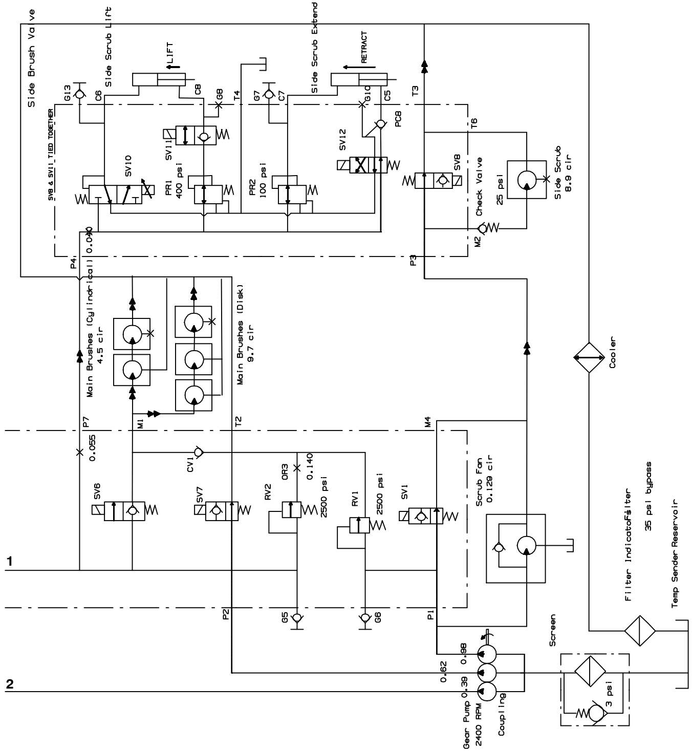
Fig. 51 – Hydraulic Schematic (001504-002282)
