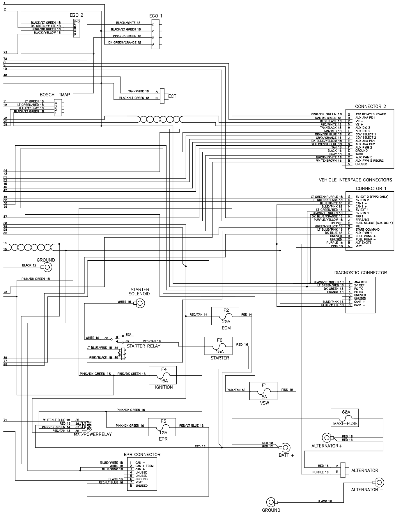
Fig. 86 - Electrical Schematic, LPG Engine Harness, GM (000000-005699) (2 of 2)
