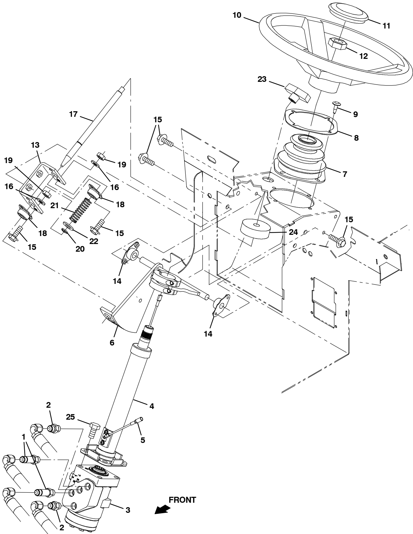
Fig. 18 - Steering Group (002100- )
