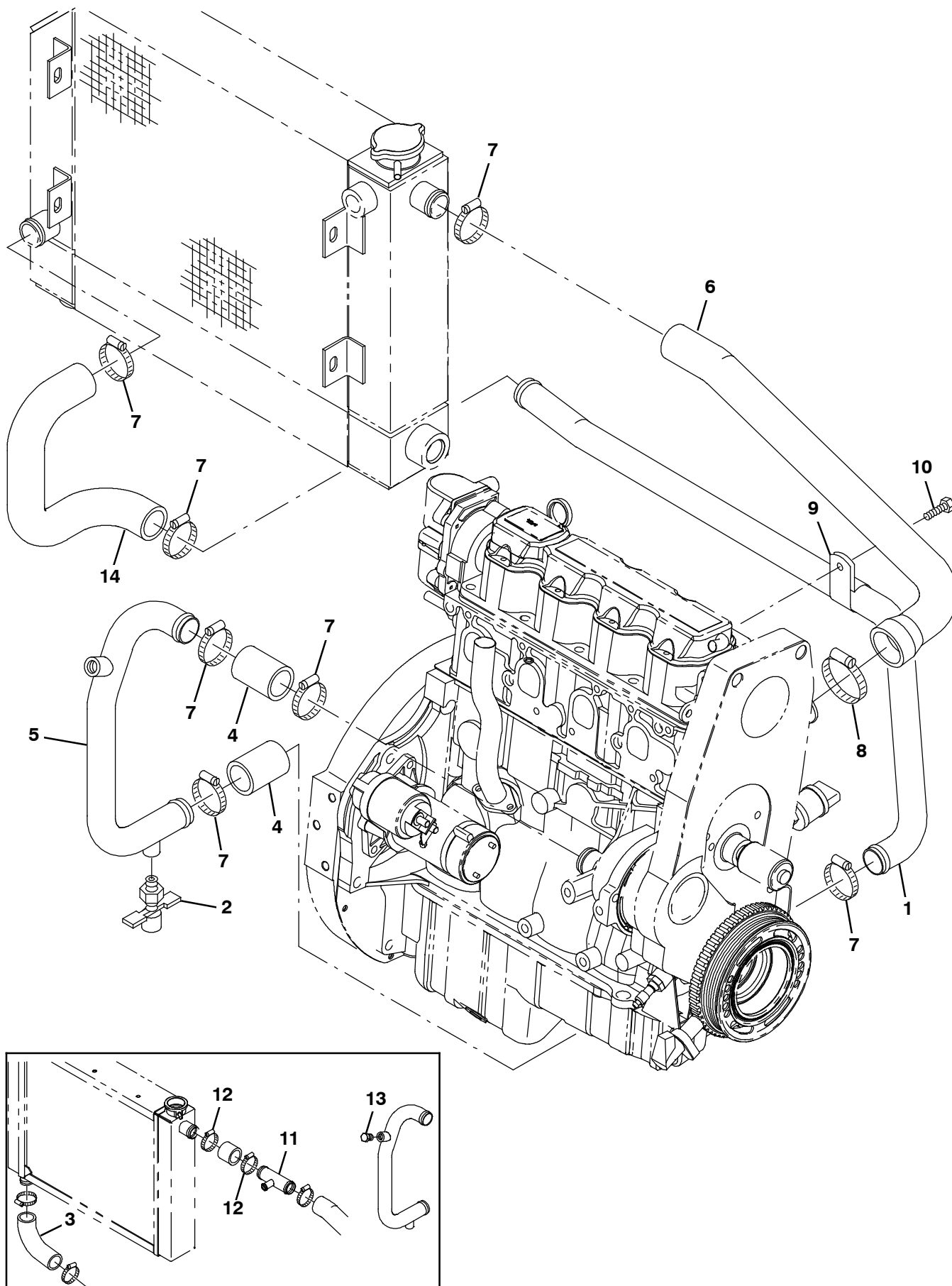
Fig. 41 - Engine Radiator Hoses Group, Gas/LPG (000000-005699)
