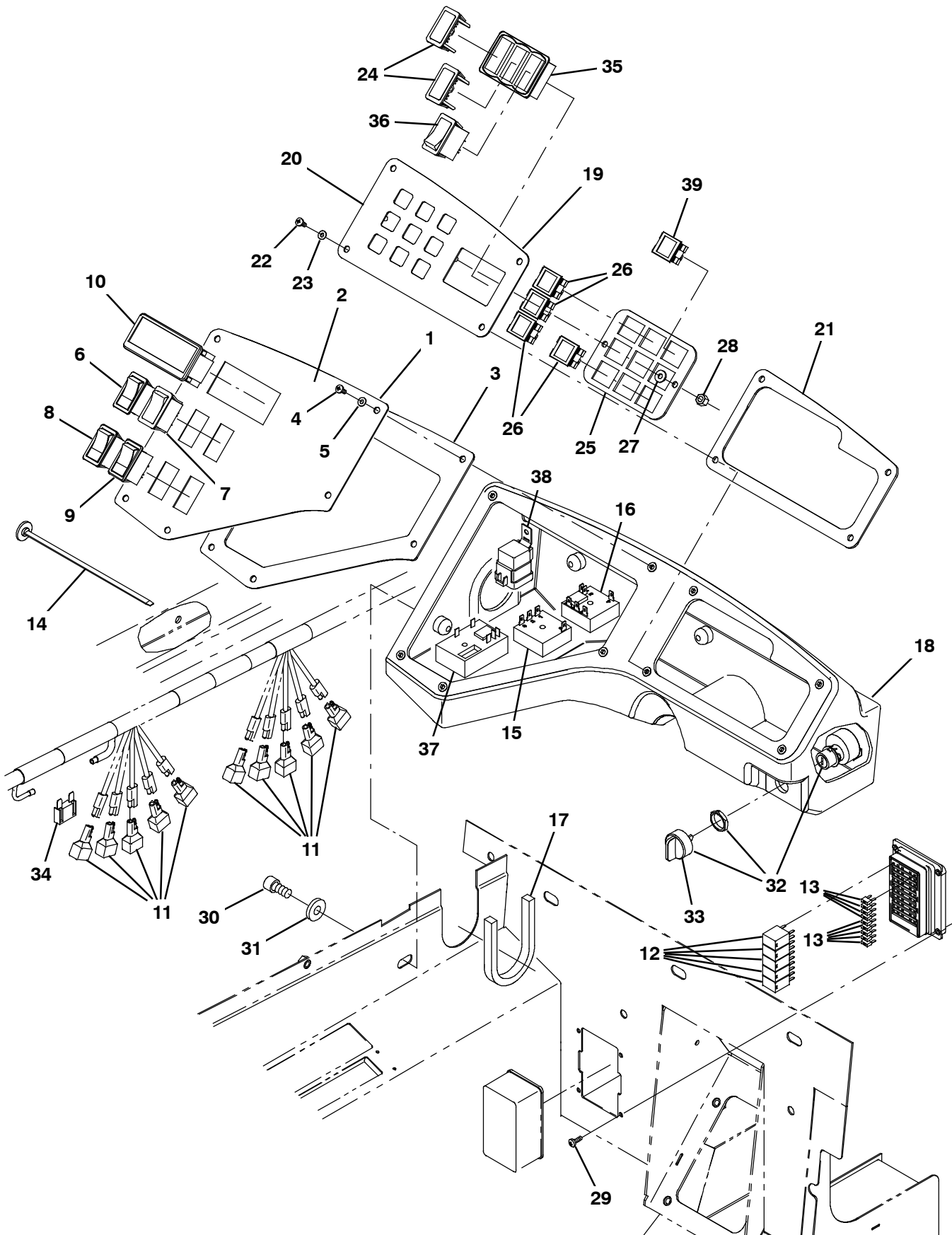
Fig. 15 - Instrument Panel Group, S30
