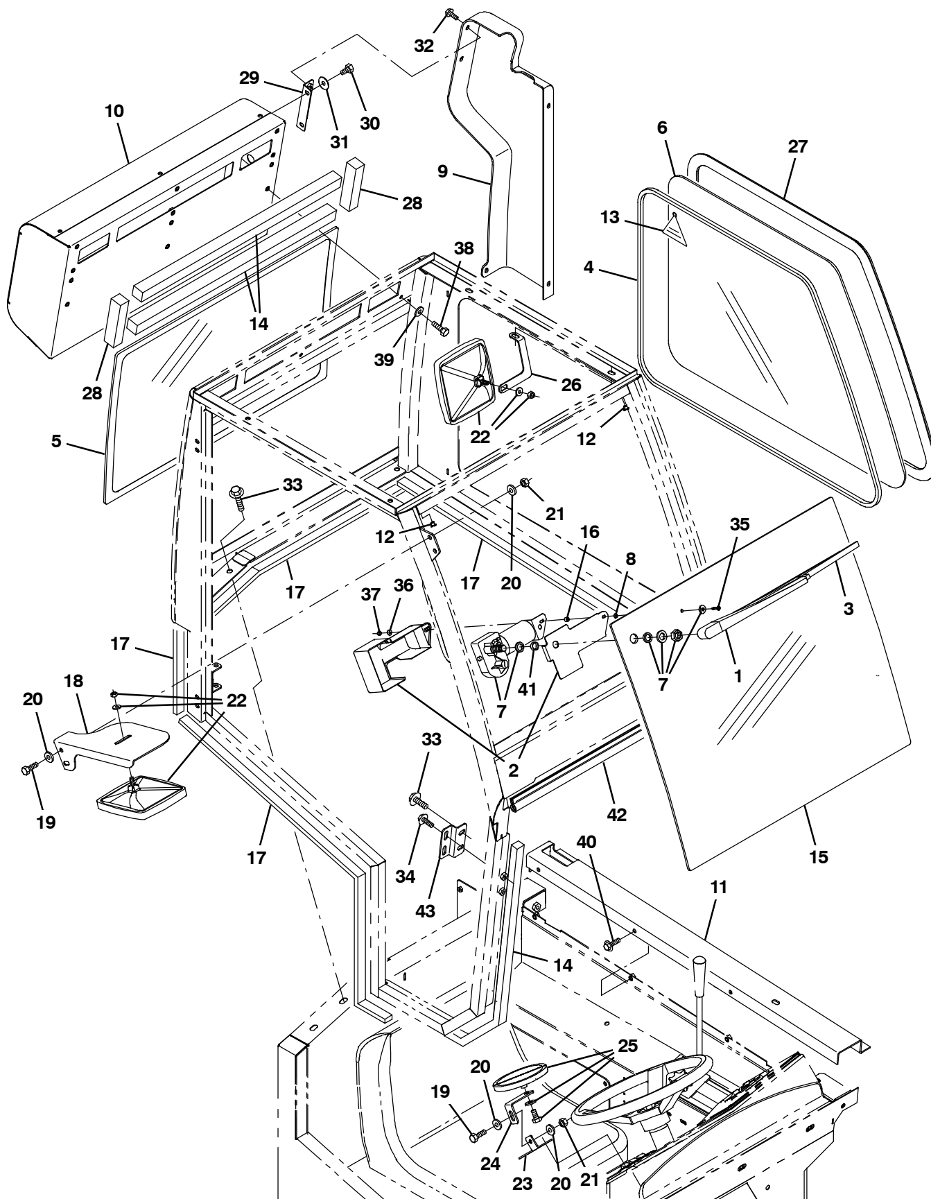
Fig. 10 - Cab Group
