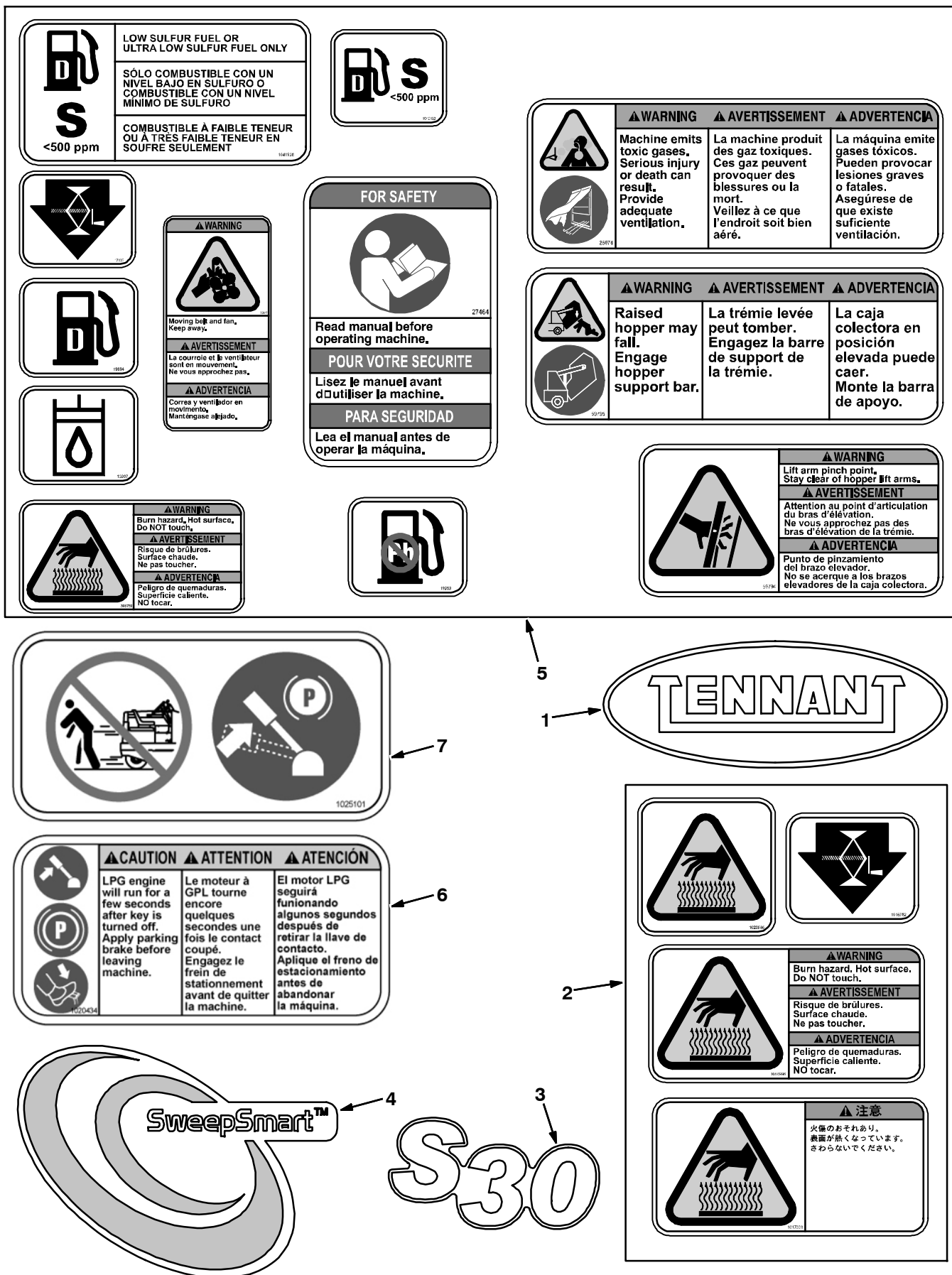
Fig. 89 - Label Group
