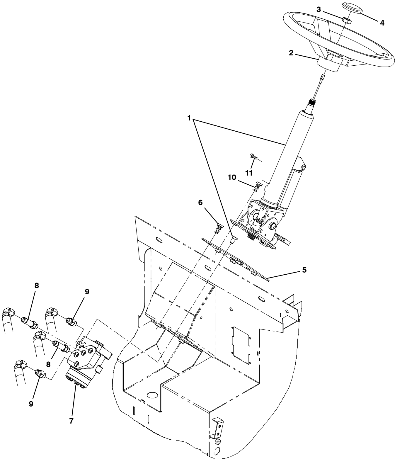
Fig. 17 - Steering Group (000000-002099)
