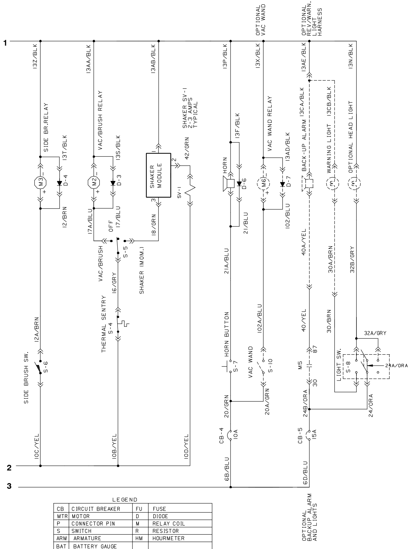
Fig. 31 – Electrical Schematic (000000-002014)
