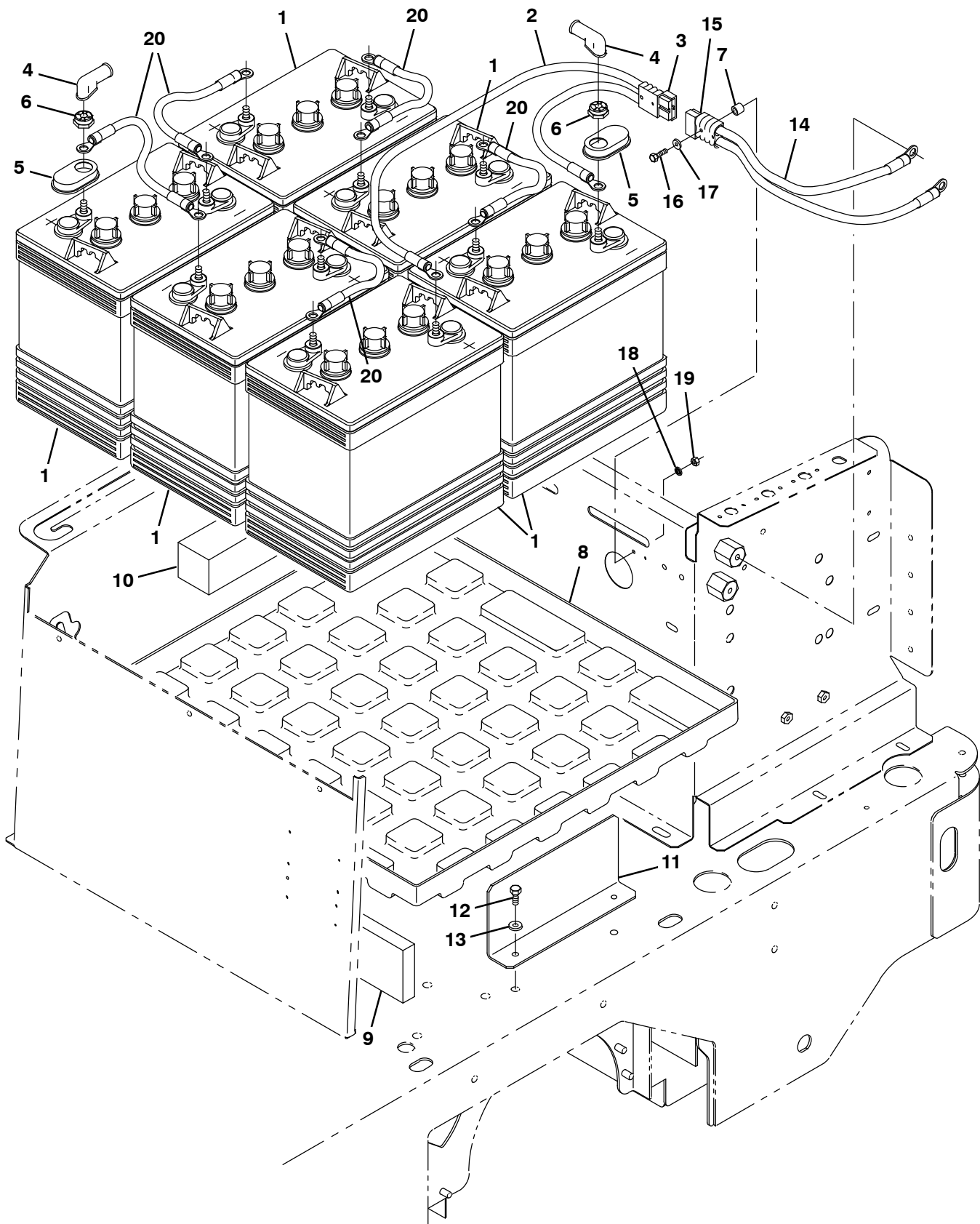
Fig. 30 – Battery Group
