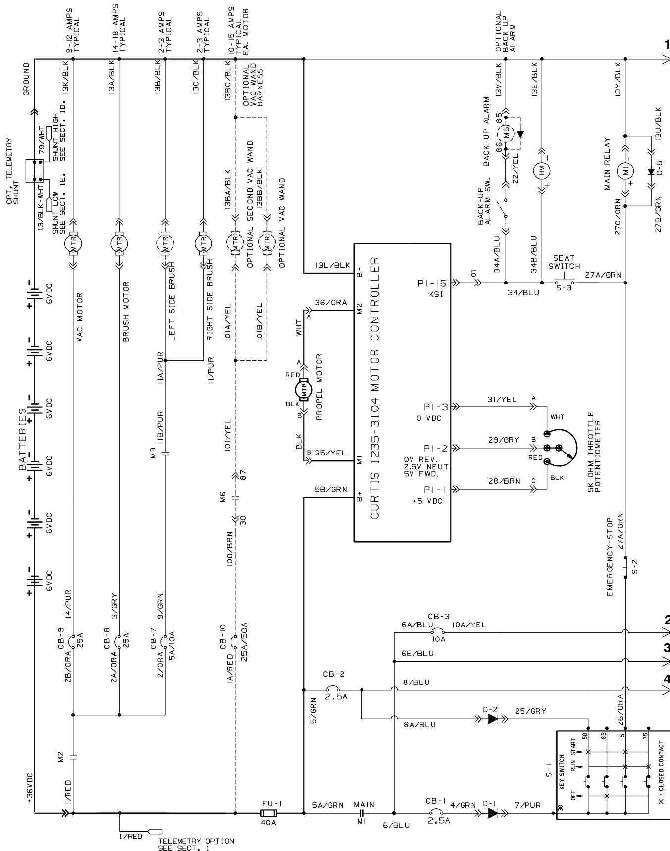
Fig. 33 - Electrical Schematic (005104- )
