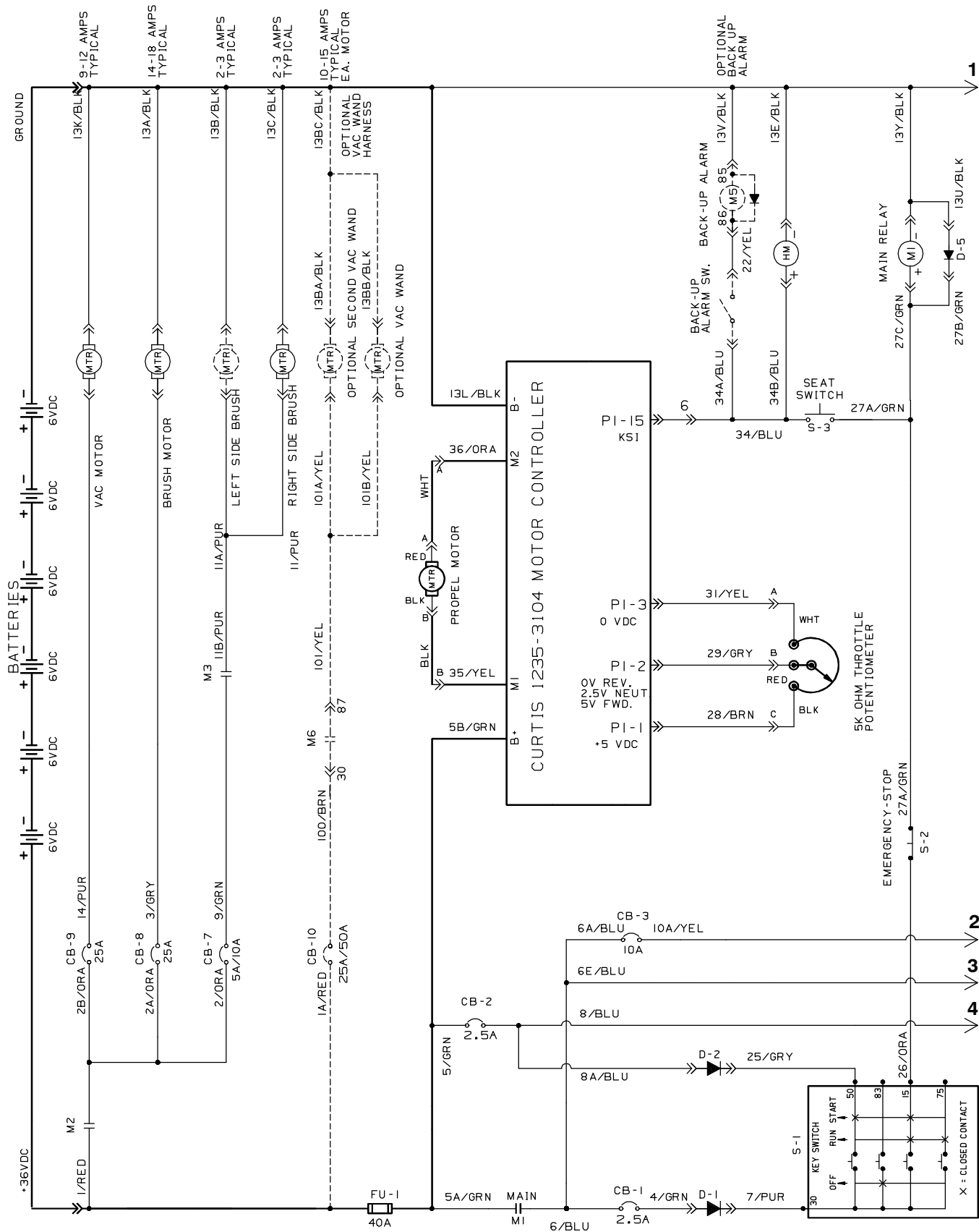
Fig. 32 – Electrical Schematic (002015–005103)
