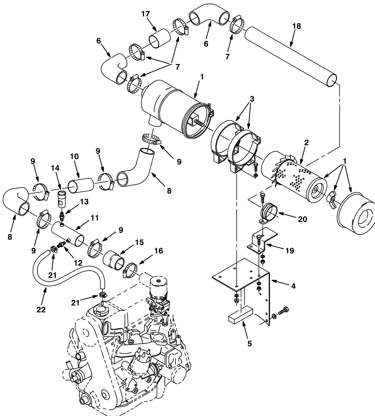
Fig. 40 – Air Cleaner Group, Gasoline
