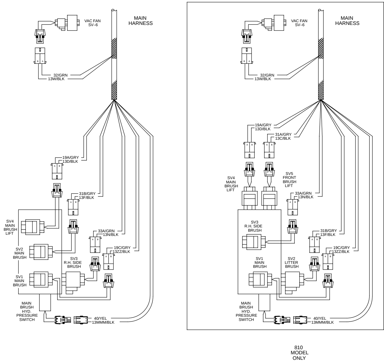
Fi 88 Wire Harnesses Group For machines serial number 1700 and above
