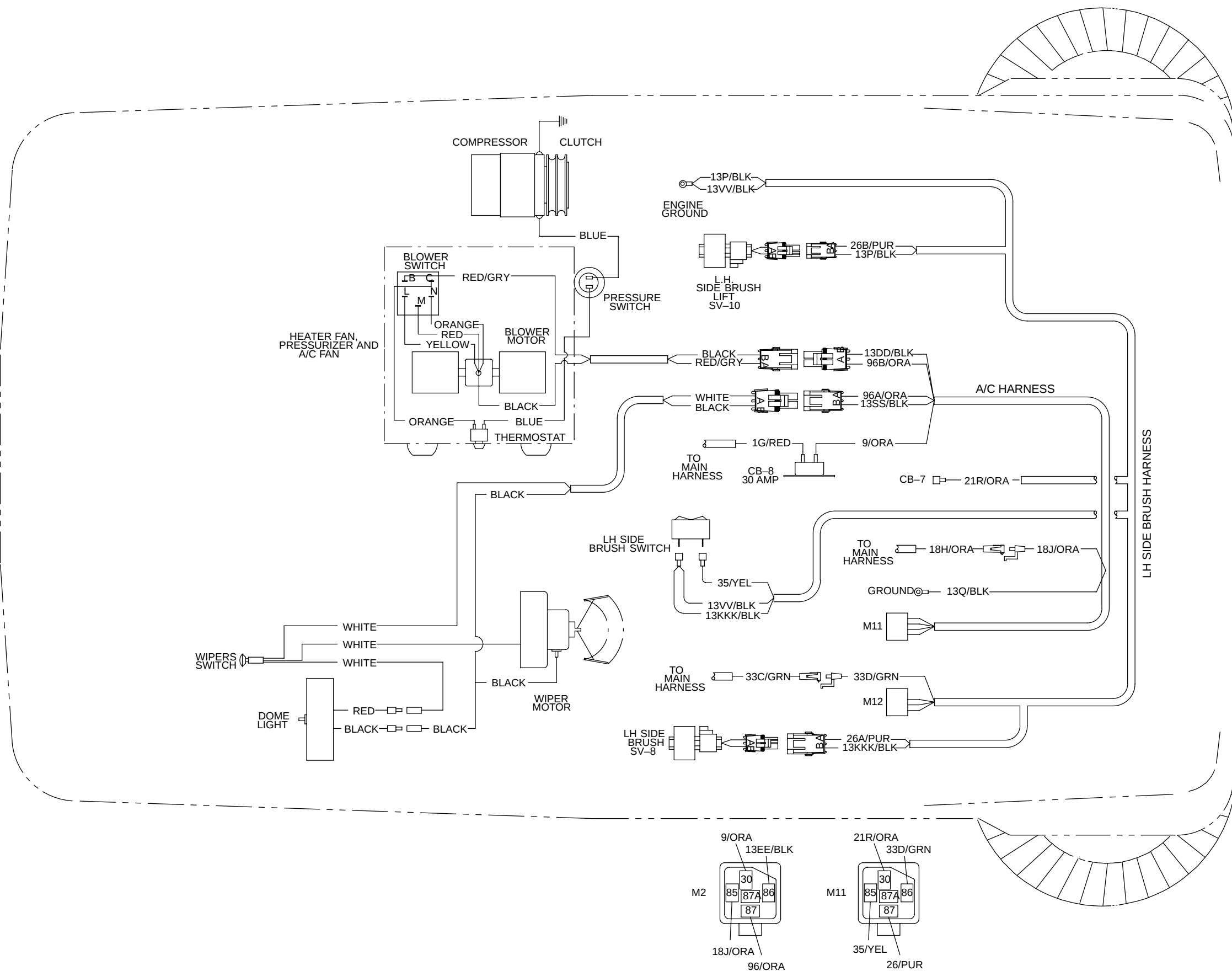
Fi 87 Wire Harnesses Group For machines below serial number 1700
