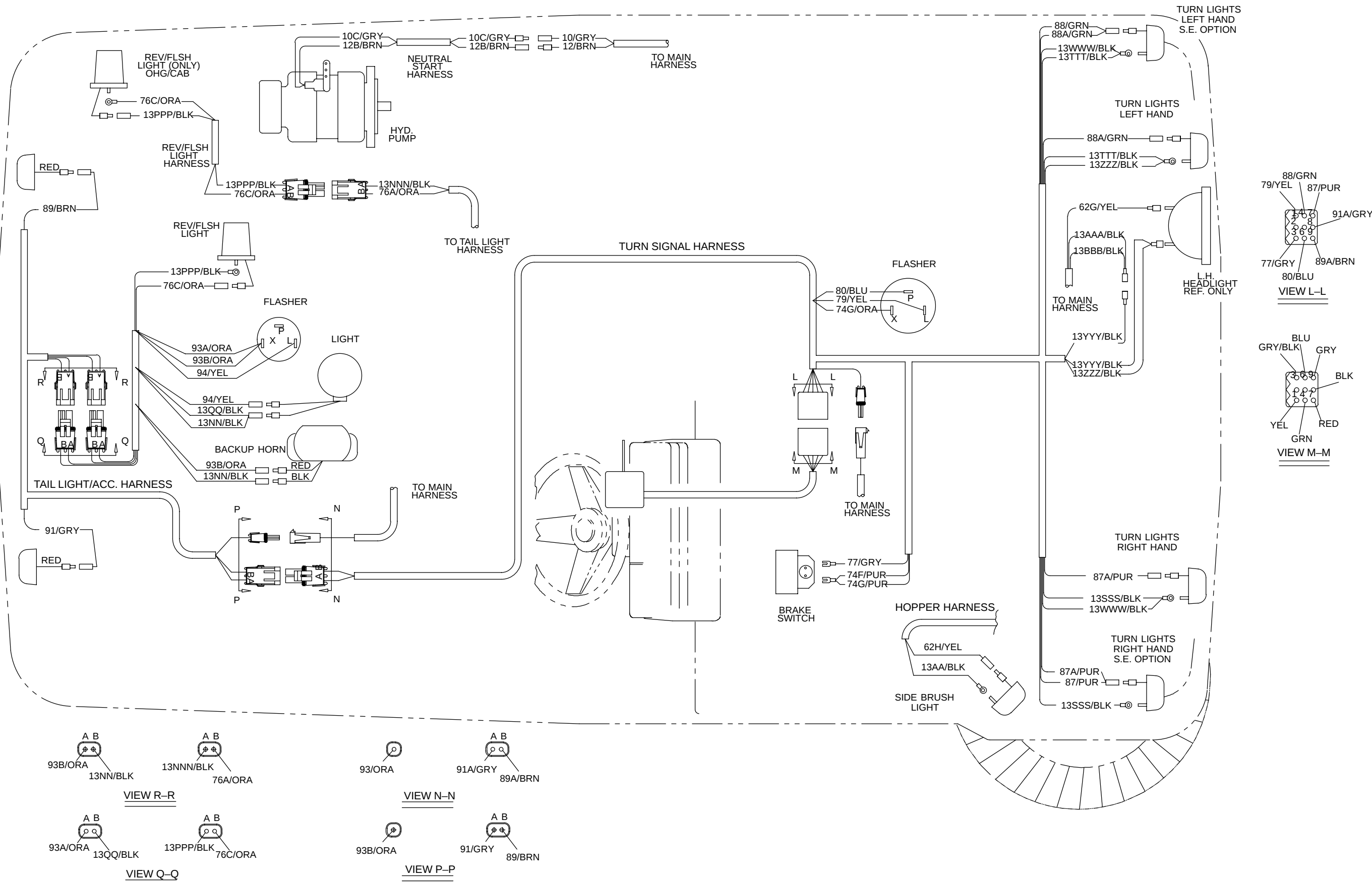
Fi 87 Wire Harnesses Group For machines below serial number 1700
