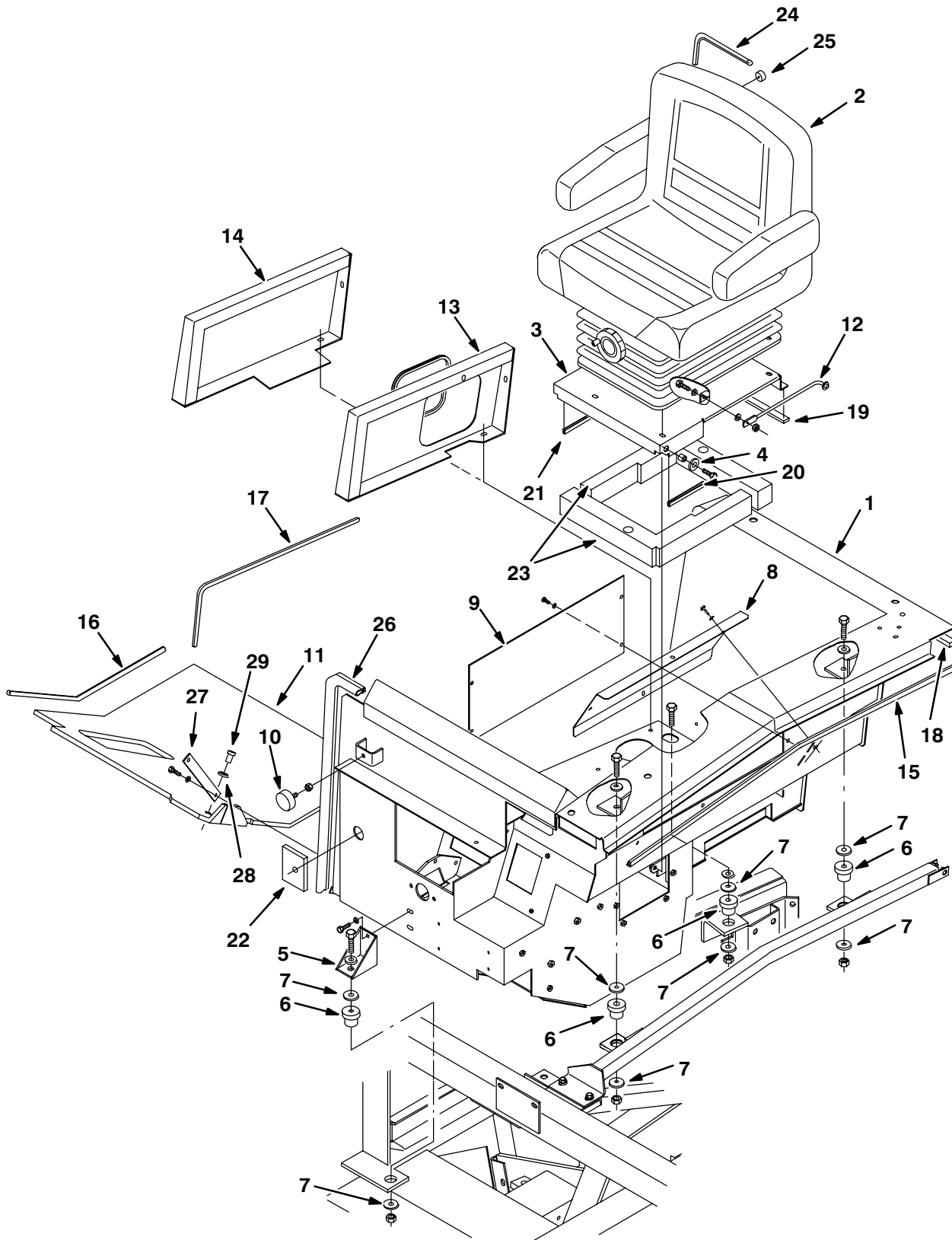
Fig. 9 – Operator Station Group
