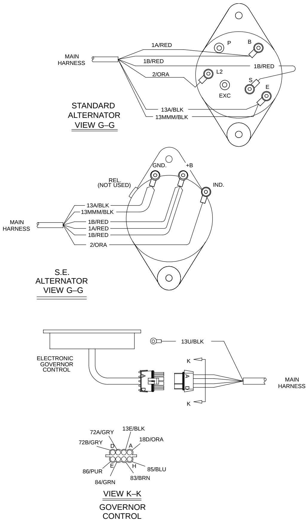
Fig. 87 – Wire Harnesses Group (For machines below serial number 1700)
