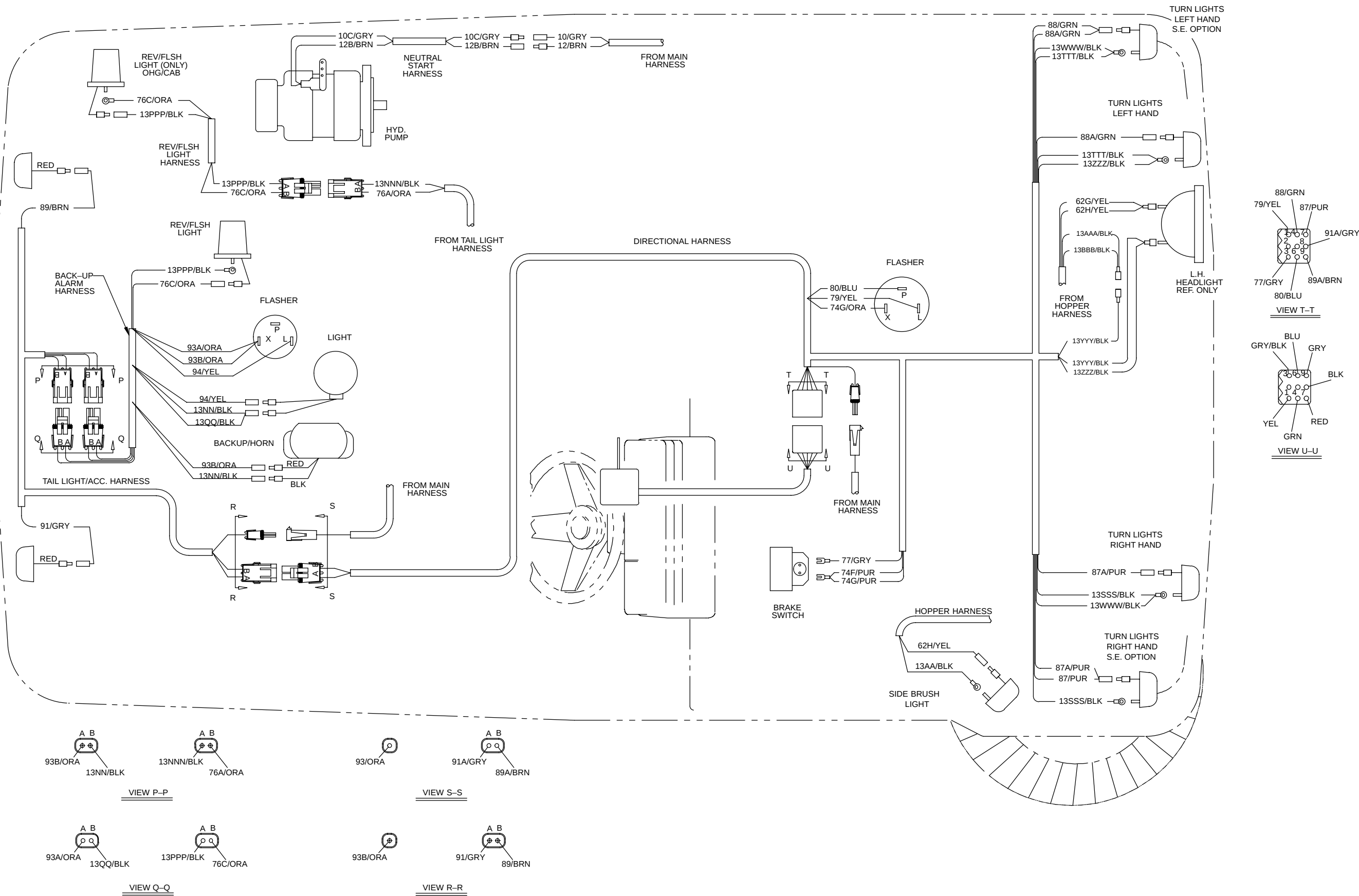
Fi 88 Wire Harnesses Group For machines serial number 1700 and above
