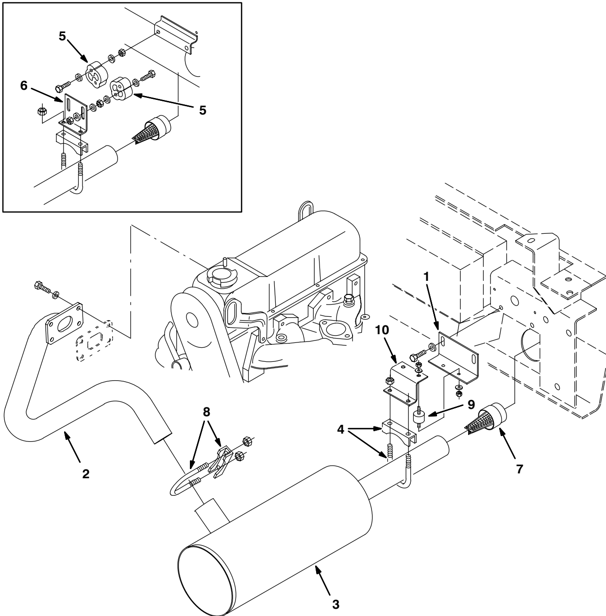
Fig. 46 – Muffler Group
