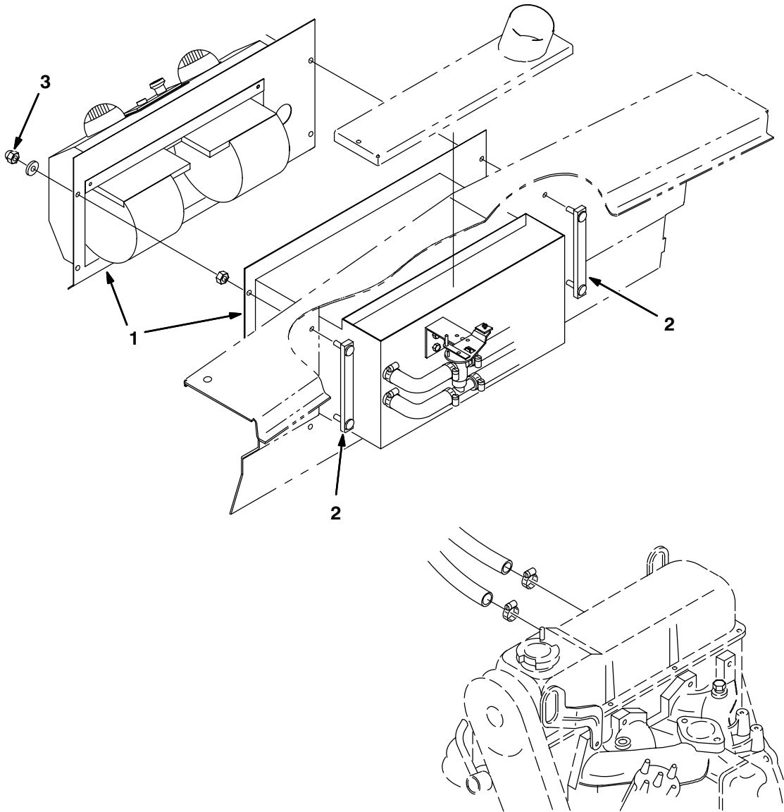
Fig. 32 – Heater/Pressurizer Assembly
