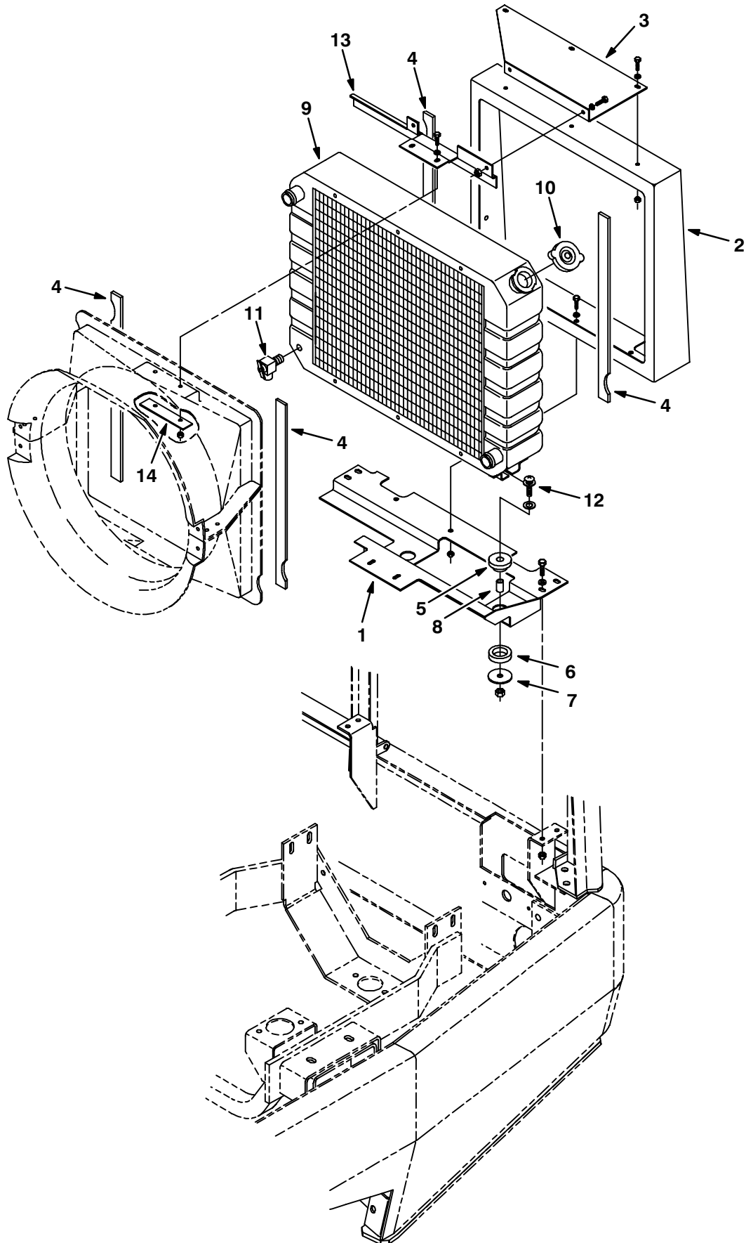
Fig. 51 – Radiator Group
