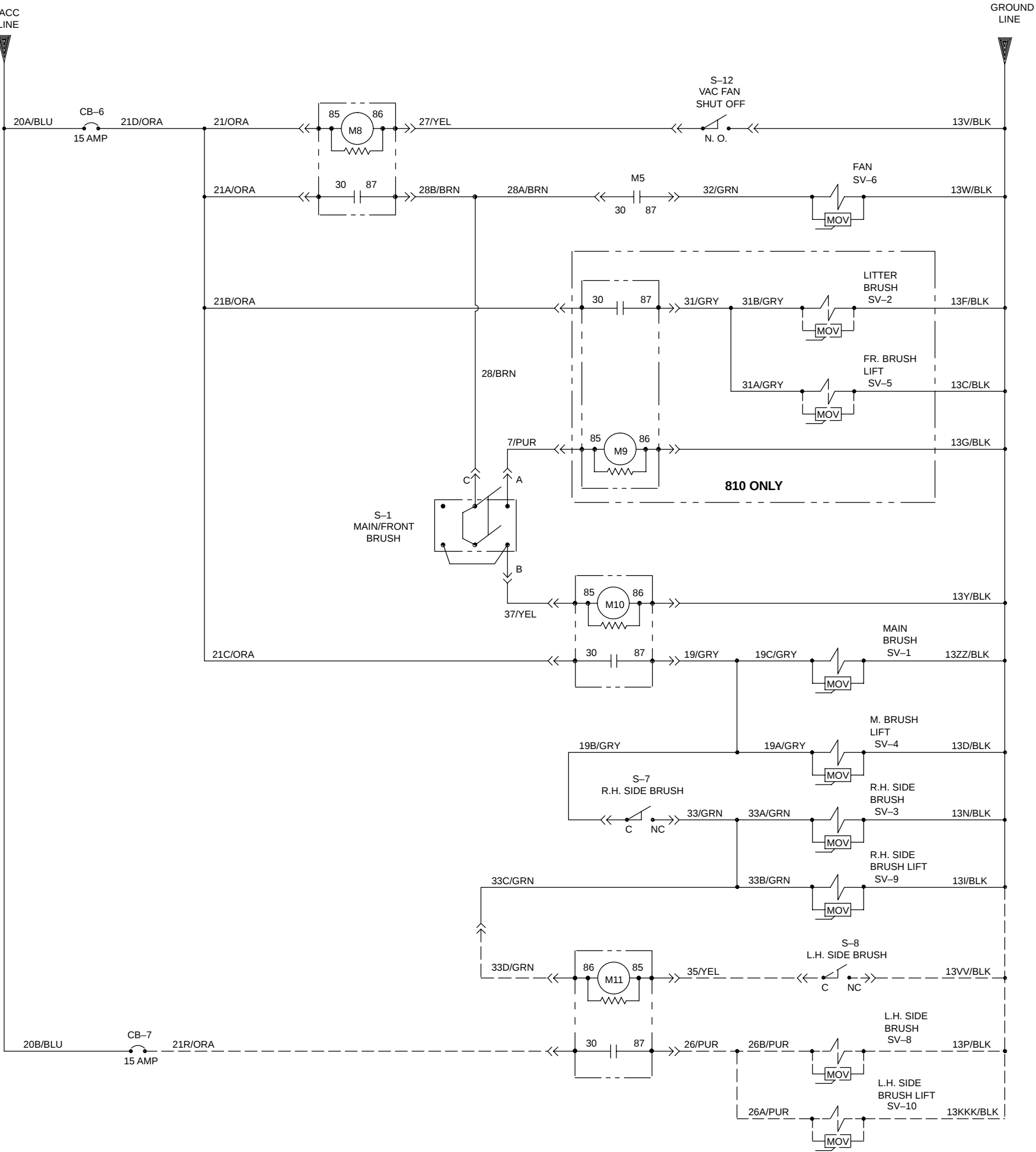
Fi 86 Electrical Schematic For machines serial number 1700 an abo e
