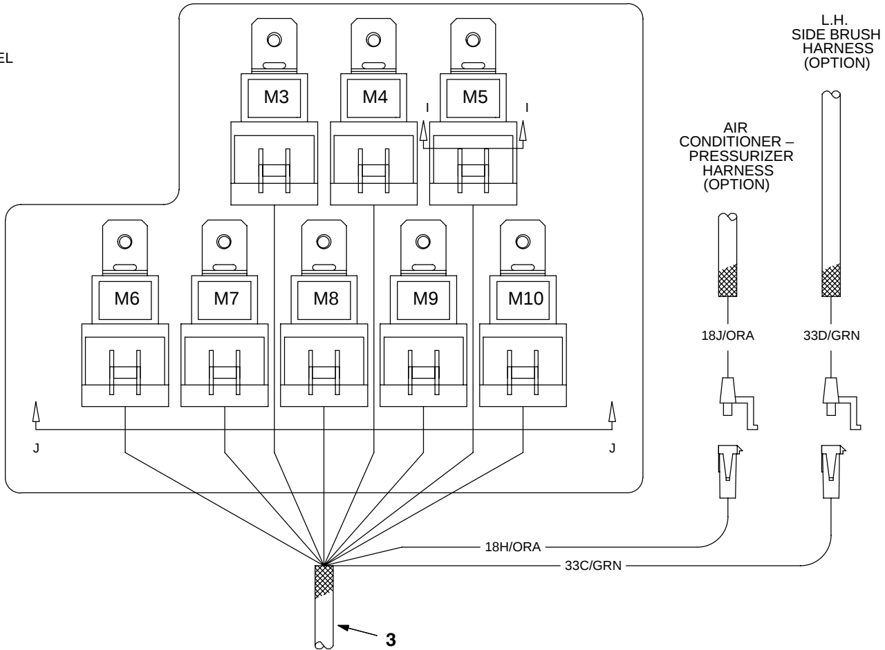
Fi 87 Wire Harnesses Group For machines below serial number 1700
