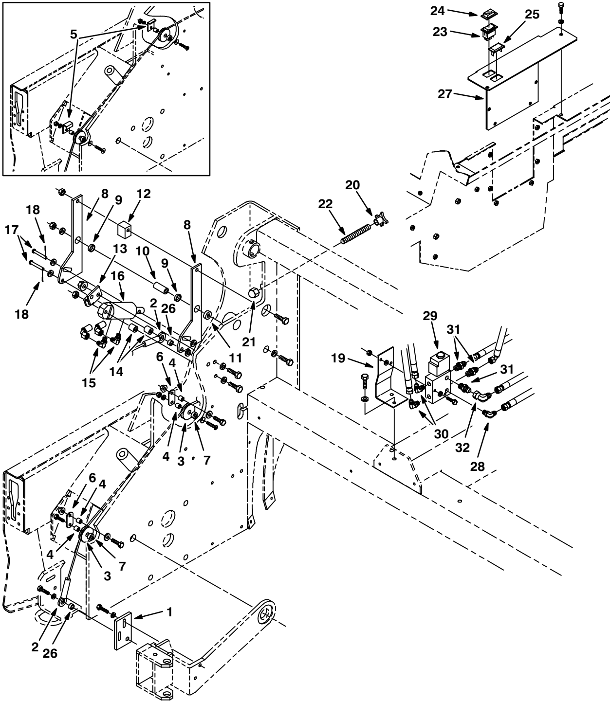
Fig. 74 – Side Brush Lift Group
