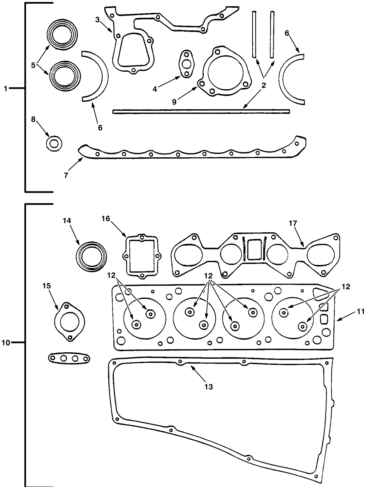
Fig. 2 – Gaskets Group
