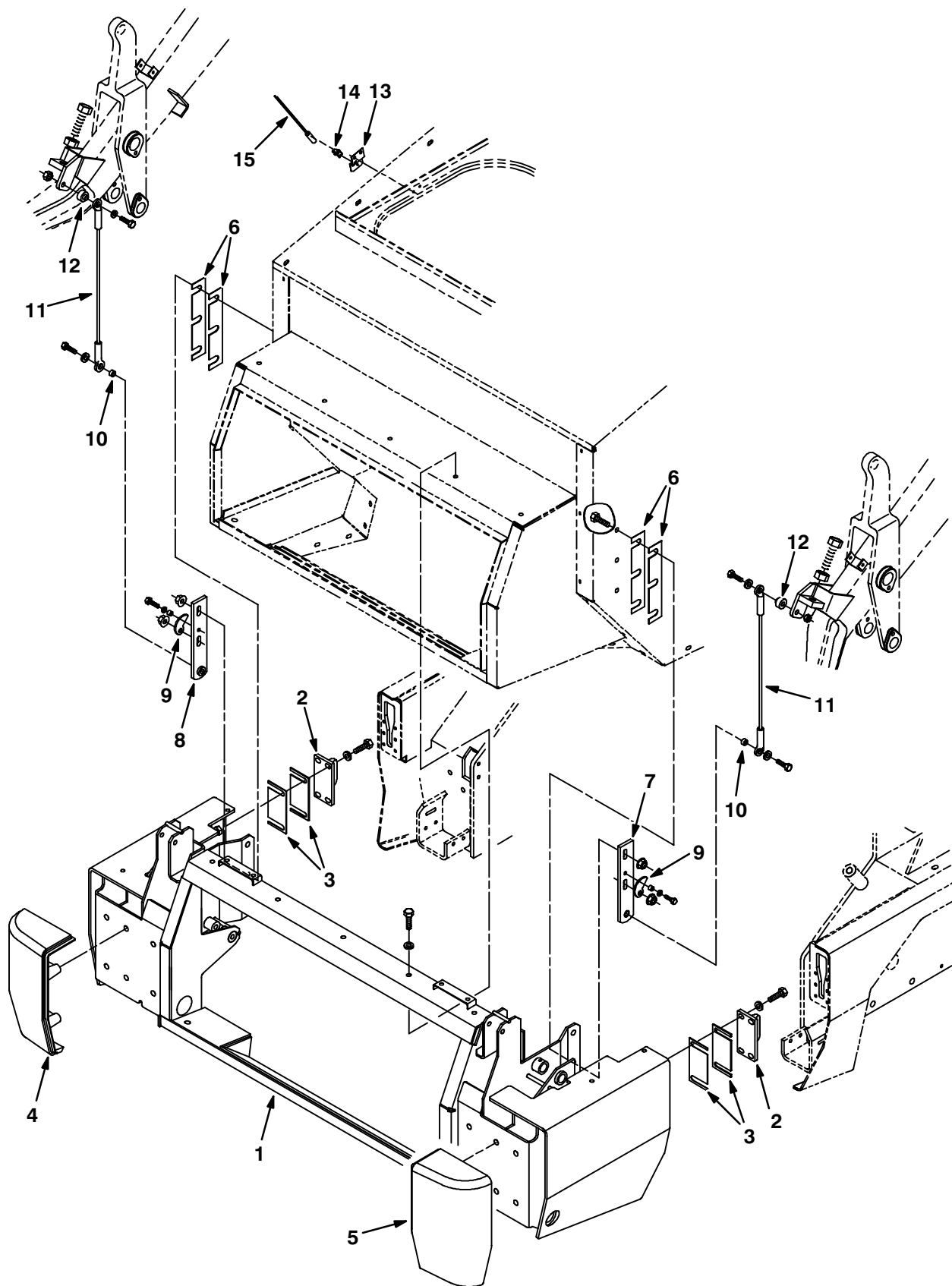
Fig. 25 – Hopper Bumper Group
