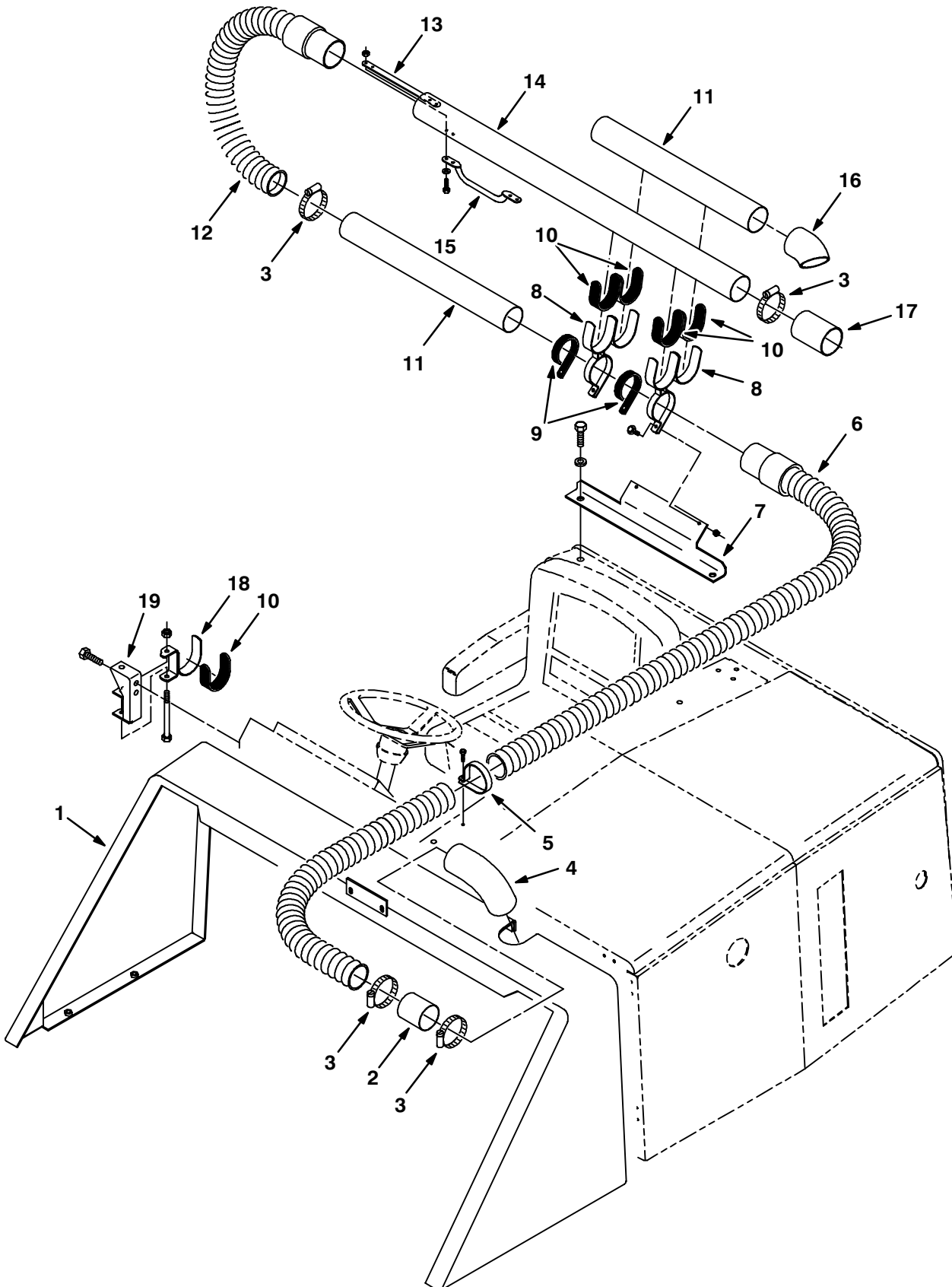
Fig. 12 – Blower Group
