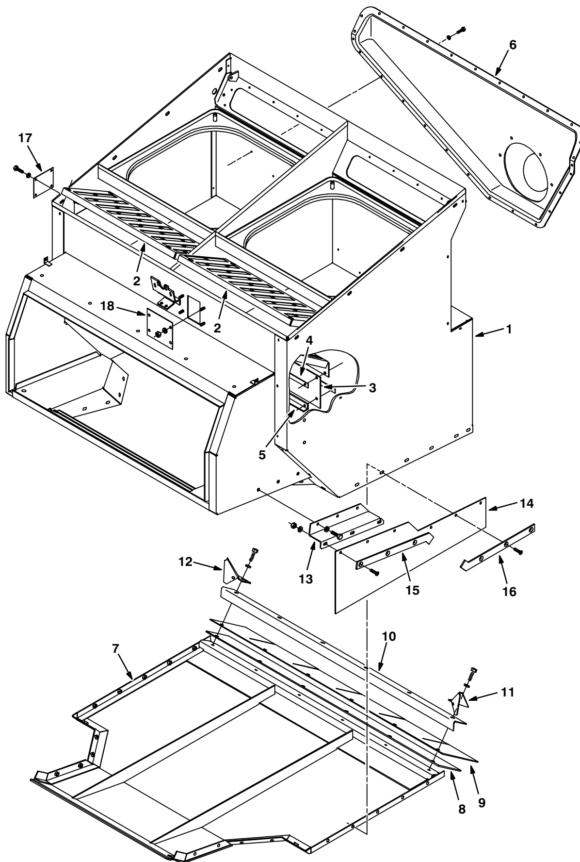
Fig. 19 – Hopper Group
