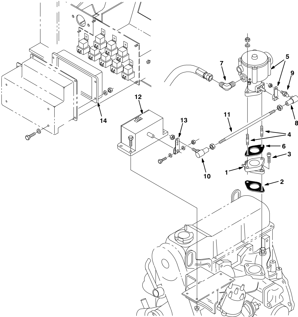
Fig. 36 – Carburetor and Governor Group, LPG
