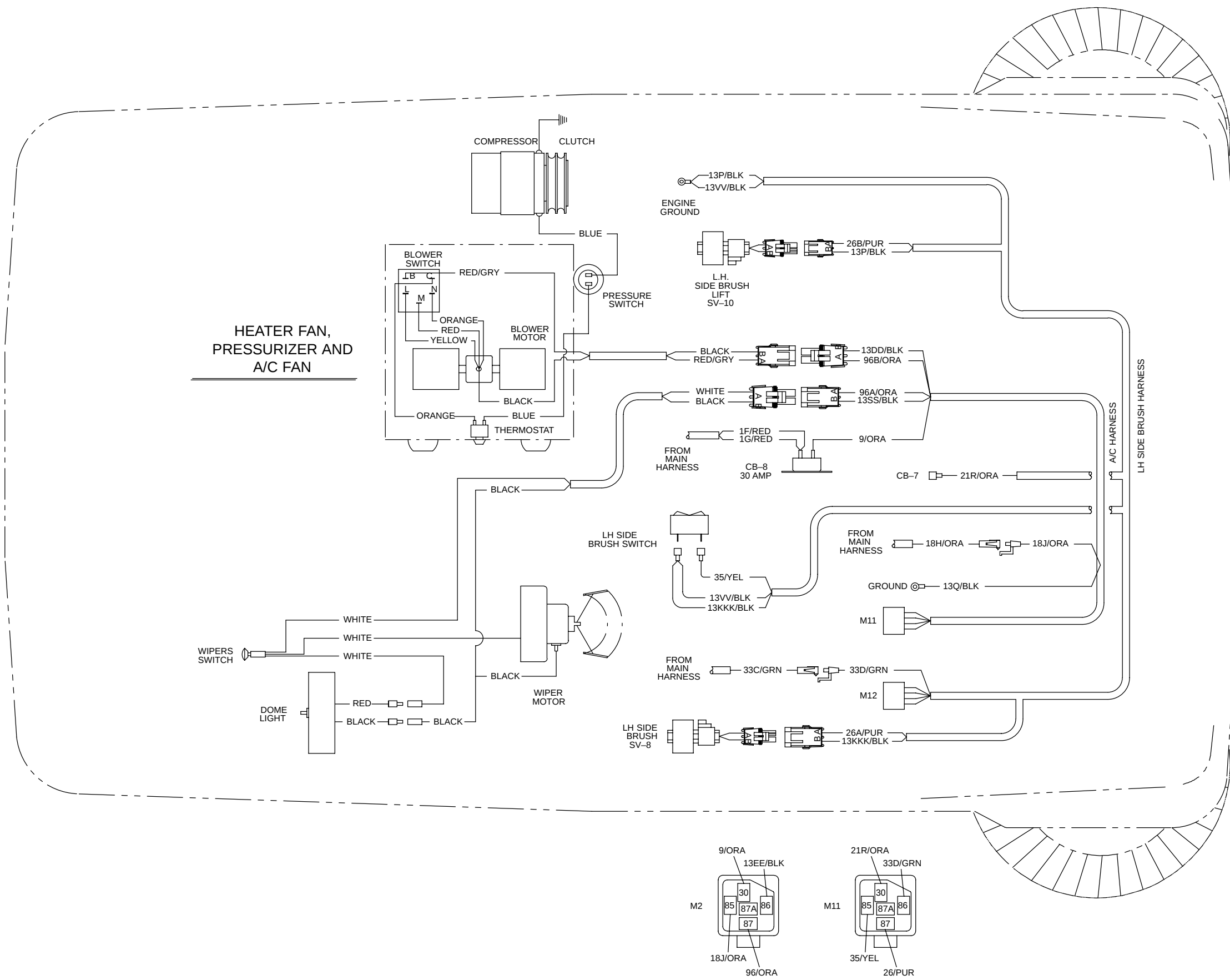
Fi 88 Wire Harnesses Group For machines serial number 1700 and above
