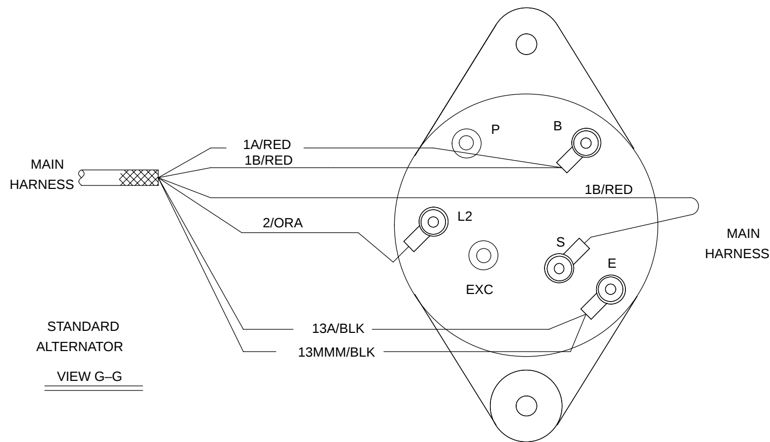
Fi 88 Wire Harnesses Group For machines serial number 1700 and above
