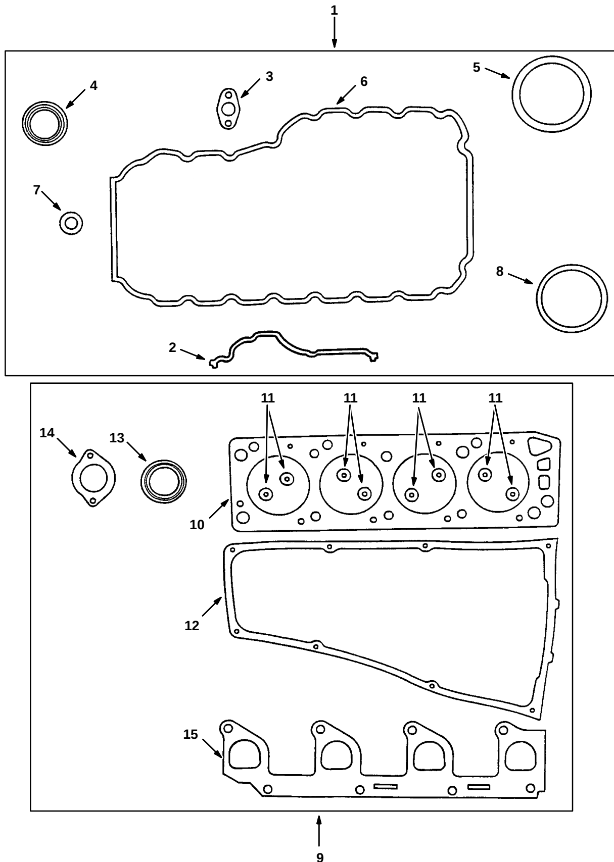
Fig. 2 – Gaskets Group
