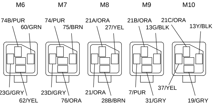
VIEW J-J
