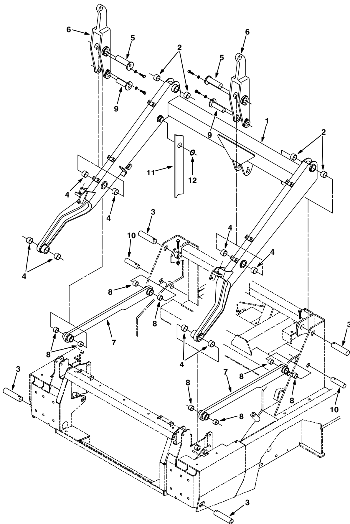
Fig. 15 – Hopper Lift Arms Group
