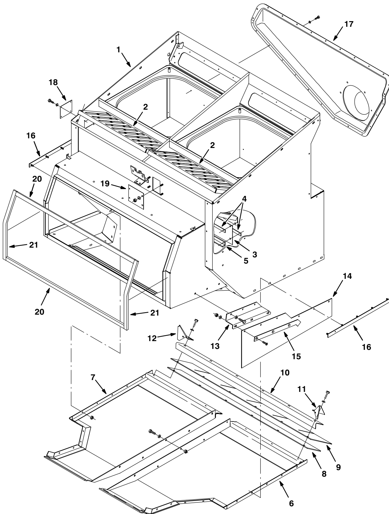
Fig. 20 – Hopper Group
