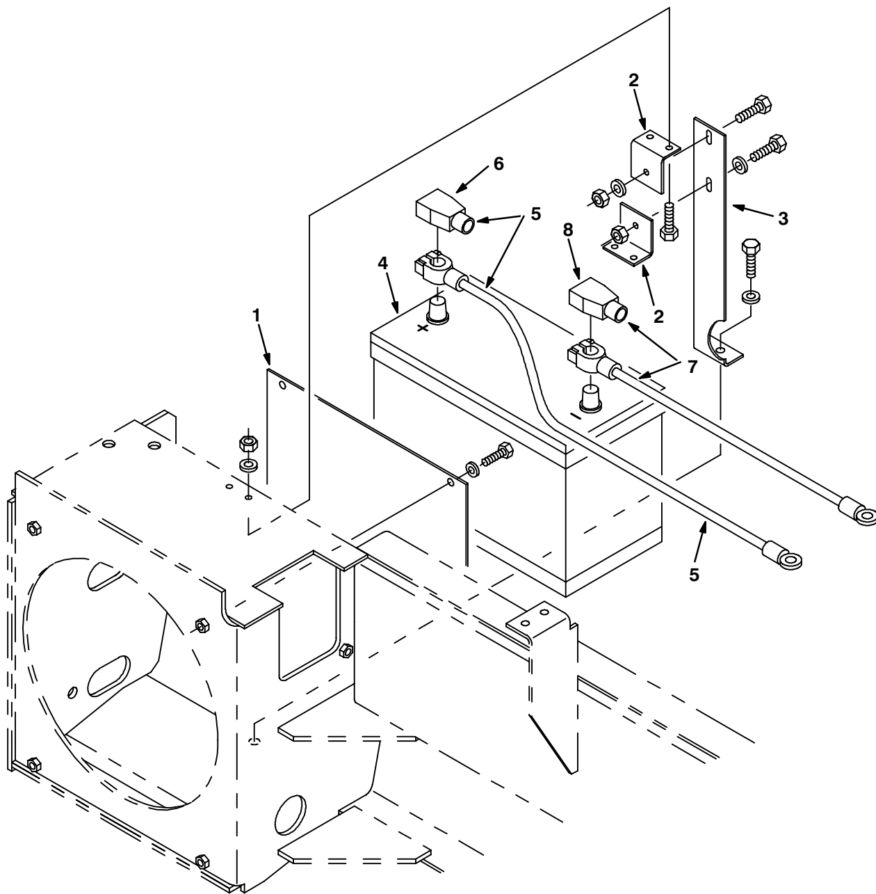
Fig. 41 – Battery Group
