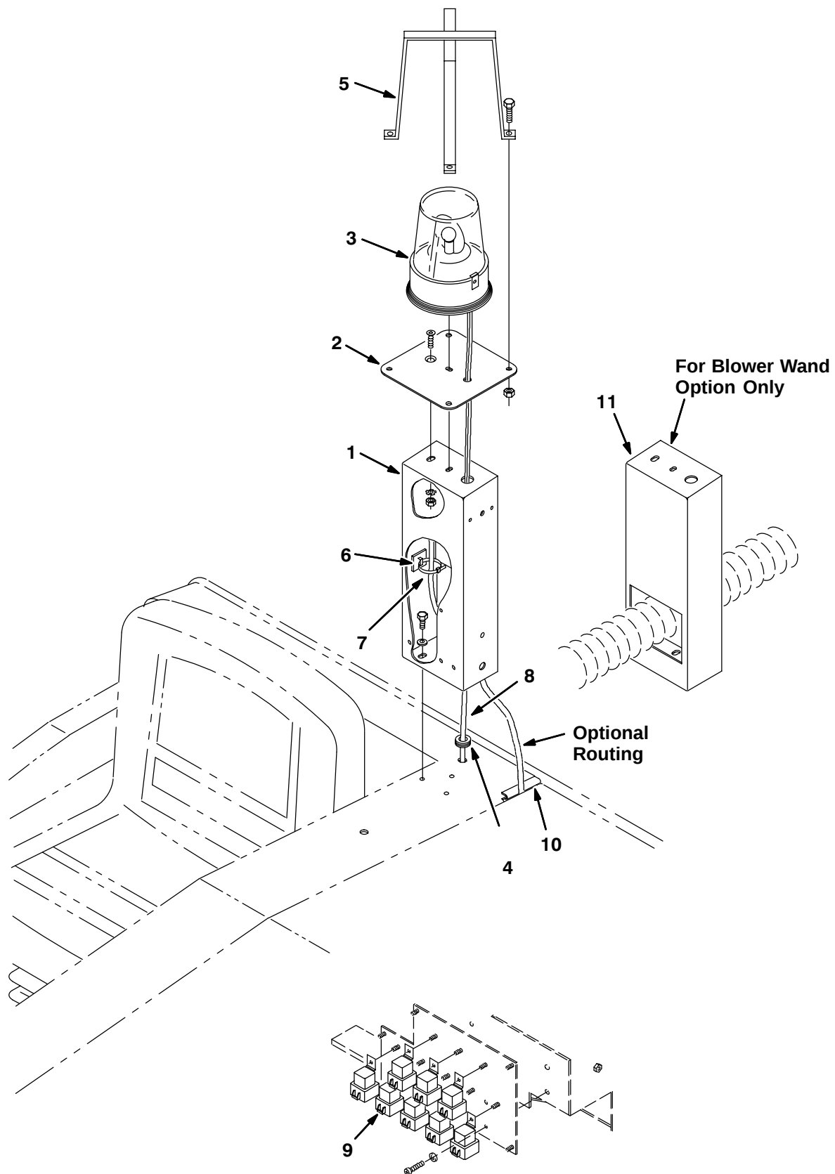
Fig. 6 – Revolving Light Kit, Low
