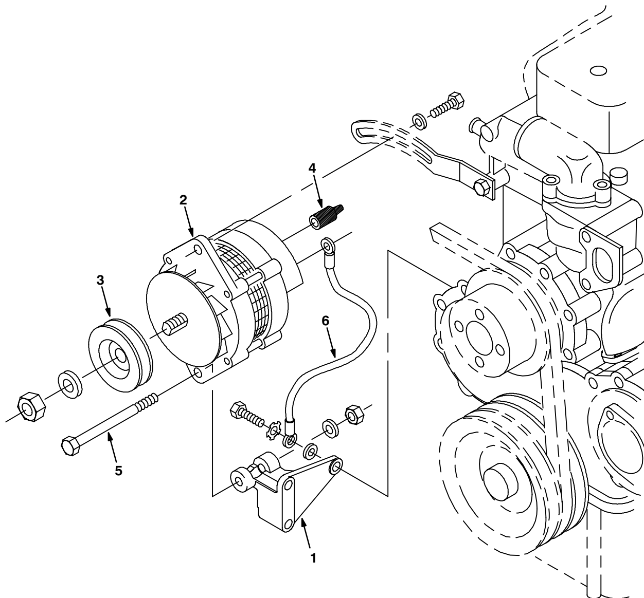
Fig. 30 – Alternator Group
