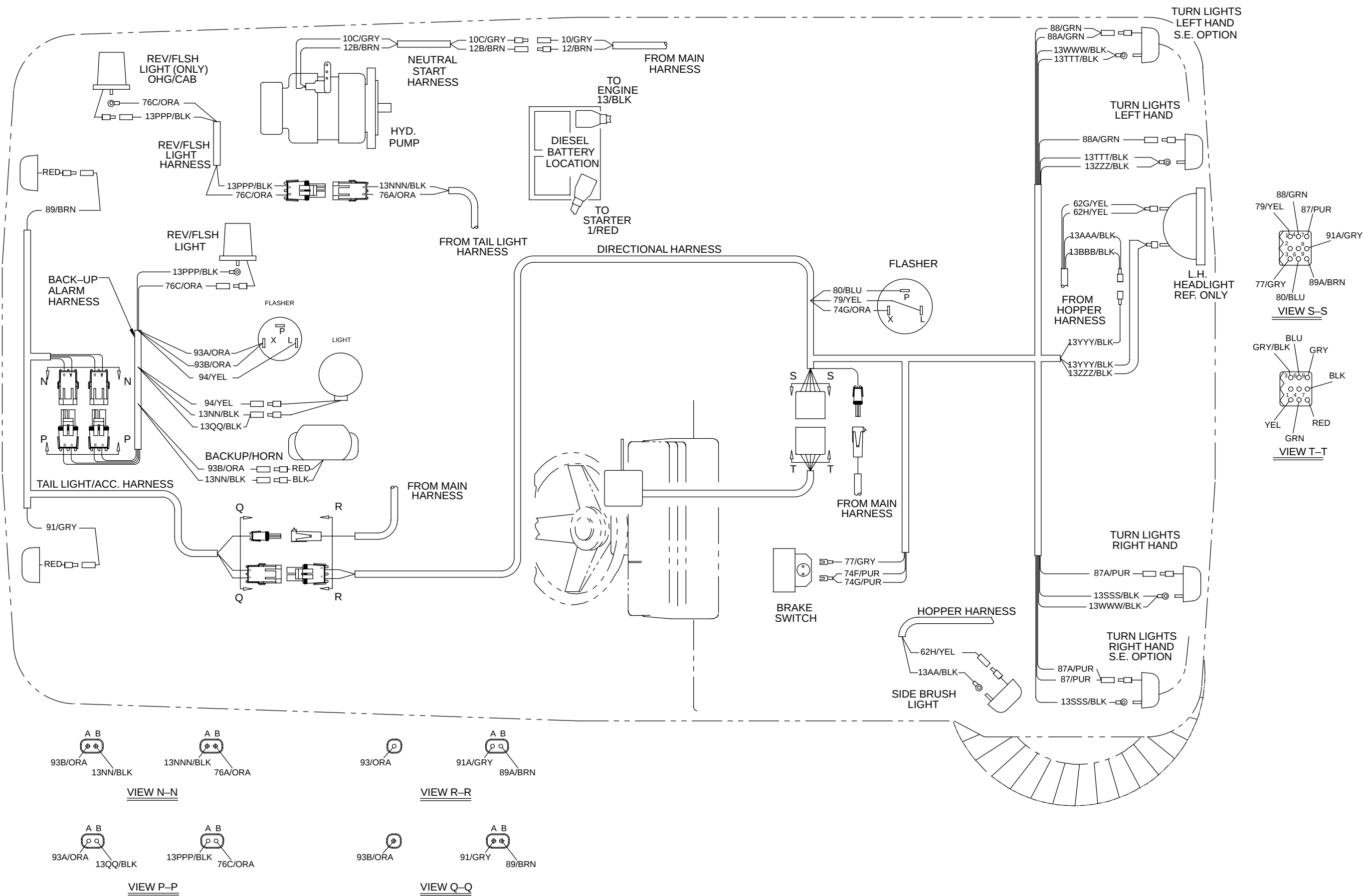
Fig. 71 – Wire Harnesses Group
