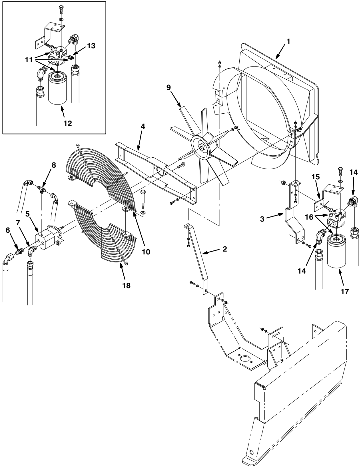
Fig. 40 – Cooling Fan and Housing Group
